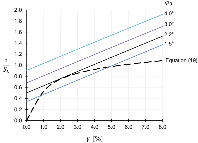
Figure 7. Criterion for matrix failure vs. instability due to shear nonlinearity, where the transition between modes occurs for the \varphi_0 that makes the results from equation (31) tangent to equation (19), after [6].
