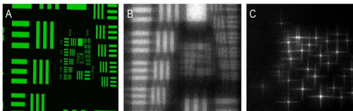
Fig. 5: Resolution test of MapX-II. USAF 1951 imaging standard, Cr on Glass. A) Cr image obtained in a commercial EDAX Orbis PC instrument with a 30 \mu\text{m} polycapillary optic ( \sim 80 \mu\text{m} resolution). B) Raw Cr map measured with the MapX-II instrument. Resolution is decreased as a result of the MPO lens PSF. C) Raw Fe map of 60 \mu\text{m} Fe particles with the MapX-II instrument. The Fe particles that appear as crosses, in which photon intensity is spread away from the source particles in x and y directions.
