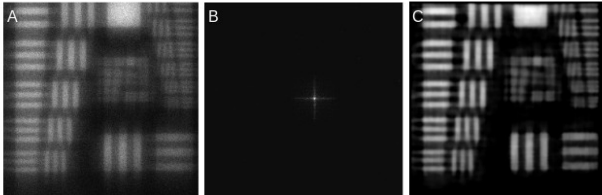
Fig. 7: MapX PSF Deconvolution Example. A) Original image. Chromium K\alpha X-rays (5.4 keV) taken with MapX-II (MPO-CCD = MPO-Target = 50 mm). The resolution of this image is estimated to be 200 \mu\text{m} . B) Point Spread Function measured at the Stanford synchrotron (FWHM \sim 165 \mu\text{m} ). C) AIDA deconvolution with automatized cost function parameters (resolution \sim 135 \mu\text{m} ).
