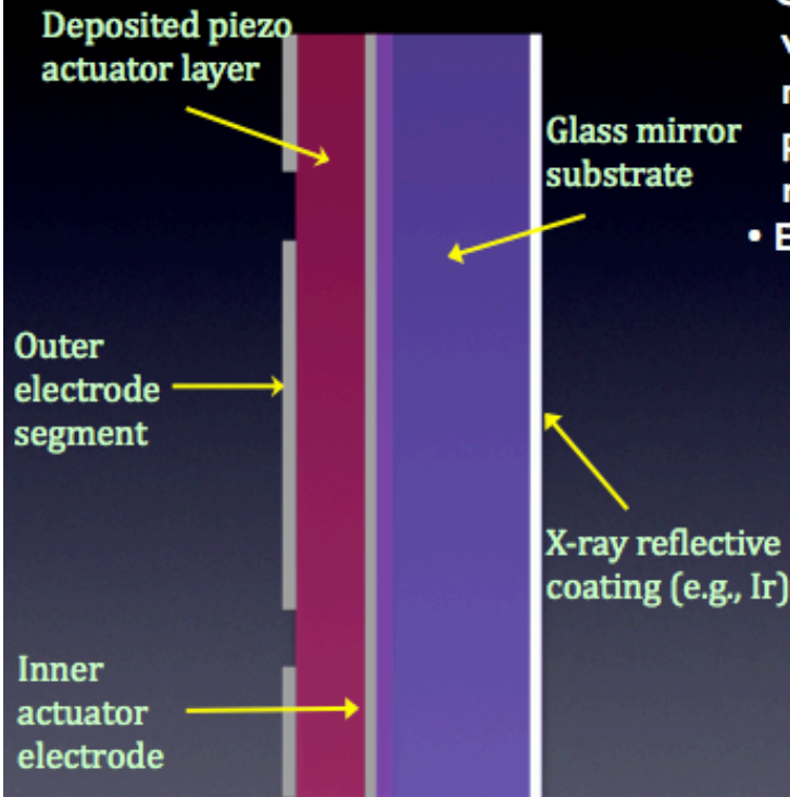
Schematic X-section
