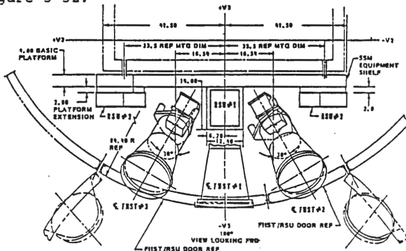
Figure 3-32 Fixed Head Star Tracker Locations on ST
