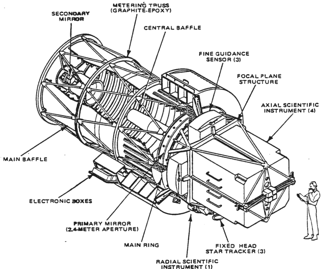
Figure 2-5 Optical Telescope Assembly - Design Features
