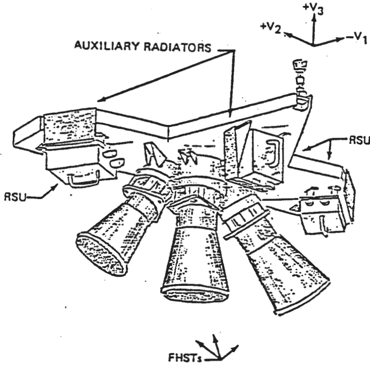
Figure 4-17 SSM-Equipment Shelf
