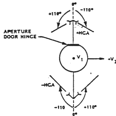
Definition of HGA Y-Axis Angles
