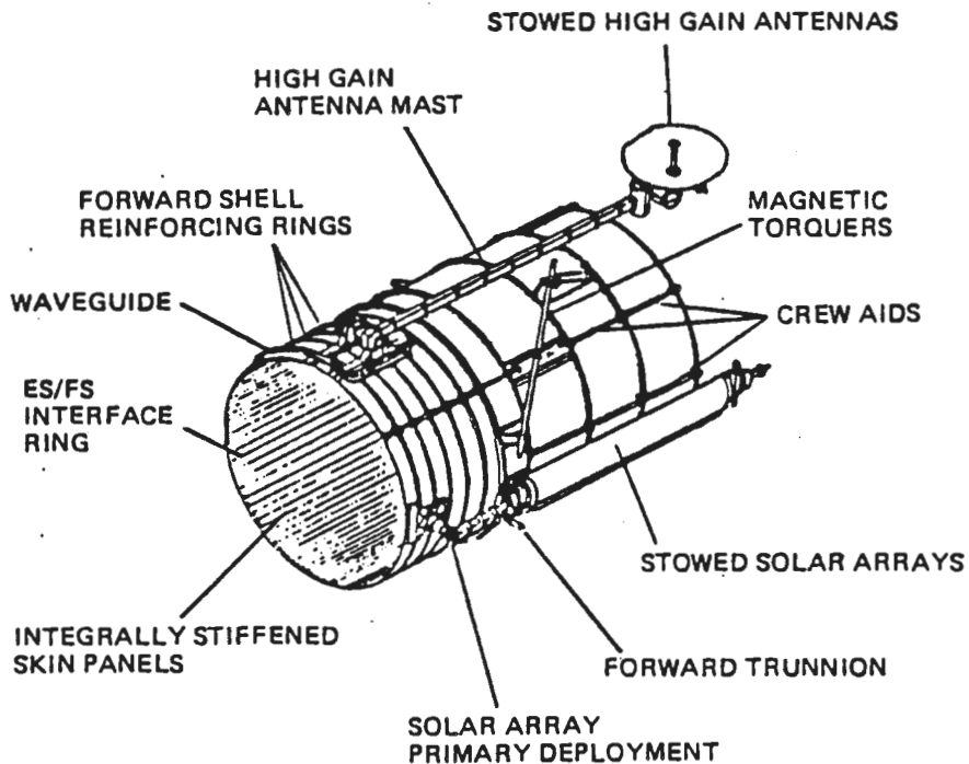
Figure 3-6 Forward Shell
