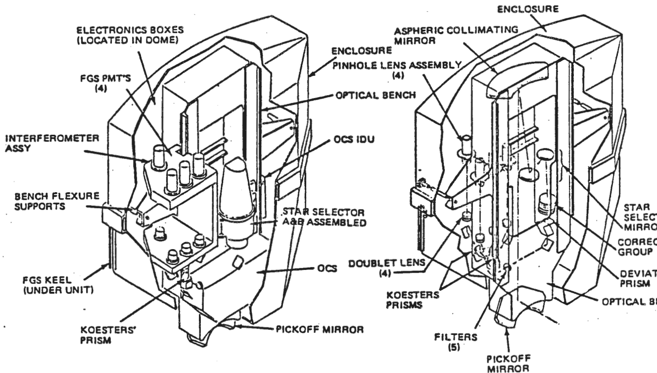
Figure 4-19 FGS Optical and Mechanical Arrangement
