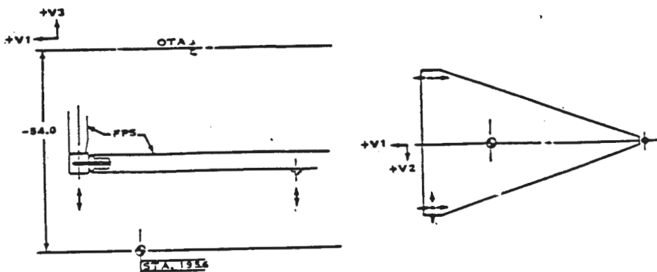
Figure 4-18 SSM-Equipment Shelf Mount Constraints
