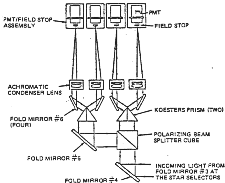
Figure 4-23 Interferometer Optical Assemblies
