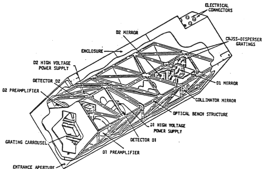
Figure 5-6 High Resolution Spectrograph
