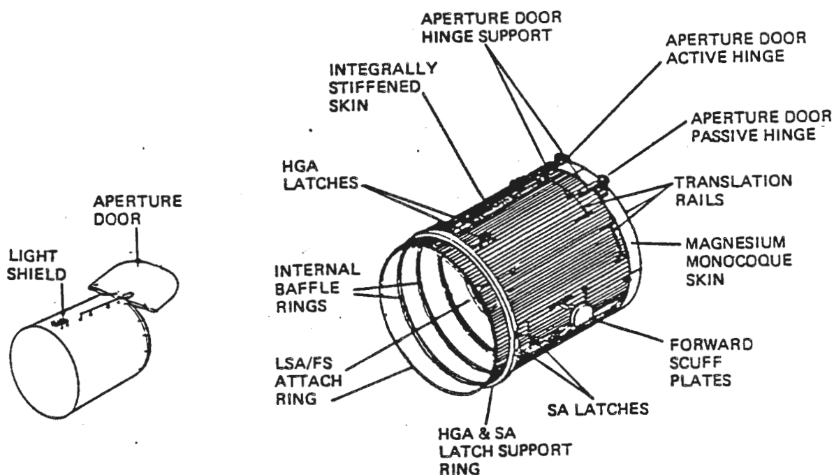
Figure 3-5 Light Shield
