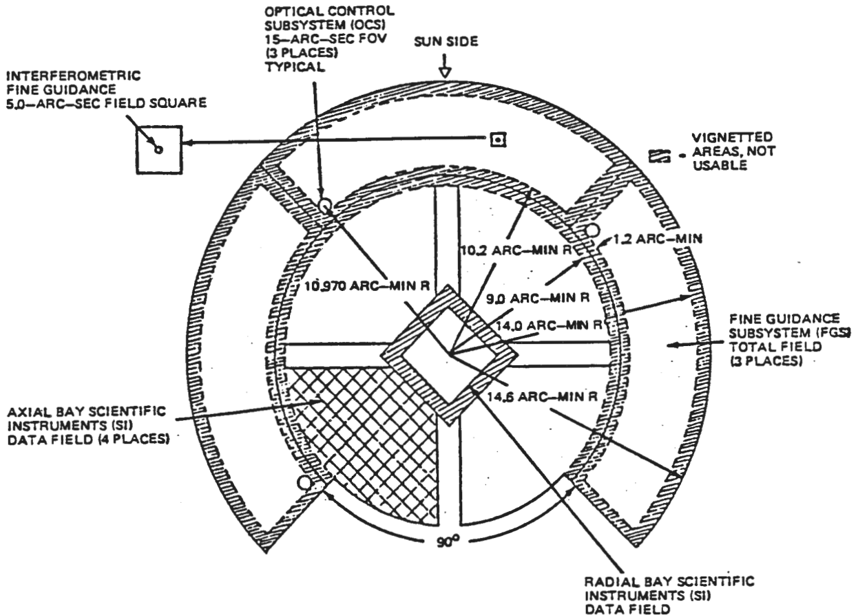
Figure 4-21 Space Telescope Focal Plane
