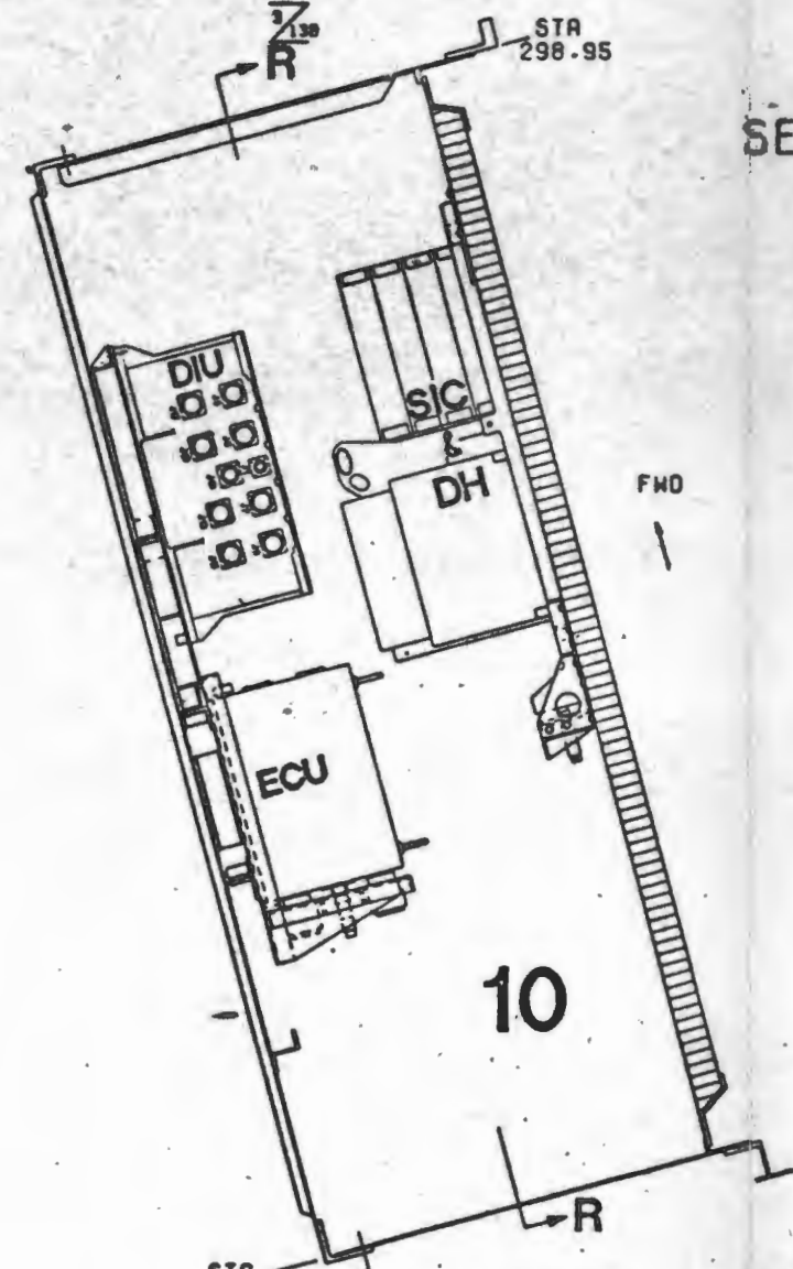
SECTION N-N
