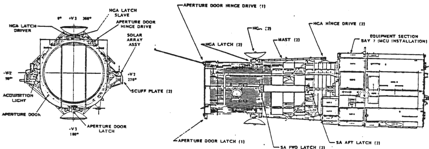
Figure 3-3 Mechanisms Located on ST
