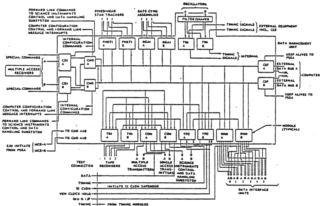
Figure 3-24 DMU Block Diagram
