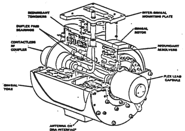
Figure 3-15 Two Axis Gimbal (TAG)
