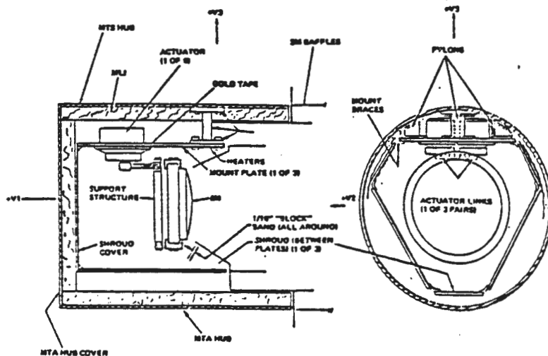
Figure 4-11 Secondary Mirror Subassembly
