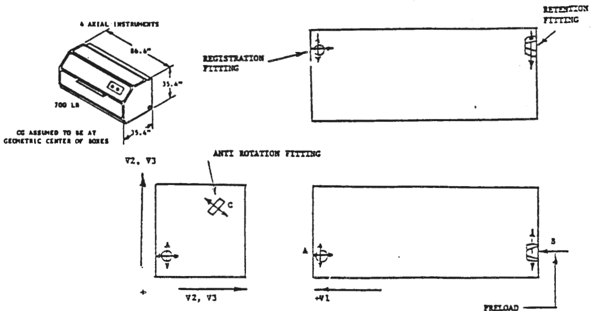
Figure 4-16 Axial SI Mounting Arrangement and Constraints
