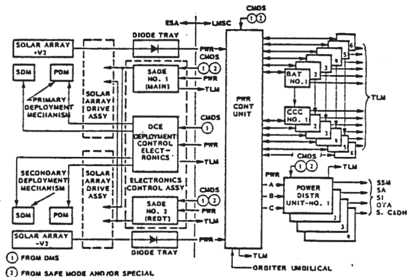
Figure 3-39 Electrical Power Subsystem Block Diagram.
