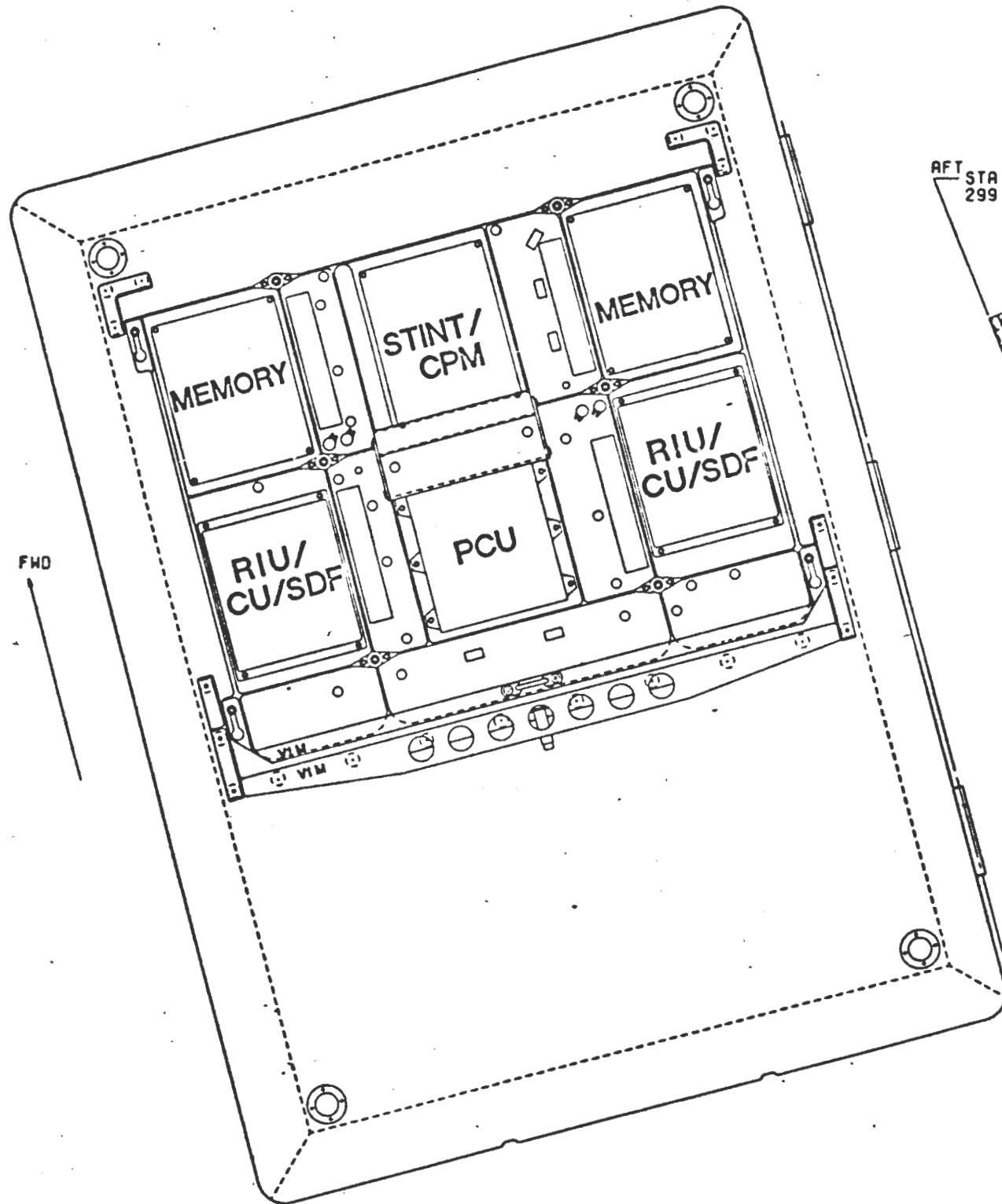
SECTION R-R \nabla VIEW OF BAY 10 DOOR
