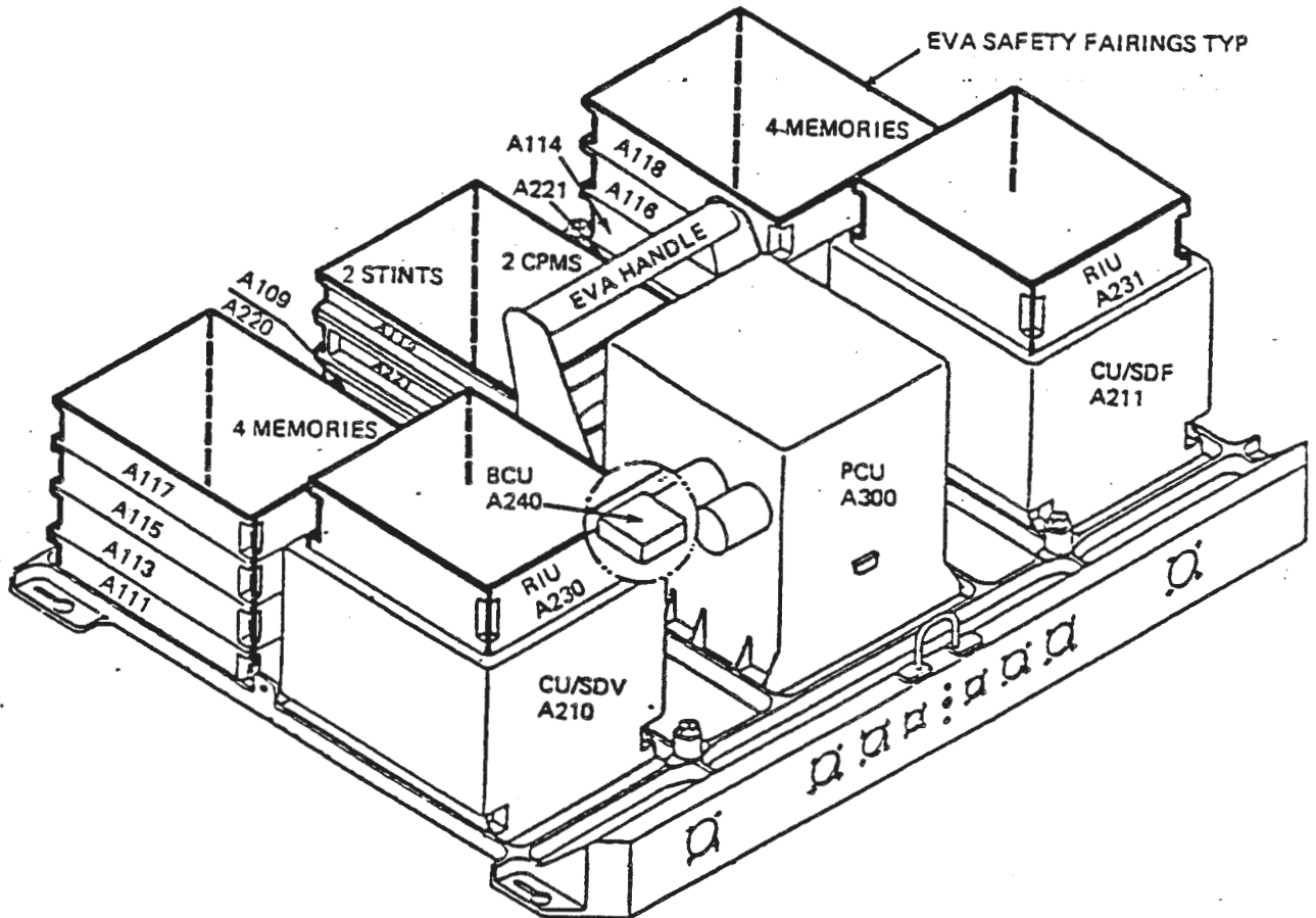
Figure 6-1 SI Control & Data Handling
