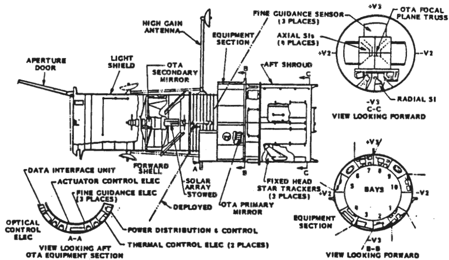
Figure 3-2 ST Inboard/Outboard Profile
