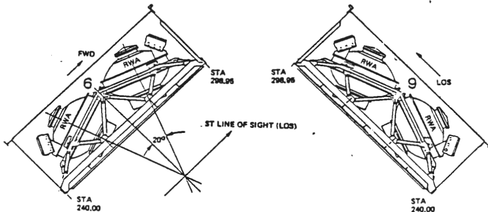
Figure 3-37 RWA Position Detailed View
