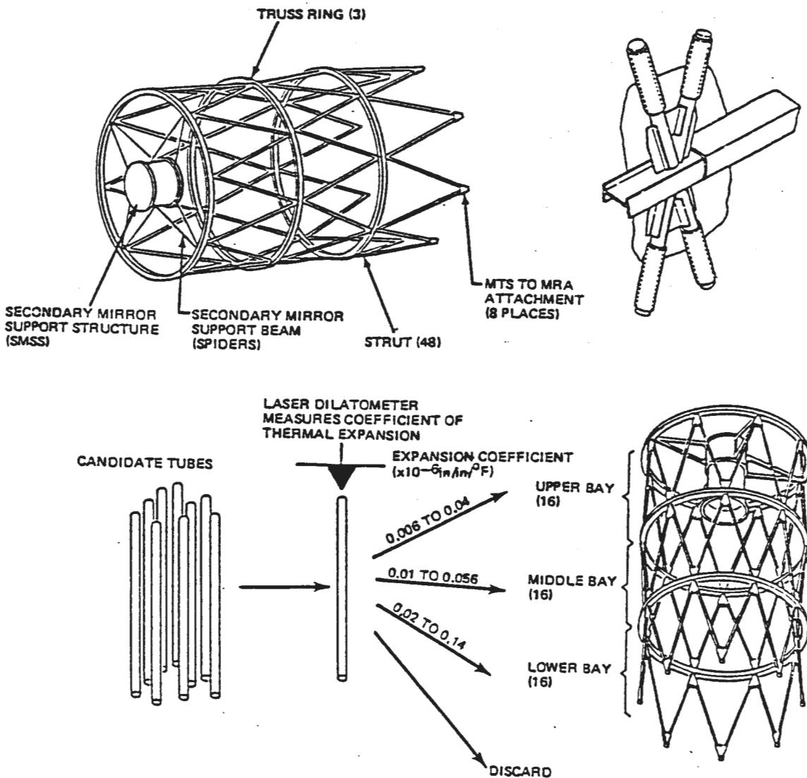
Figure 4-13 Metering Truss
