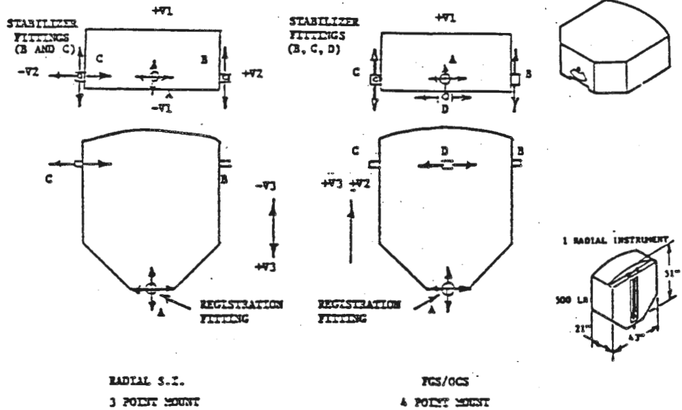
Figure 4-15 Radial Bay Mounting Arrangement and Constraints
