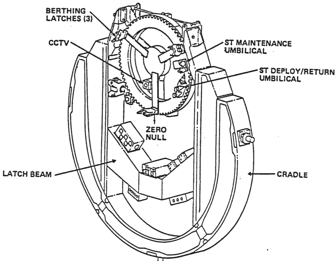
Figure 9-2 SSE Maintenance Platform (Modified FSS)
