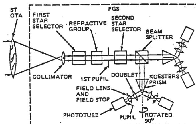
Figure 4-20 Fine Guidance Sensor Optical Schematic
