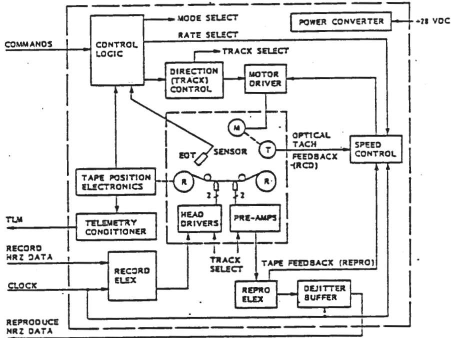
Figure 3-27 Functional Block Diagram of ESTR
