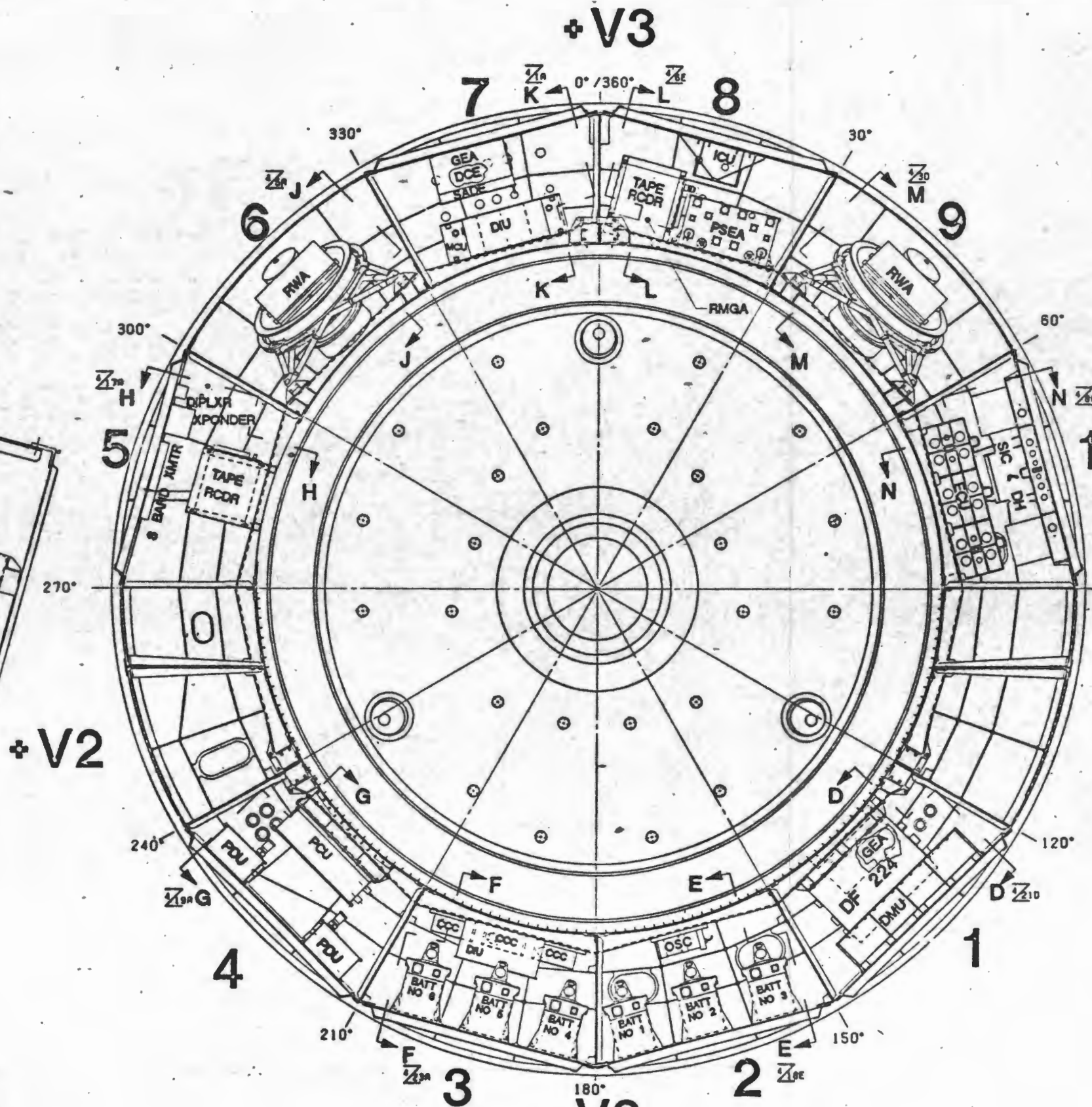
+V3 -V3 SECTION C-C LOOKING FWD
