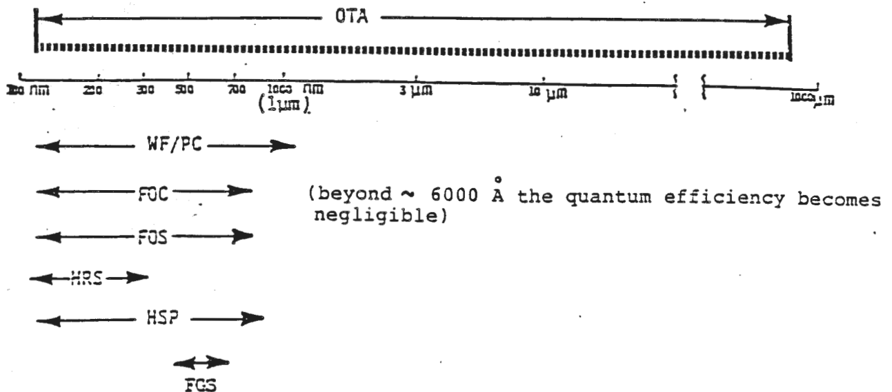
Figure 5-2 Spectral Ranges of the SIs and the OTA
