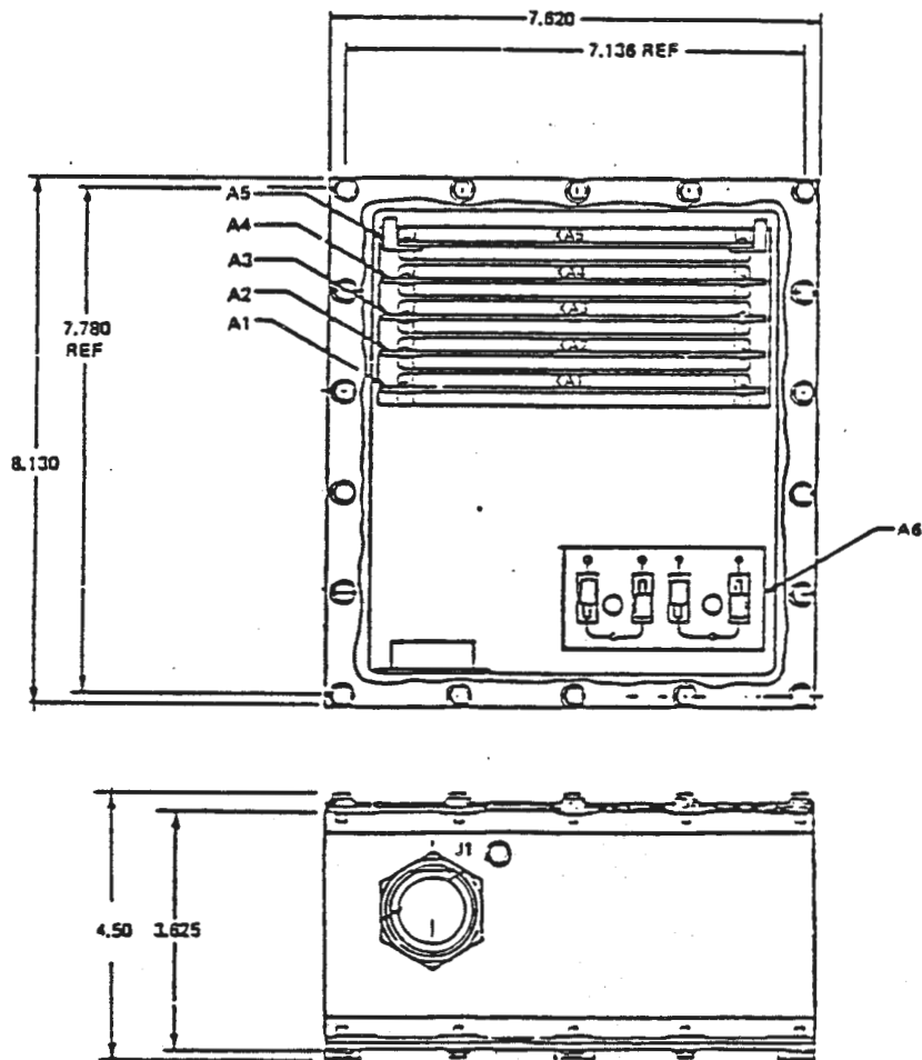
Figure 3-46 Charge Current Controller
