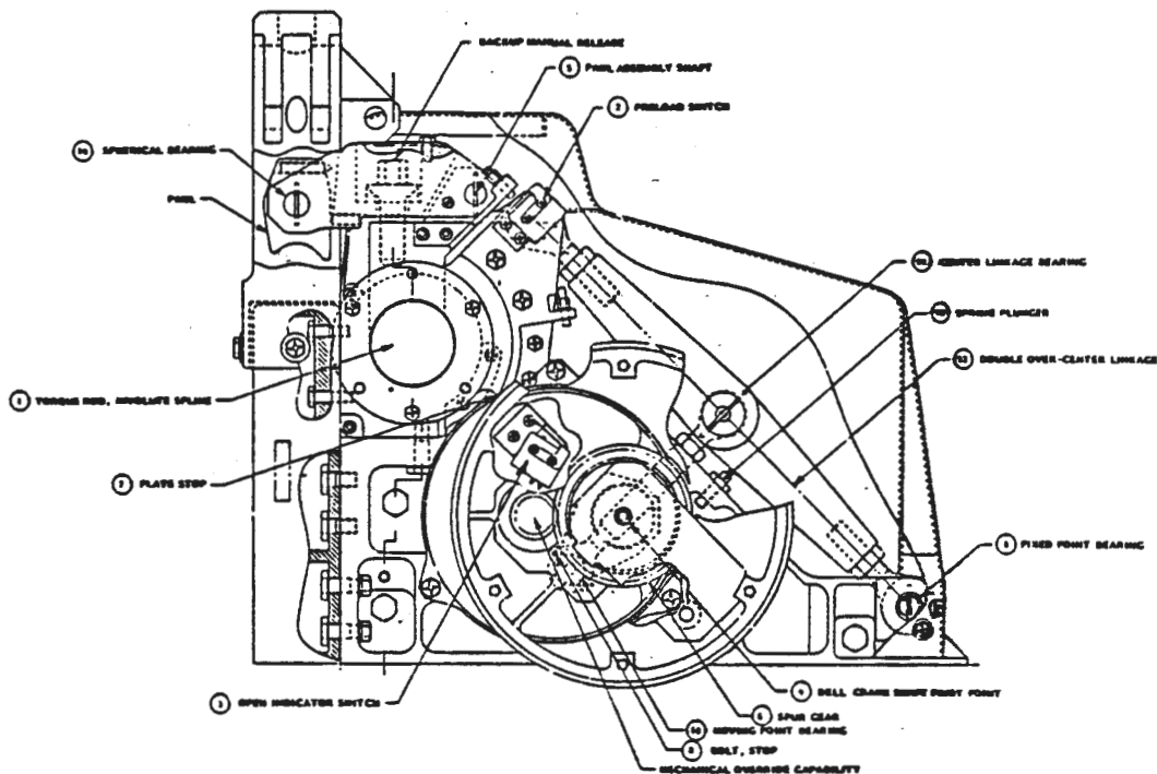
Figure 3-12 Latch Assembly
