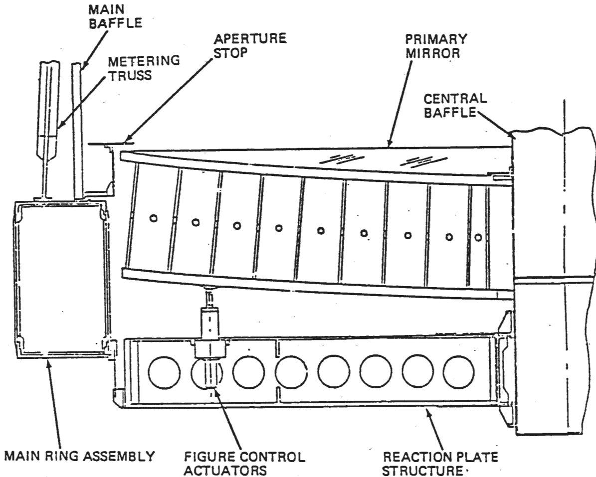
Figure 4-5 Primary Mirror Assembly Cross Section
