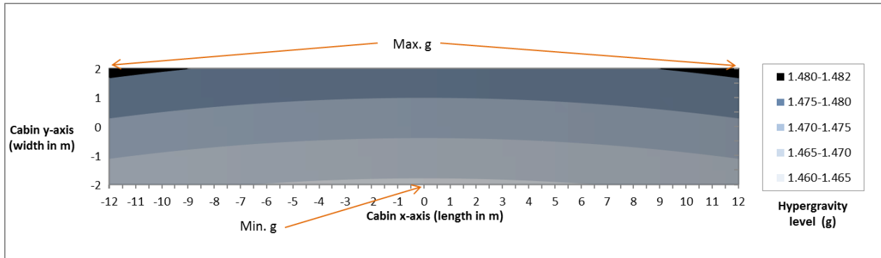
Figure 22. HGVC 24 x 4m Floor Hypergravity Map Example
