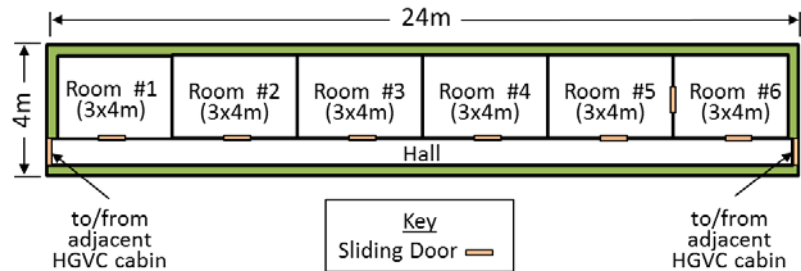
Figure 12. HGVC 6-room Cabin Floor Plan Example (Top View)
