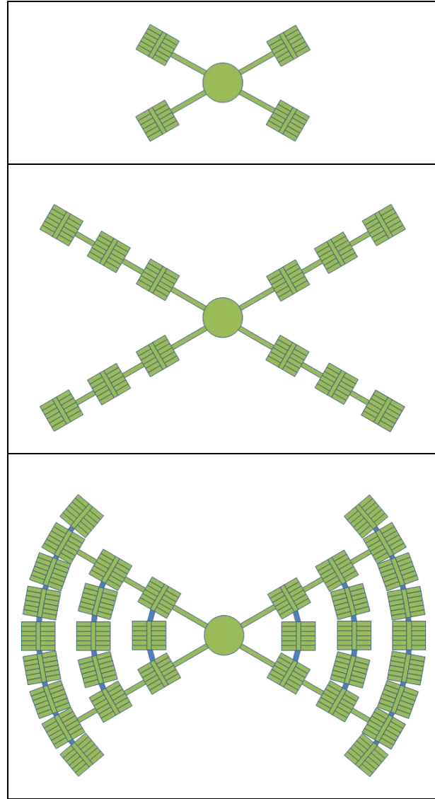
Figure 31. ESHGF Incremental Implementation with 26-Cabin HGVCs in 'X' Configuration Top View Implementations: 4-HGVC (top), 12-HGVC (middle), 34-HGVC (bottom)
