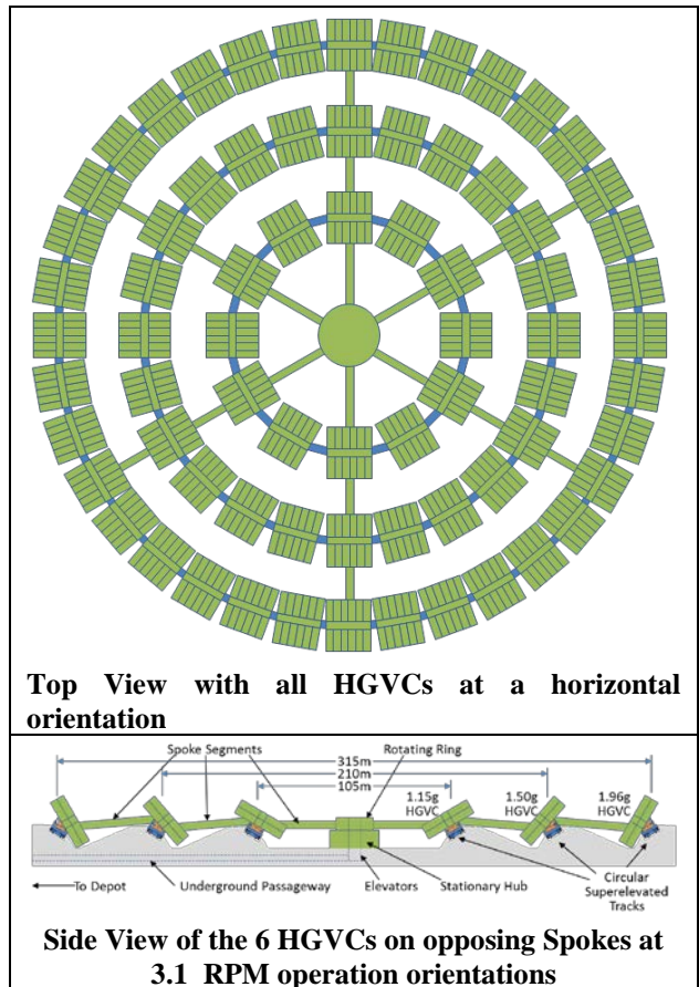
Figure 27. Triple Ring 26-Cabin 72-HGVC ESHGF
