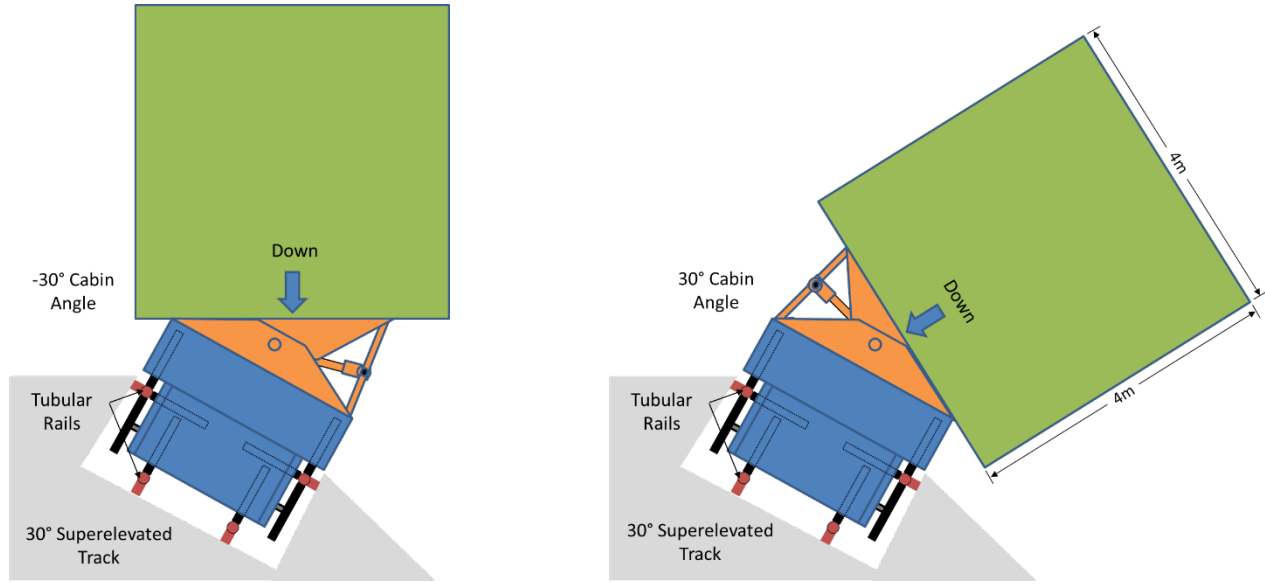
Figure 21. HGVC Car in Stopped Orientation (left) and Max g Orientation (right)
