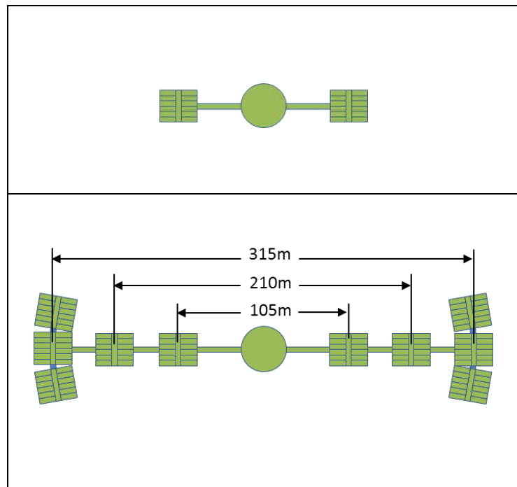
Figure 29. ESHGF Incremental Implementation with 26-Cabin HGVCs
