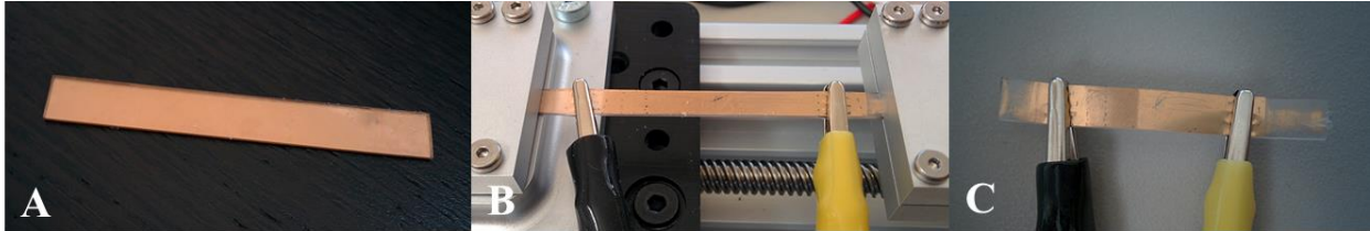
Figure 22. NanoSonic Metal Rubber sensors before, during, and after tensile testing. A) Pristine sensor prior to testing. B) Sample during tensile testing. C) Sample after testing was completed.
