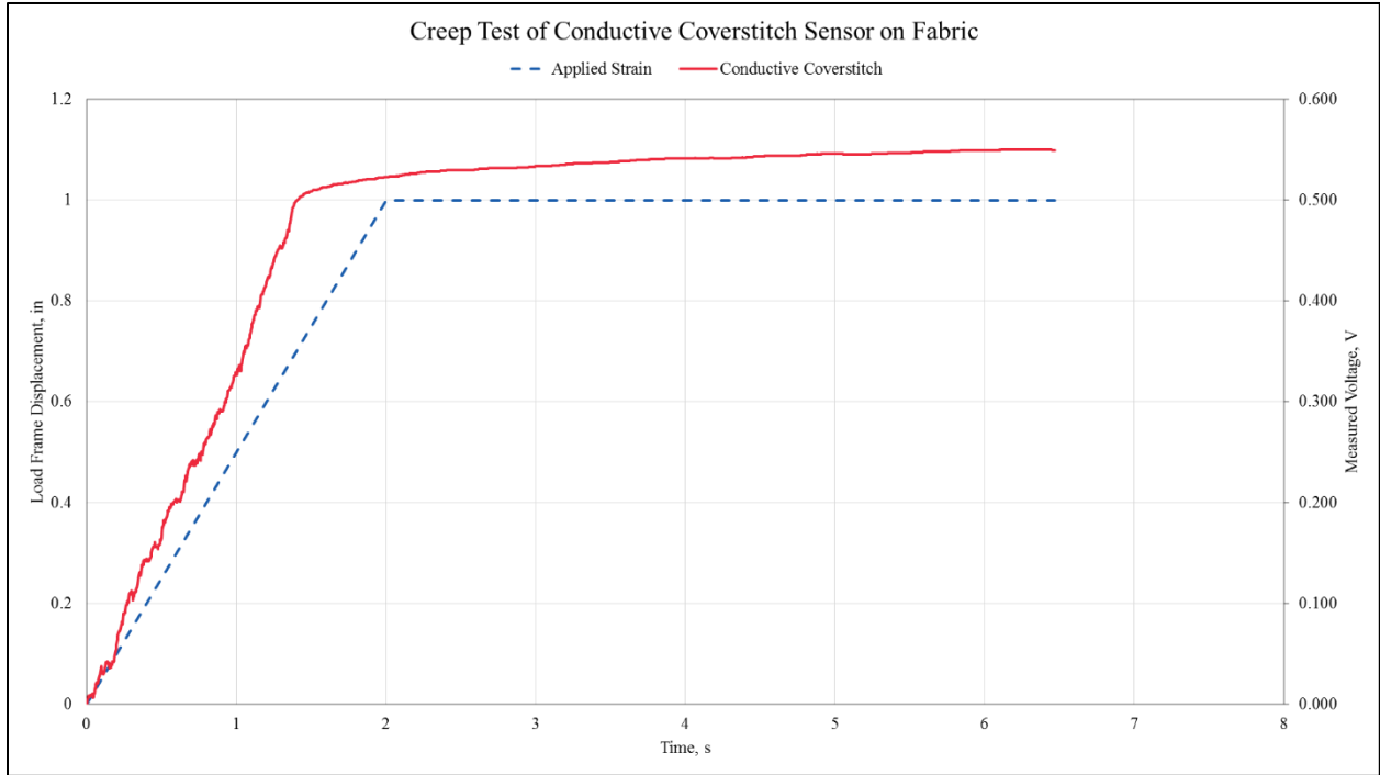
Figure 14. Creep test result of Conductive Coverstitch sensor on fabric.
