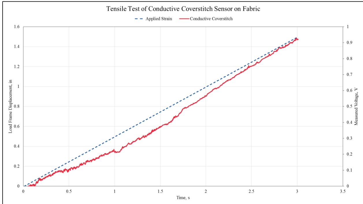
Figure 13. Tensile test result of Conductive Coverstitch sensor on fabric.
