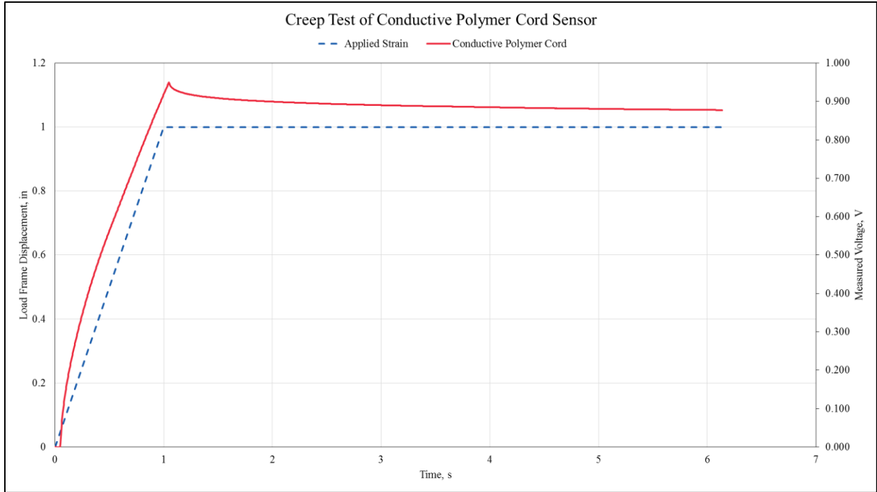
Figure 19. Creep test result of a conductive polymer cord sensor.
