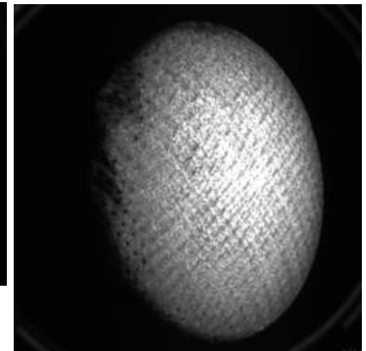
3DQP stagnation arcjet testing
