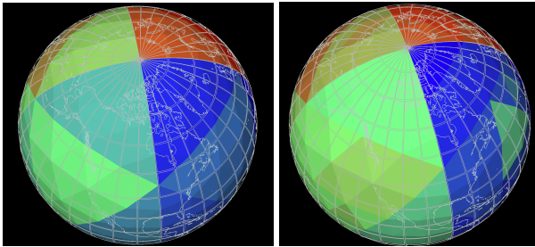
Figure 8. Simple automatic chunking based on HTM integer intervals for different spatial distributions of data/work. Left: homogeneous. Right: non-uniform. Different colors correspond to different partitions and their placement.
