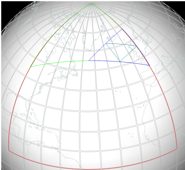
Figure 4. The spherical triangles N0 (red), N01 (green), N012 (purple), N0123 (cyan).
