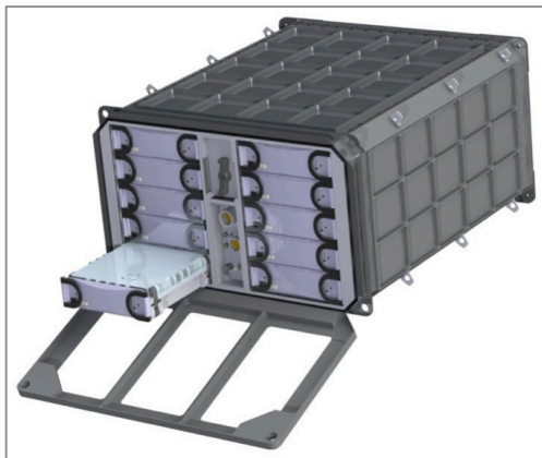
Bioculture System with ten Cassettes and gas supply assembly shown (Image credit: Tissue Genesis, Inc.)
