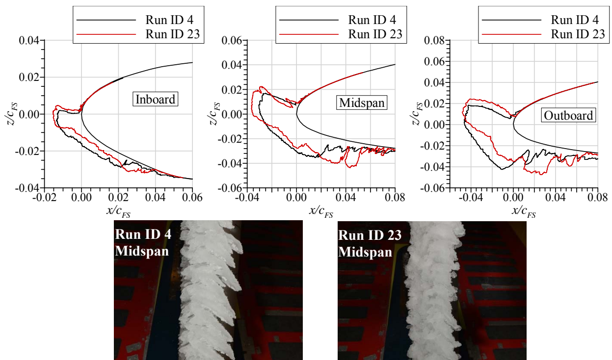
Figure 26. MCCS and photographs of ice accretion on Midspan model showing comparison of maximum scallop condition (Run ID 4) to App. C scaled condition (Run ID 23) (cf. Table 3).
