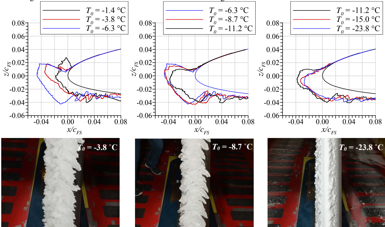
Figure 21. MCCS and photographs of ice accretion on the Outboard model at various total temperatures with other conditions from Table 3 Run ID’s 2, 3, 4, 5, 6, 7 and 8.
