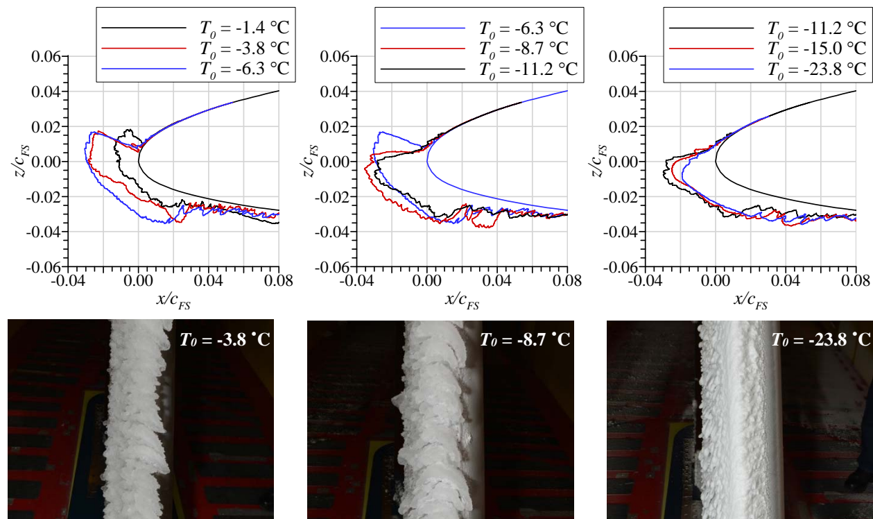
Figure 20. MCCS and photographs of ice accretion on the Midspan model at various total temperatures with other conditions from Table 3 Run ID’s 2, 3, 4, 5, 6, 7 and 8.
