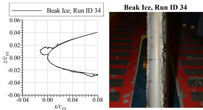
Figure 29. Outboard model MCCS and photograph for beak ice case; Run ID 34.
