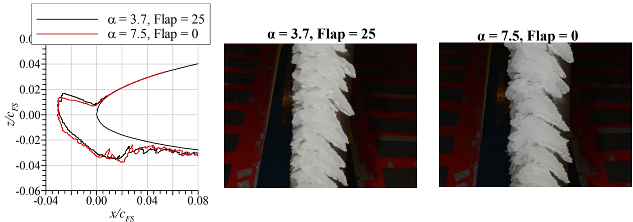
Figure 25. Midspan model MCCS and photographs of ice accretion comparison of maximum scallop condition with attachment point matched at two different angles of attack; \alpha=3.7 deg., Flap = 25 Run ID 4 and \alpha=7.5 deg. Flap = 0 deg. Run ID 31 at identical icing conditions.
