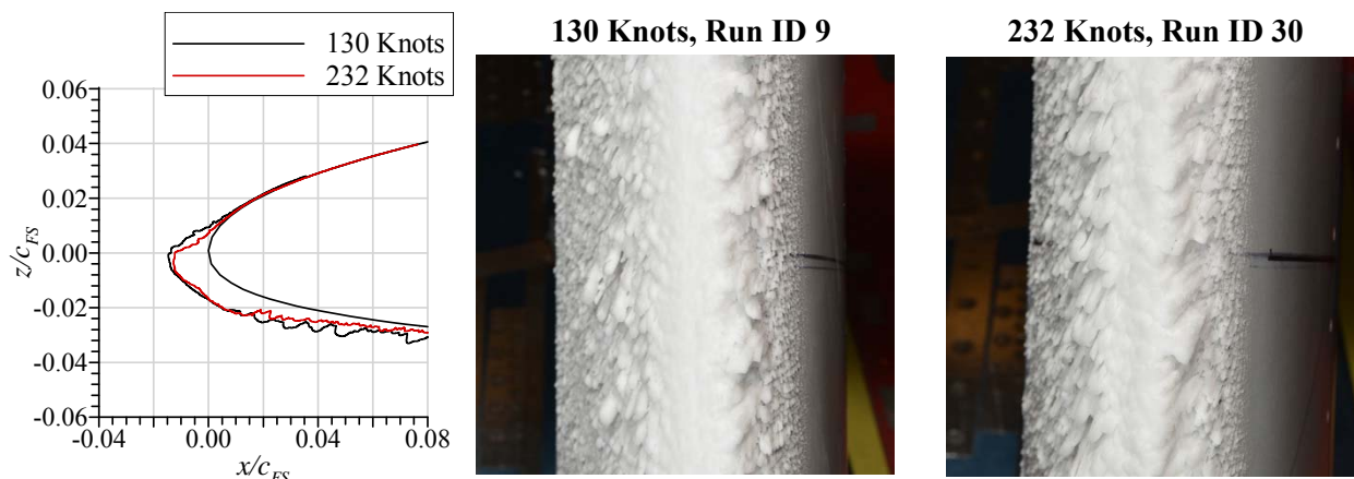
Figure 28. Outboard model MCCS and photographs of ice accretion showing effect of airspeed on scaled ice accretion; 130 knots Run ID 9 and 232 knots Run ID 30.
