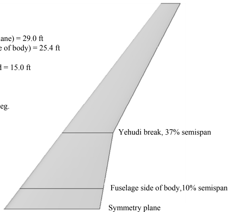
Figure 1. Summary of CRM65 wing geometric characteristics, adapted from Broeren et al. 1 and Vassberg et al. 29
