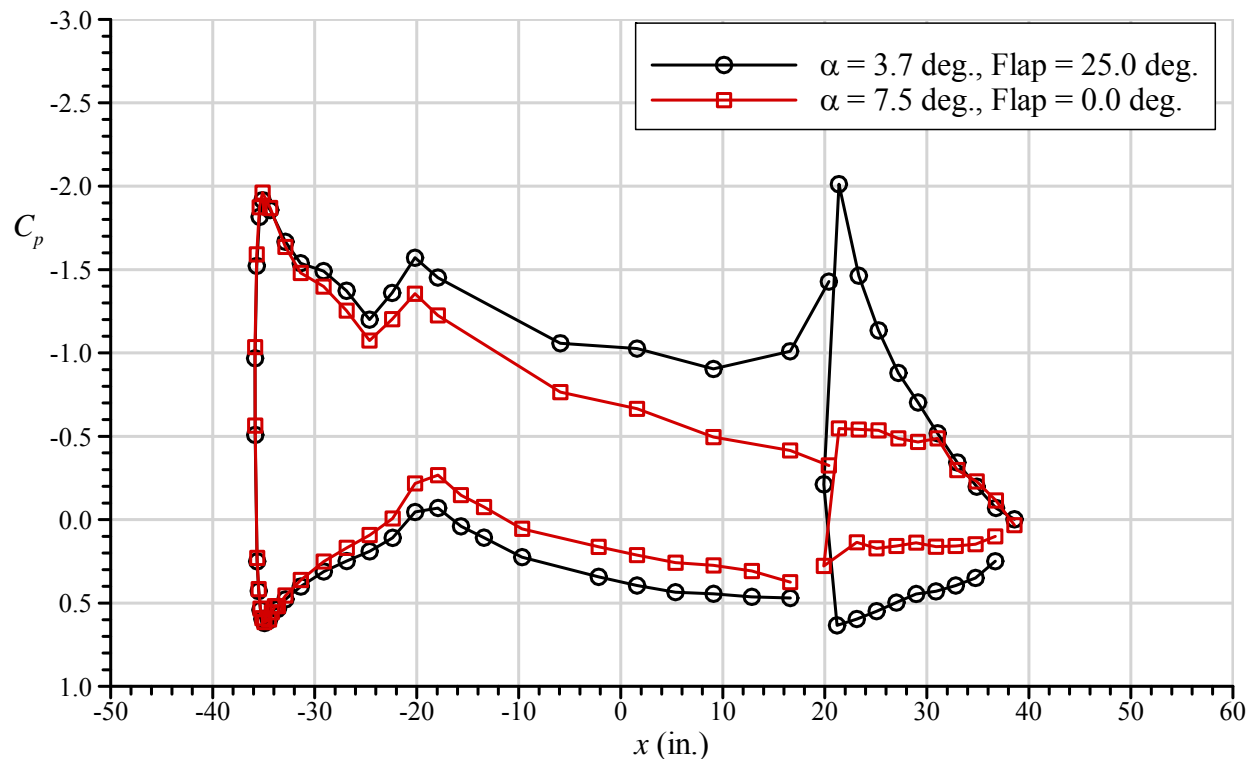
Figure 24. Midspan model pressure distribution for alternative incidence and flap angles. Data were acquired at 130 knots and total temperature = -9.2 °C.
