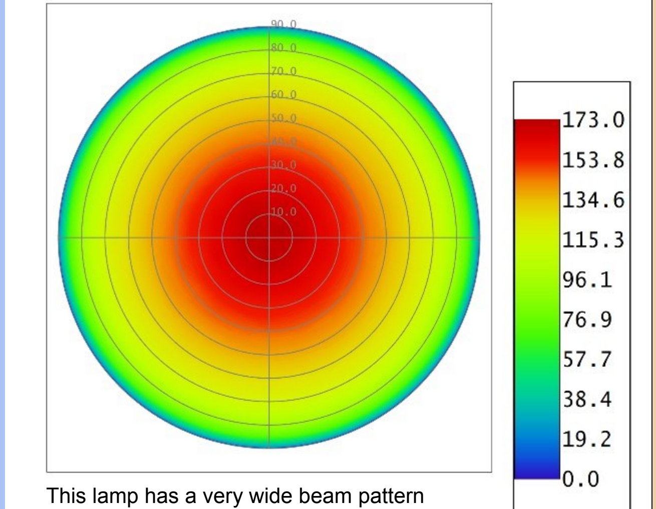
Isocandela Beam Pattern Plot for Mockup Facility Ambient Light System Lamps.
