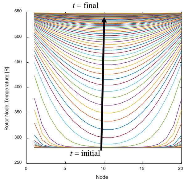
Figure 7. Rotor internal temperature transient.
