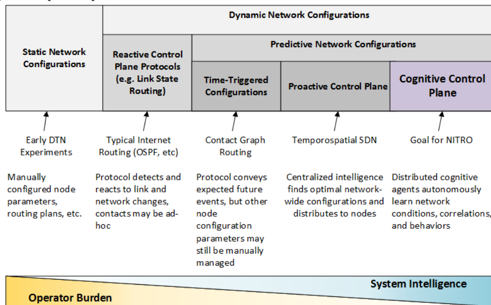
Figure 2. Progression of routing technology towards cognitive control plane capabilities
