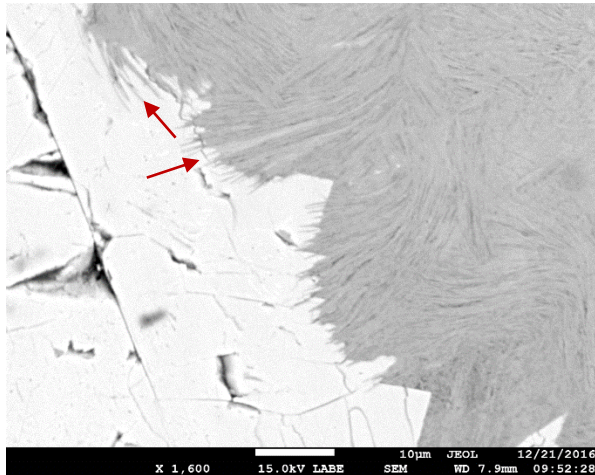
Fig. 3. BSEI: Transformation of the Ca-, Fe-silicate to a wispy, fine-grained silicates. The transformation seems to be oriented in two distinct directions (red arrows).
