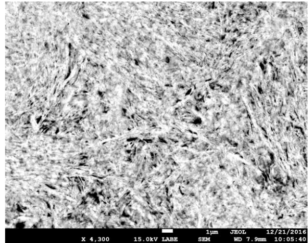
Fig. 5 BSE closeup of olivine pseudomorphs after phyllosilicates in the vein shown (arrowed) in Fig. 1.
