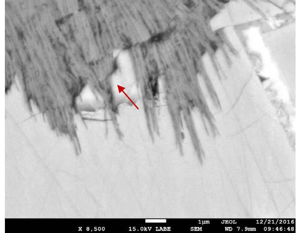
Fig. 4. BSEI: Close-up of the boundary between the serrated edge of the Ca-, Fe-silicate and wispy silicate. Note the conjoined boundary between the two minerals at the tip of the red arrow.
