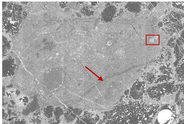
Fig. 1. BSEI of a dark inclusion in the Leoville thin section USNM 3535-1. The clast is ~6 mm across. The red rectangle marks the area of Fig. 2.
