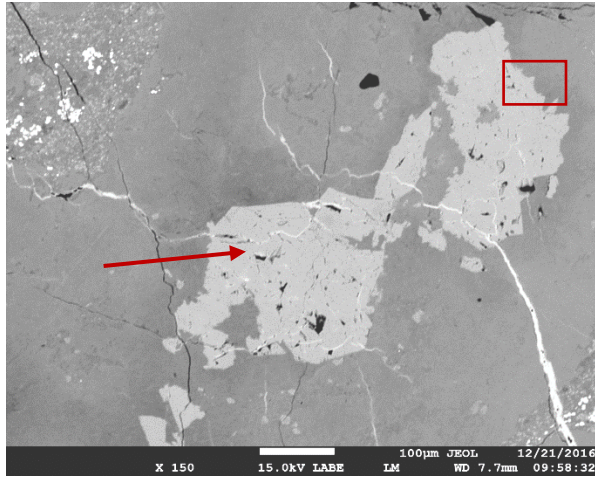
Fig. 2. BSEI: Euhedral to subhedral Ca, Fe-silicate grains (red arrow) in the dark inclusion seen in Fig. 1. The red rectangle marks the area seen in Fig. 3.
