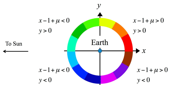
Figure 8: Color scheme used in the mapping strategy, indicating the angular location of the final apoogee relative to the Sun- L_2 line.
