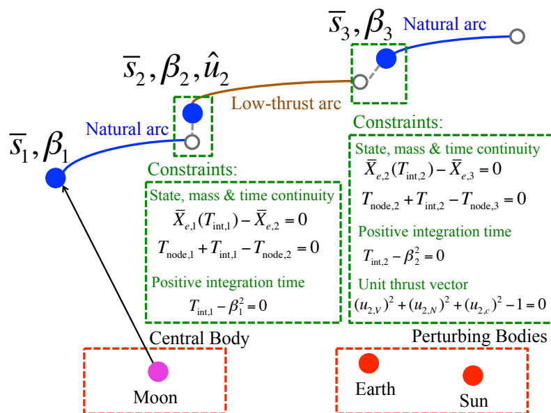
Figure 2: Illustration of variable time multiple shooting formulation to target a continuous trajectory for a low-thrust-enabled spacecraft in an ephemeris model.
