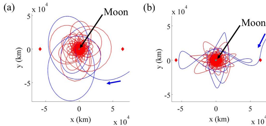
Figure 17: Sample science orbit approach trajectories with (a) low Jacobi constant value and long time of flight, and (b) high Jacobi constant value and short time of flight.
