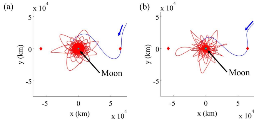
Figure 18: Recovery of lunar approach paths from the L2 gateway map at (a) an epoch of 28433 MJD and (b) two days later at an epoch of 28435 MJD. Trajectories appear in an Earth-Moon rotating frame with blue arcs indicating natural motion and red arcs indicating low-thrust-enabled motion.
