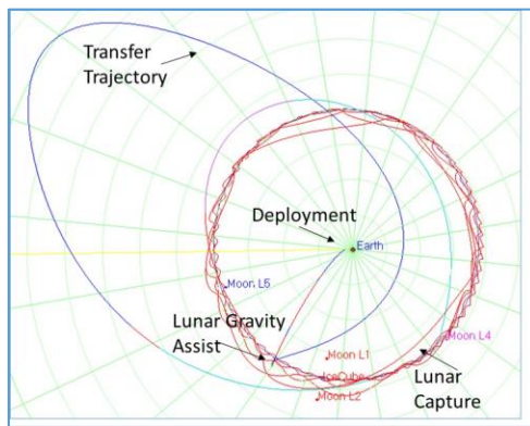
Figure 3. Lunar IceCube Trajectory Transfer
