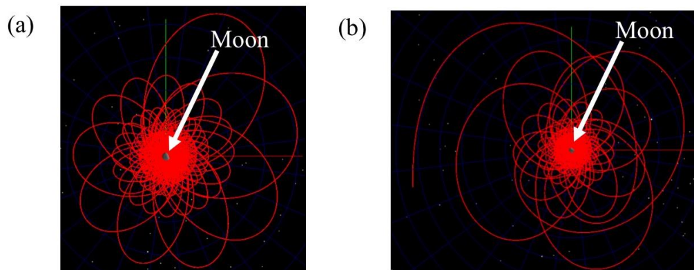
Figure 10 (a) Low-thrust-enabled trajectory of a spacecraft integrated backwards in time for nearly six months from an initial condition located at TA=40 degrees along a feasible science orbit with a RAAN equal to 160 degrees at an epoch of 28610 MJD, and (b) similar trajectory for a RAAN equal to 180 degrees.
