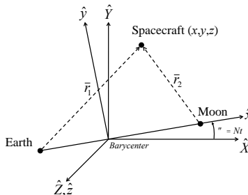
Figure 2. System configuration for a spacecraft within the Earth-Moon CR3BP.
