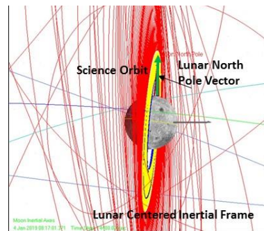
Figure 22. Transfer to Science Orbit Showing Polar Orbit
