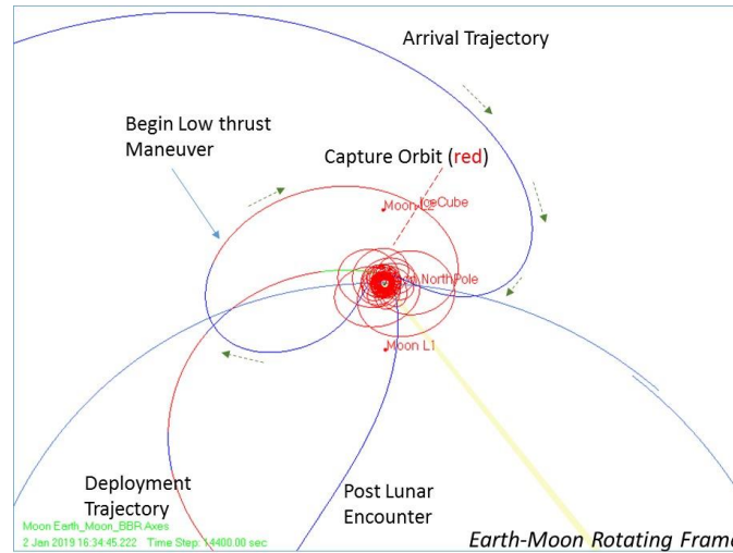
Figure 24. Sample point solution that reaches a 45 degree inclination lunar orbit, viewed in Earth-Moon rotating frame.
