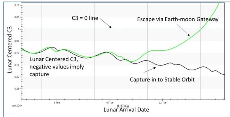
Figure 7. Comparison of the lunar C3 for two trajectories, a reference path (black) and perturbed solution (green), that differ in the start of the low-thrust maneuver by two days.
