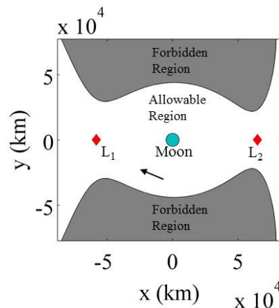
Figure 11. Earth-Moon gateways and zero velocity curves separating forbidden and allowable regions of motion for a given Jacobi constant.
