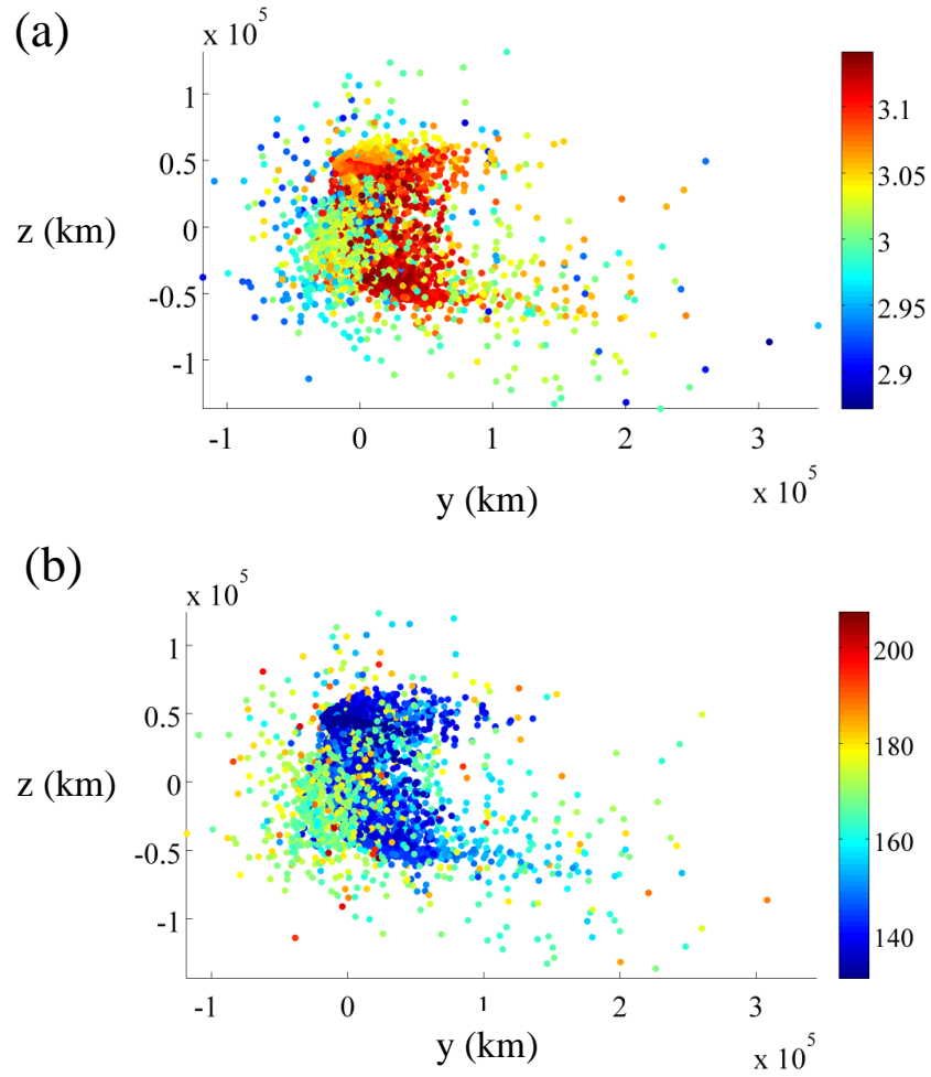
Figure 16: L_2 gateway map depicting the crossings of trajectories that arrive at the lunar science orbit in forward time with the assistance of a low-thrust engine at epochs between 28610 MJD and 28630 MJD, colored by (a) the Jacobi constant in the Earth-Moon CR3BP and (b) the time of flight to the crossing of the hyperplane.
