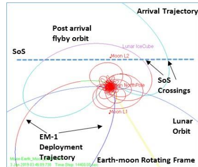
Figure 20. Lunar IceCube Transfer Trajectory
