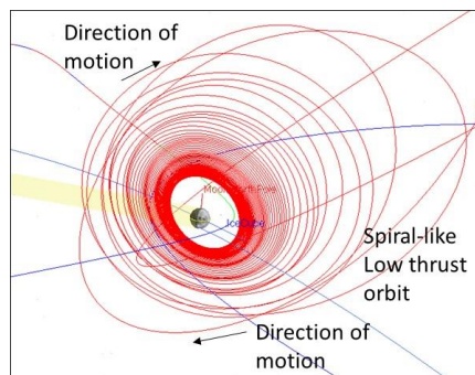
Figure 5. Lunar Capture with Low Thrust
