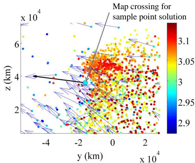
Figure 25. Comparison of L2 gateway map, colored by Jacobi constant measured in the Earth-Moon system, and a sample point solution that reaches a 45 degree inclination lunar orbit. Vectors indicated y- and z- velocity components.
