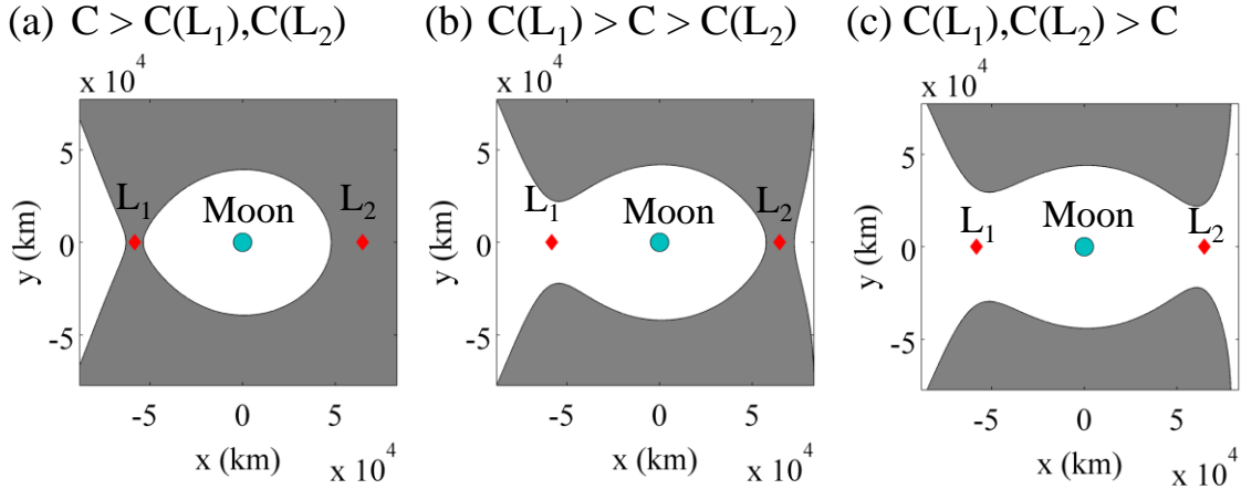
Figure 12: Evolution of the zero velocity curves and opening of the L_2 gateway as the Jacobi constant is decreased.
