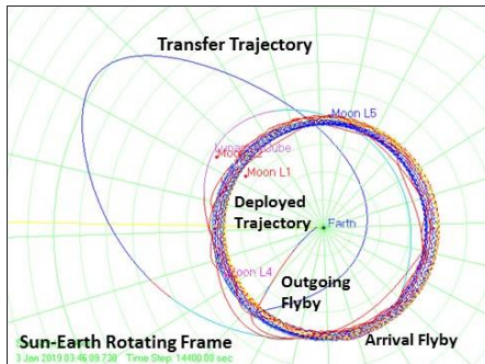
Figure 19. Lunar IceCube Transfer Trajectory
