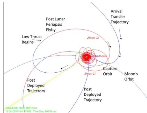
Figure 4. Arrival Trajectory in Earth-Moon Rotating Coordinates
