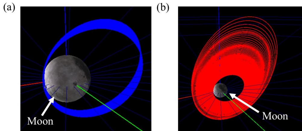
Figure 9 (a) The natural motion of a spacecraft backwards in time for 88 days from an initial condition located at periaapsis along a feasible science orbit with a RAAN equal to 0 degrees at an epoch of 28610 MJD, and (b) low-thrust-enabled motion for 90 days backwards in time from the same initial condition.
