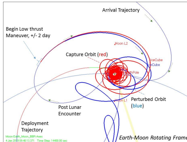
Figure 8. Sensitivity of arrival energy on a capture trajectory
