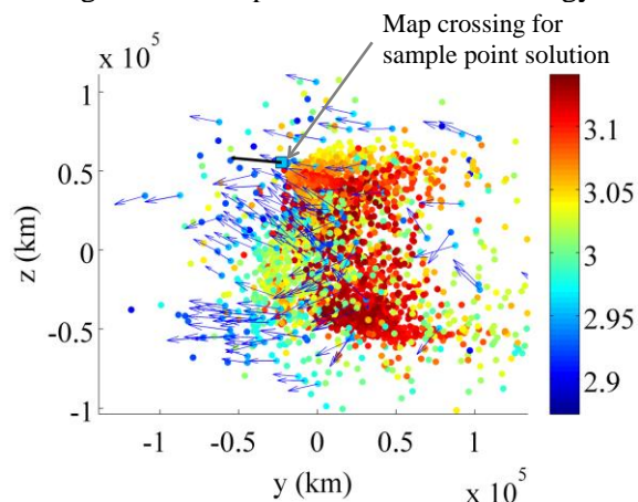
Figure 23. Comparison of L2 gateway map, colored by Jacobi constant measured in the Earth-Moon system, and a sample point solution that reaches a 93 degree inclination lunar orbit. Vectors indicated y- and z- velocity components.
