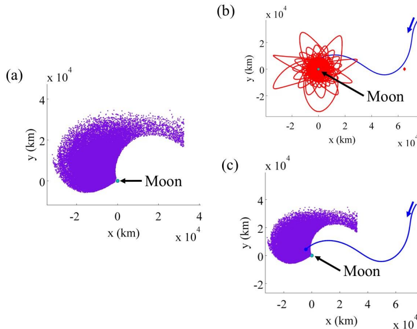
Figure 14: Demonstration of natural manifold structures enabling flow towards the lunar vicinity through (a) the first periapses of the unstable manifolds of the L_2 periodic and quasi-periodic orbits, (b) a sample science orbit approach trajectory where the low-thrust engine is activated at the first perilune, and (c) the location of this perilune overlaid on the unstable manifold periapses.
