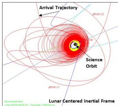
Figure 21. Transfer to Science Orbit-Side view
