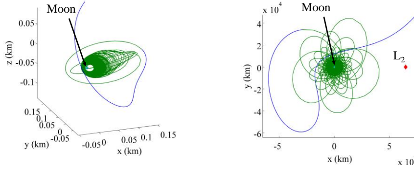
Figure 13: Sample arc that captures into the desired lunar science orbit, displayed in (a) a Moon-centered inertial J2000 equatorial frame, and (b) a Moon-centered Earth-Moon rotating frame. Green arcs indicate that the thruster is activated in the anti-velocity direction, while blue arcs correspond to natural motion
