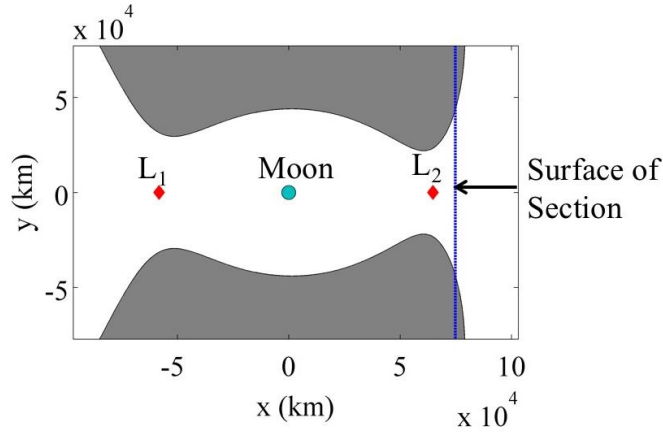
Figure 15: Definition of the surface of section used to construct an L_2 gateway map
