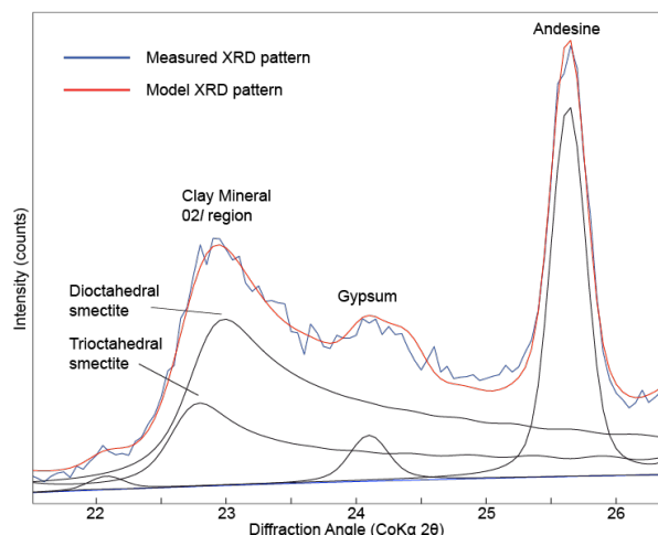
Figure 1 – Rietveld refinement of Marimba XRD pattern showing modeled contributions from dioctahedral and trioctahedral clay mineral phases to 02l region of the pattern.
