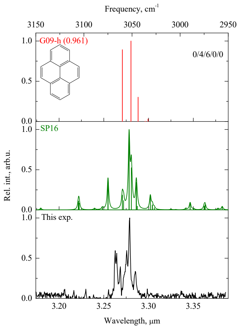
Fig. 2.— The IR absorption spectrum of pyrene as predicted by G09-h and SP16 calculations together with the molecular beam gas-phase spectrum as measured in the present experiments.
