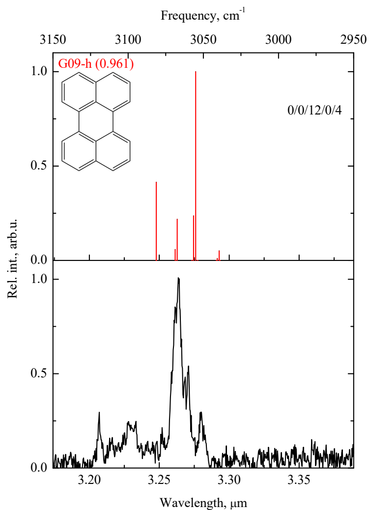
Fig. 6.— The IR absorption spectrum of perylene as predicted by G09-h calculations together with the molecular beam gas-phase spectrum as measured in the present experiments. Calculations at the SP16 level lead to incorrect results (see text) and therefore are not reported.
