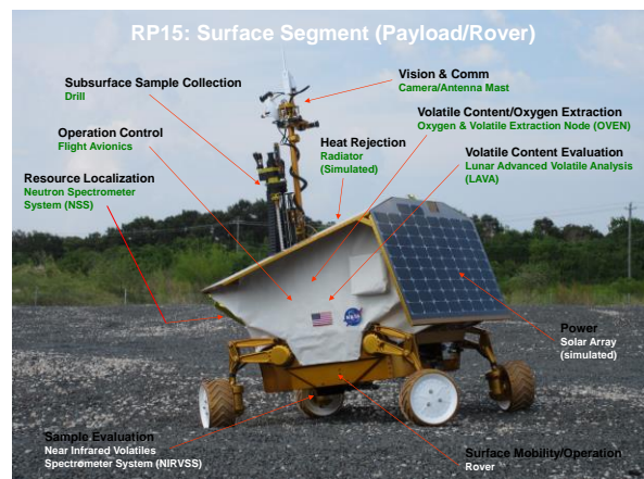
Figure 1. The RP15 rover and payload propotype was designed, built, and operated remotely with distributed operations network.
