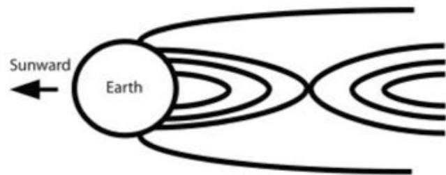
1. Magnetotail Substorm
