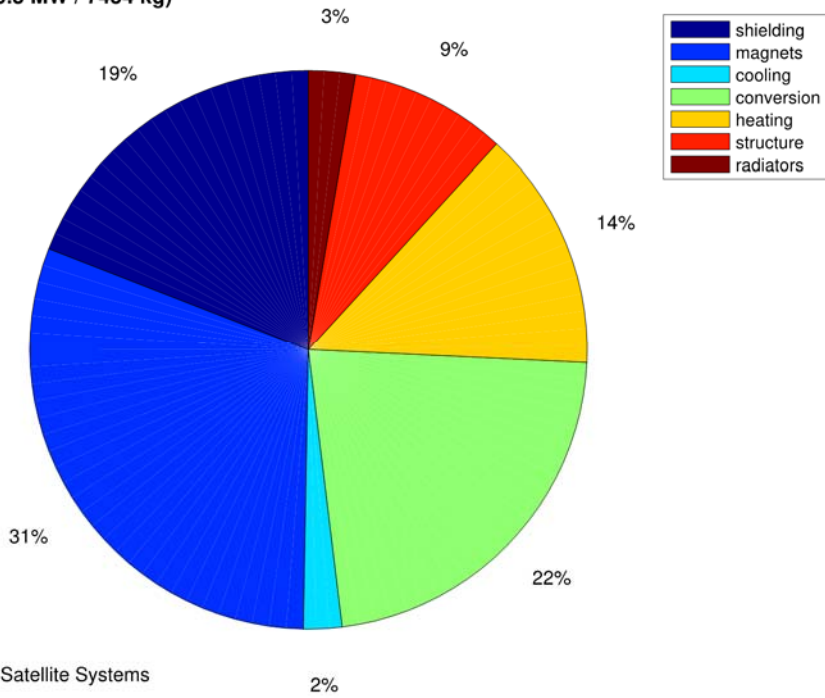
Princeton Satellite Systems Figure 37. Engine Mass Pie Chart for 10 MW Engine.
