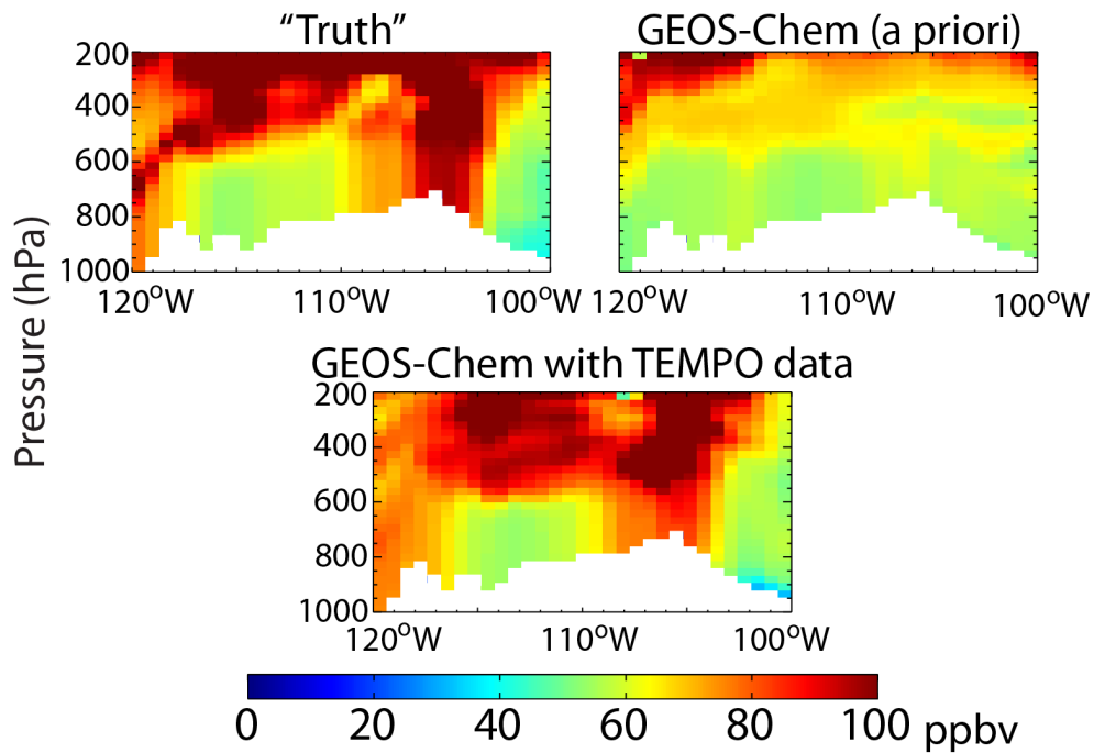
Figure 9. Longitude-altitude cross-section of ozone concentrations ( 36^{\circ}\text{N} , 3 GMT on June 14, 2010) associated with a stratospheric intrusion. The “true” state from an independent chemical transport model (top left) is compared to the GEOS-Chem model without data assimilation (top right) and with assimilation of TEMPO data (bottom). Local topography is shown in white. Modified from Zoogman et al. [2014].
