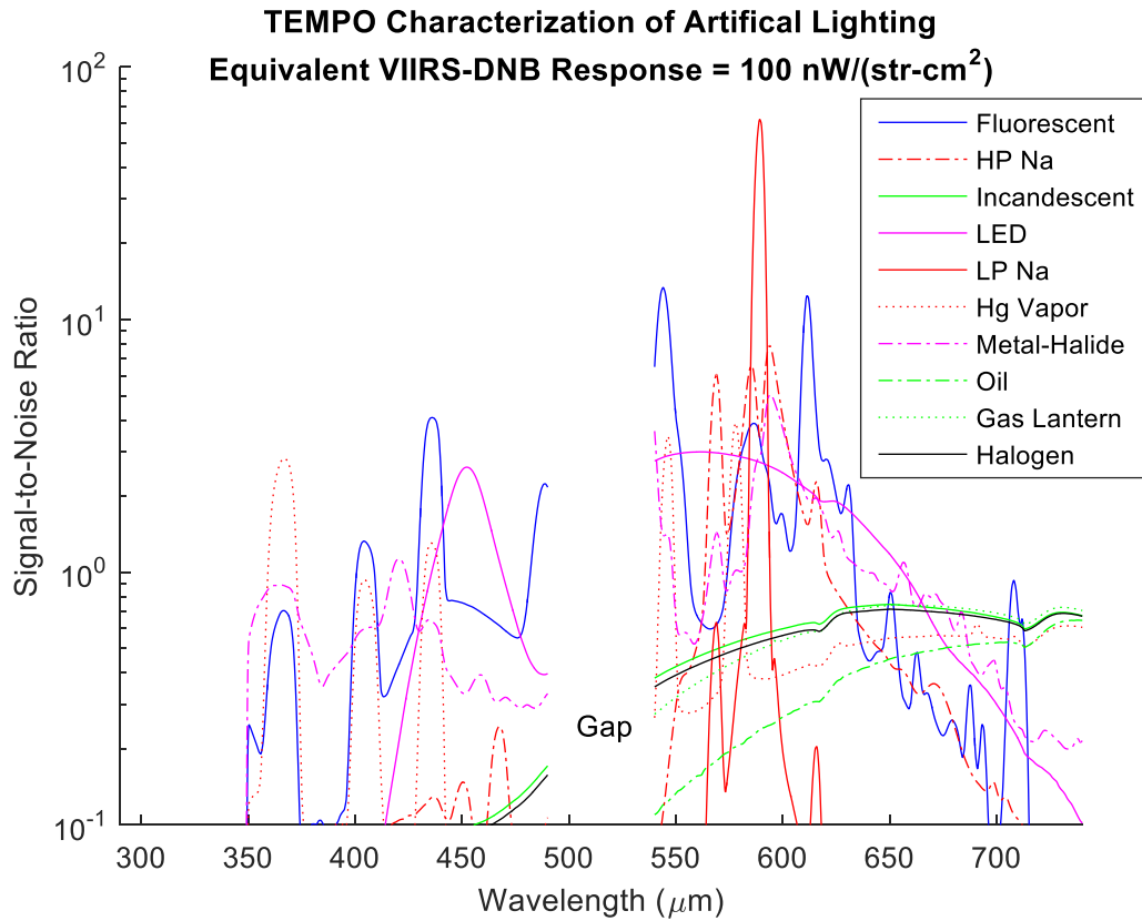
Figure 10. SNRs of various artificial lighting types normalized to a common VIIRS-DNB response with a 10s dwell, no co-addition, and no spatial binning, assuming a dark current of 2800 \text{ e}^- \text{ s}^{-1} . City lights over all of greater North America can either be observed piecemeal over several days or in a single scan near the winter solstice.
