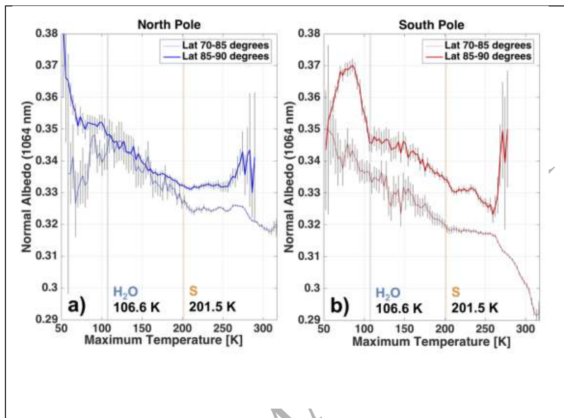
Figure 5. Average 1064 nm reflectance as a function of maximum temperature (maximum temperature bin width=3K) for low slope (slope <math>< 10^\circ</math>) areas free of mass wasting influence for areas within 5 degrees of each pole, and between 5 and 20 degrees from each pole., illustrating spatial heterogeneity in polar reflectance-temperature relationships. a) North polar data; b) South polar data. Curves plotted with 2\sigma standard error of the mean. Volatility thresholds for elemental sulfur and water ice are included for comparison. Thresholds were derived by Zhang and Paige [2010] a sublimation rate of 1mm/Gyr.
