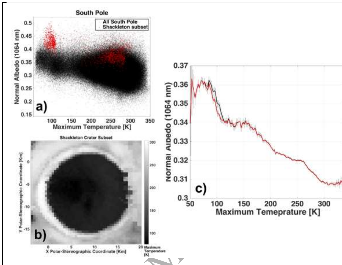
Figure 7. a) Scatter plot of South polar reflectance vs. maximum temperature, with points in red derived from a small subset chosen to isolate South-polar Shackleton crater. Region included as red points are shown in (b) . c) Curves comparing average 1064 nm reflectance as a function of maximum temperature for the south polar dataset within 20 degrees of the pole (black), and the same data with the \sim 25 \times 25 km Shackleton subset shown in (b) removed (red). Maximum temperature bin width=2K. Curves are plotted with 2\sigma standard error of the mean. Exclusion of Shackleton shifts, but does not eliminate, the sharp uptick in reflectance below 110K. [2 column]
