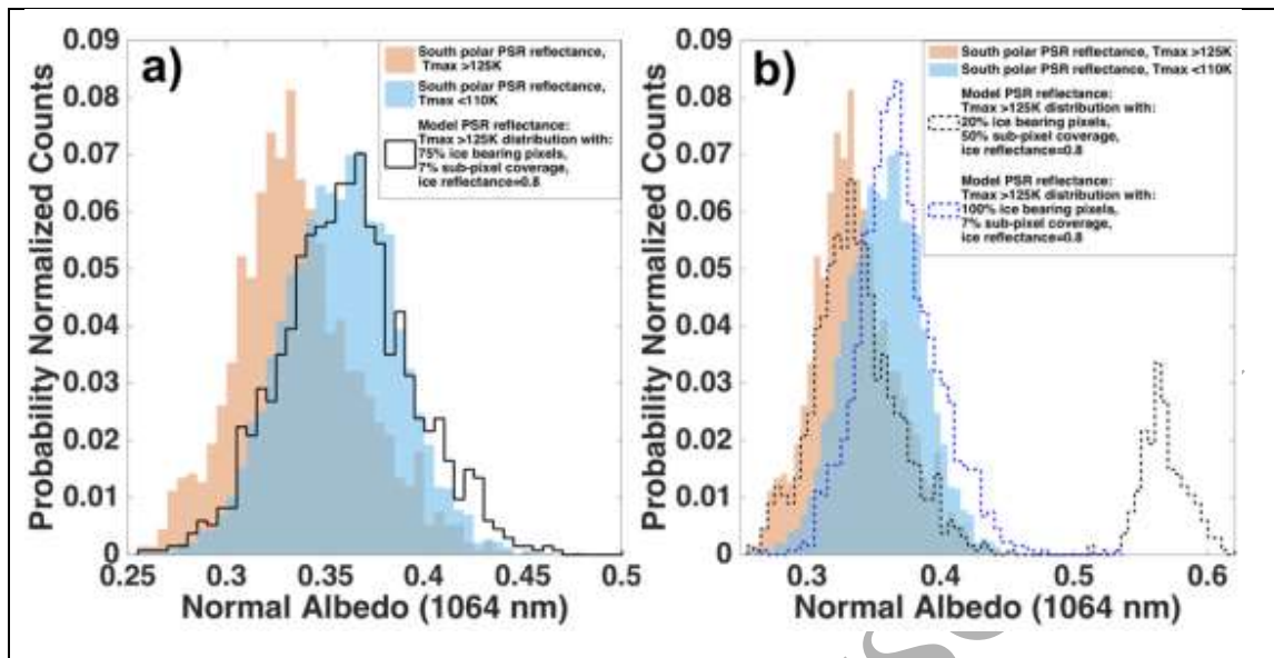
Figure 10. Results of some combinations of ice-modeling parameters consistent with plausible modes of ice preservation, compared to the real reflectance distributions of low slope (slope < 10^\circ ) South-polar PSRs (average incident flux=0%), with maximum temperatures low enough ( < 110K ) to preserve surface ice (filled blue), and high enough ( > 125K ) to preclude the preservation of surface ice (filled orange). Reflectance bin width=0.005. a) results of adding sub-pixel scale, heterogeneously distributed icy material to the reflectance distribution of ice-free south polar PSRs (black solid line). b) results of adding sub-pixel scale, homogeneously distributed icy material (black dashed line), and supra-pixel scale heterogeneously distributed icy material (blue dashed line) to the reflectance distribution of ice-free south polar PSRs. [1.5 column]
