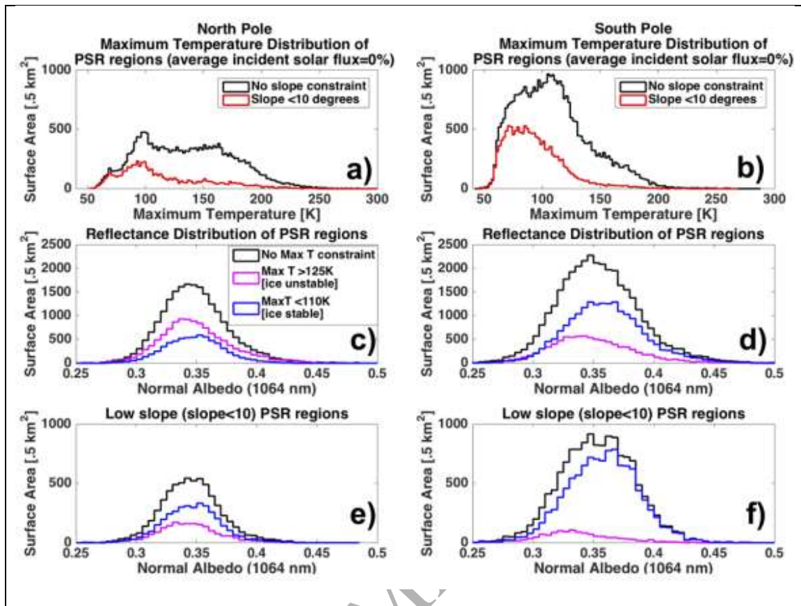
Figure 8. a,b) Maximum temperature distribution of all PSR regions (defined as having average incident solar flux of 0%), compared to the maximum temperature distribution of low slope (slope < 10°) PSR regions, for the North( a ) and South( b ) poles (maximum temperature bin width=2K). Many portions of these PSRs exhibit maximum temperatures far above the stability threshold for water ice. c,d) LOLA normal albedo distribution of low temperature PSR regions capable of sustaining surface water frost (maximum temperature < 110K, blue), compared to reflectance distribution of high temperature PSR regions incapable of sustaining surface frost (maximum temperature > 125K magenta) at the North( c ) and South( d ) poles (reflectance bin width=0.005). Reflectance distribution of PSR regions with no temperature constraints included for comparison purposes (black) (reflectance bin width=0.005)] e,f) same as c, d but constrained to low slopes (< 10 degrees) to minimize mass wasting influence. [1.5 column]
