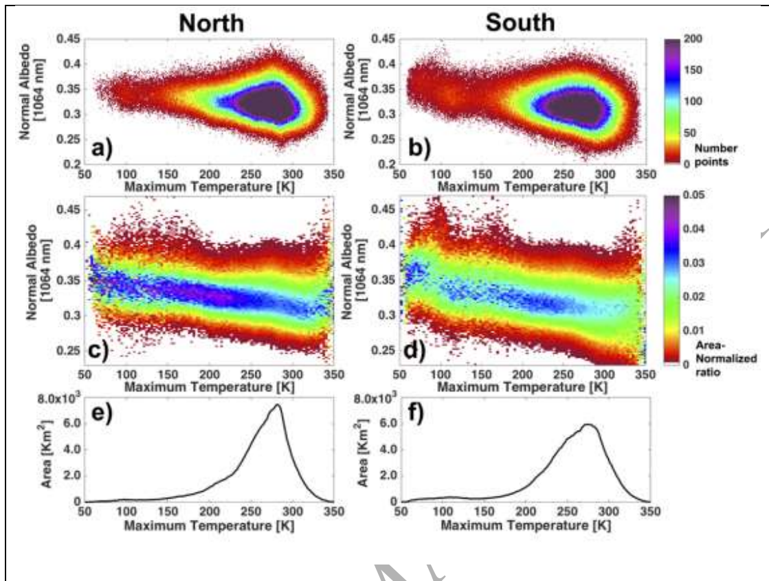
Figure 1 . Plots illustrating the relationship between Diviner maximum temperature and LOLA 1064 nm reflectance at the lunar poles (defined as regions within 20 latitude of the pole). Top: Two-dimensional histograms of 1064 nm normal albedo vs. maximum temperature for the lunar North (a) , and South (b) polar regions. Normal Albedo bin width=0.002, Maximum Temperature bin width=1K; Center: Two-dimensional histograms of 1064 nm normal albedo vs. maximum temperature where data within each temperature bin is normalized to the total area within that temperature bin, for the lunar North (a) , and South (b) polar regions. Normal Albedo bin width=0.002, Maximum Temperature bin width=3K. Histograms showing maximum temperature distribution for the North (e) and South (f) poles
