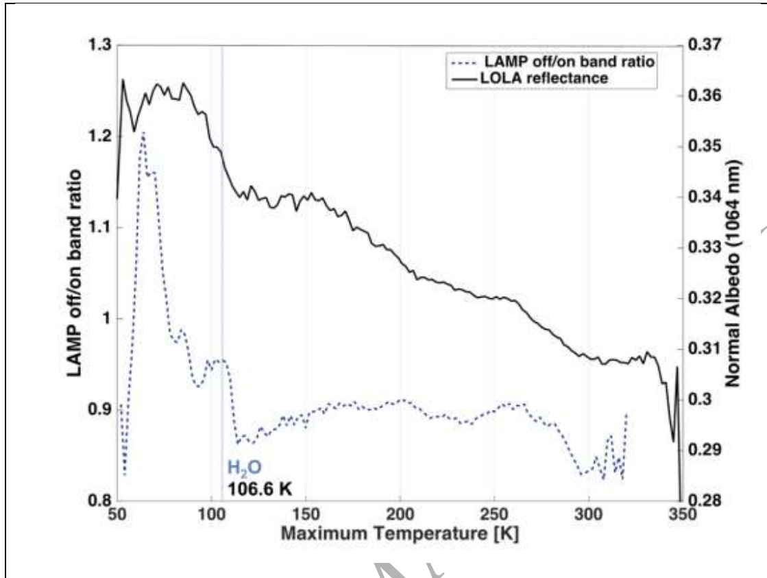
Figure 6. Plot comparing LAMP water band ratio value (positively correlated with increasing water abundance) as a function of maximum Diviner temperature [Hayne et al. , 2015], with average South polar LOLA reflectance as a function maximum Diviner temperature derived in this study. Maximum temperature bin width=2K. LOLA reflectance data shown include all data within 20 degrees of the South Pole. The volatility threshold for water ice, derived by Zhang & Paige [2010] for 1mm/Gyr is included for comparison. [1 column]
