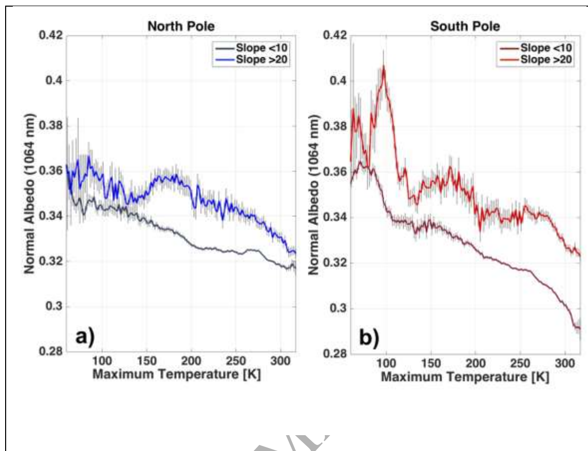
Figure 4. Average 1064 nm reflectance as a function of maximum temperature for low slope (slope < 10°) and high slope (slope > 20°) areas for the North (a) and South (b) polar regions. Maximum Temperature bin width=2K. Reflectance average plotted with 2\sigma errors (standard error of the mean). [1.5 column]
