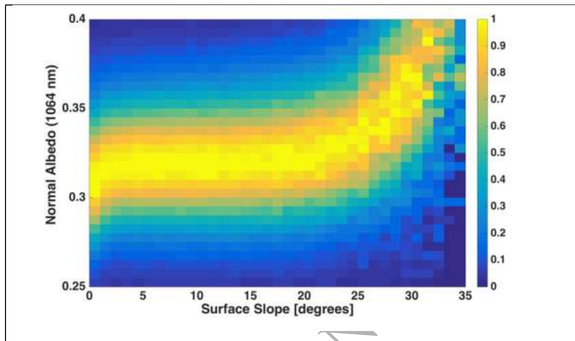
Figure 3. Two-dimensional histogram that displays mode-normalized LOLA reflectance distribution as a function of surface slope for the North and South pole. Reflectance bin width=0.005 and slope bin width=1 degree . The strong influence of surface slope is a potential source of temperature-independent bias on the reflectance-temperature relationships observed in the polar regions. [1 column]
