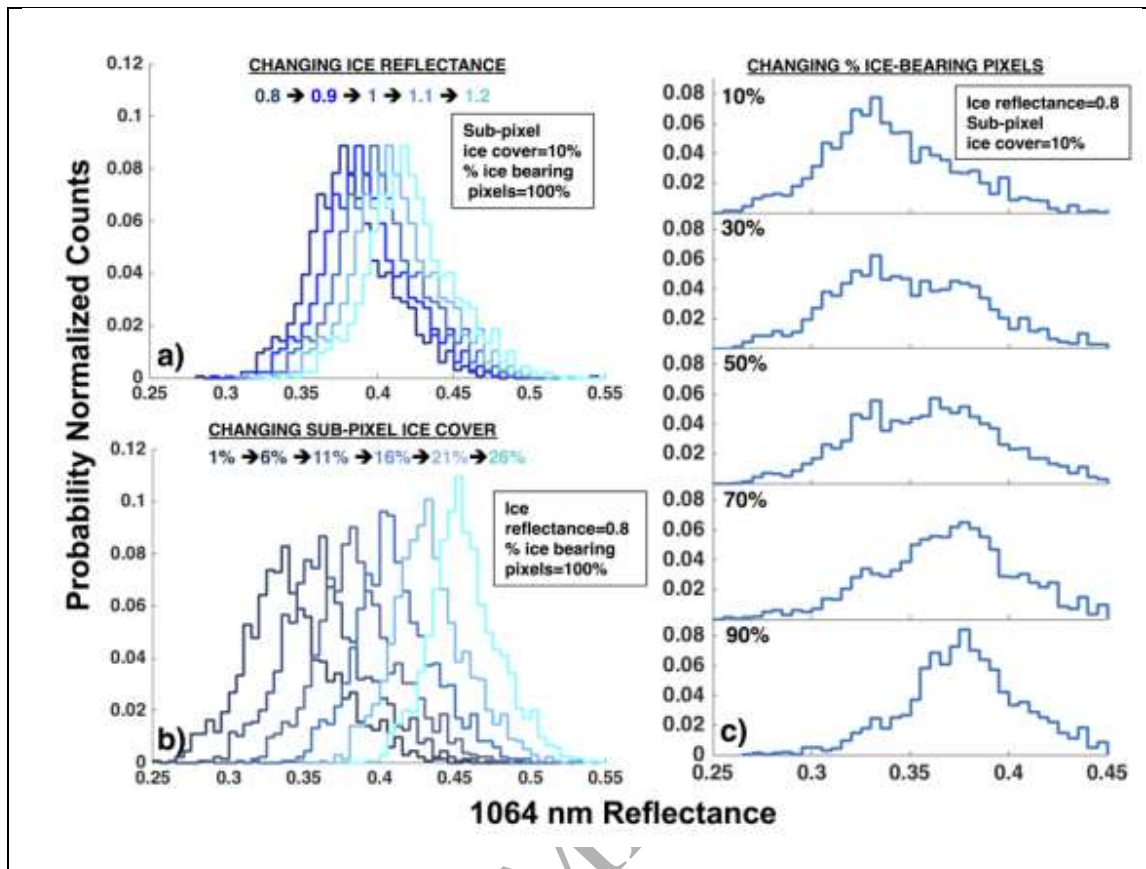
Figure 9. Results showing the effect of varying our three ice model input parameters: ‘ice reflectance’ (a), ‘sub-pixel ice cover’ (b), and ‘percent ice bearing pixels’ (ice-heterogeneity)(c). This model applies ice-brightened material to an ice free distribution via linear mixing. The ice-free starting distribution was we chose the reflectance distribution of low slope (slope <10^\circ ) South-polar PSRs (average incident flux=0%), with maximum temperatures high enough ( >125\text{K} ) to preclude the preservation of surface ice. Reflectance bin width of all histograms equals 0.005. [1.5 column]
