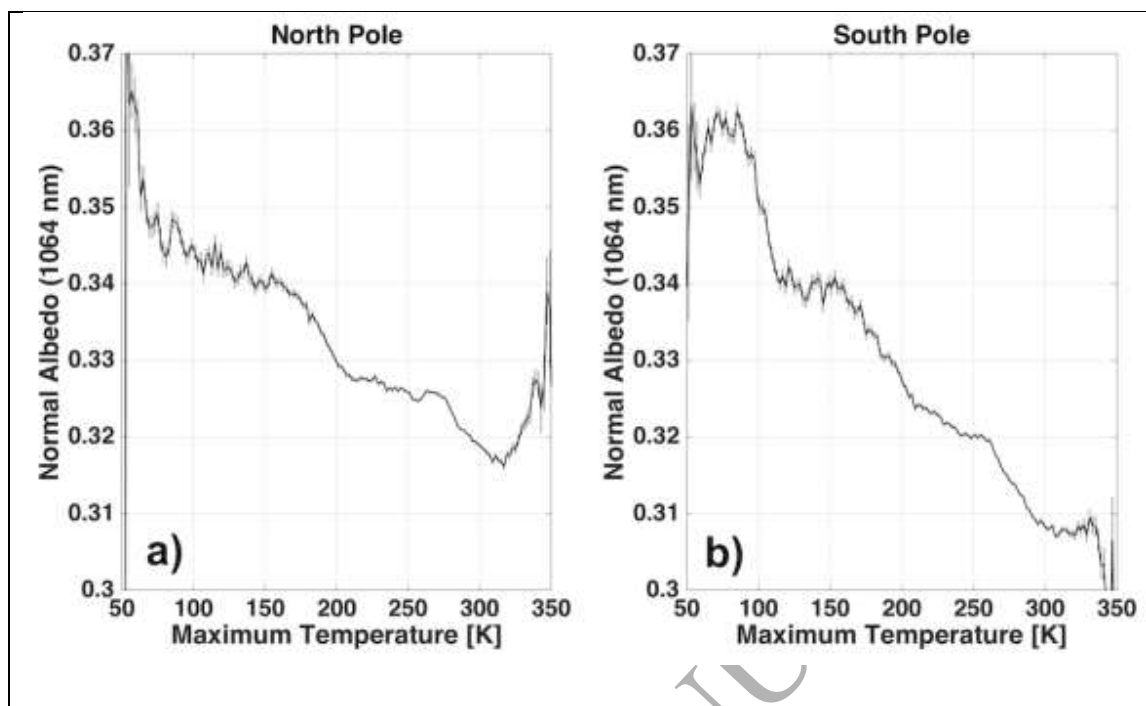
Figure 2. Average reflectance plotted as functions of maximum temperature for the (a) North and (b) South poles. Maximum temperature bin width=1K. Average reflectance curves are plotted with 2\sigma standard error of the mean.
