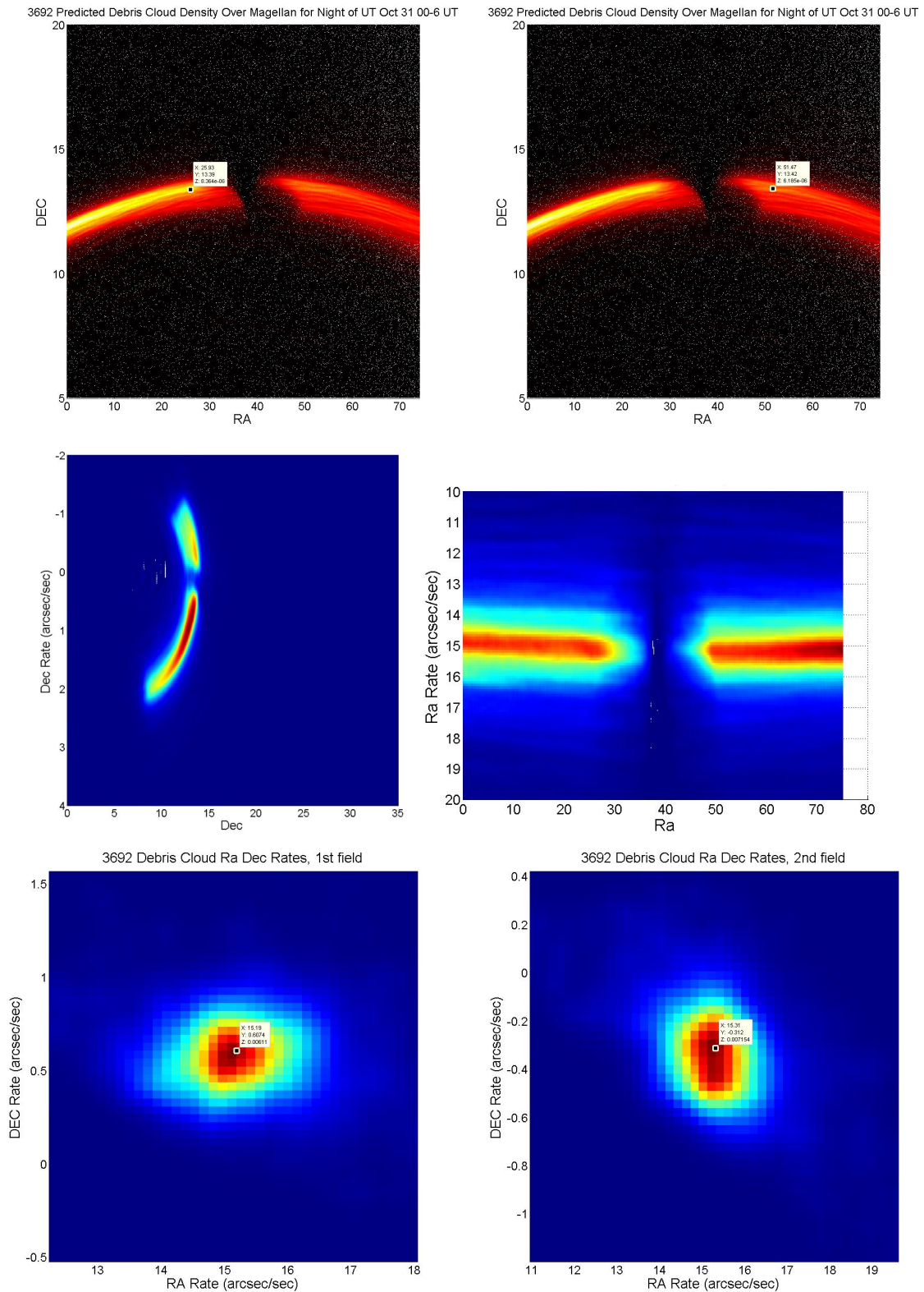
Figure 6. The same debris cloud as in Fig. 3 but propagated forward to an observing period centered on 31 October 2014. During these observations, the Earth's shadow prevents any objects at the anti-solar point from reflecting sunlight (illustrated in the top 4 figures as blank regions). The RA and Dec rates vary between the two regions so it is necessary to calculate the tracking rates for each individual region. The optimized RA and Dec tracking rates for the two regions are displayed in the bottom most figures.
