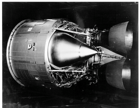
Figure 1. Titan 3C Transtage prior to launch
