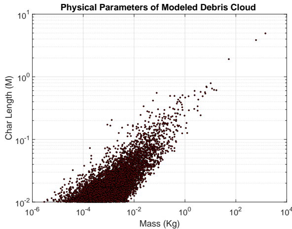
Figure 2. The Characteristic Length vs the Mass of the objects produced using the NASA Breakup Model. These objects were propagated forward from the location and time of the 4 June breakup and used to predict locations and tracking rates of possible associated debris over Las Campanas Observatory. Objects as small as 1cm were modeled but likely beyond the detection limit of the Baade telescope.
