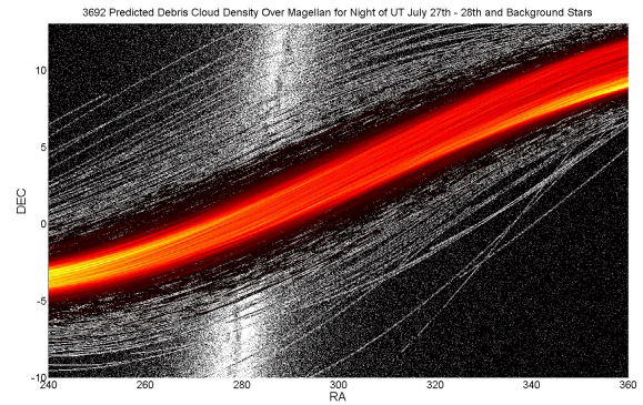
Figure 3. A density plot showing the path of the modeled debris objects in RA and Dec space over Las Campanas Observatory on the nights of 27-28 July 2014. The regions of sky that are red to orange in color have more of the modeled objects passing through that location than the darker regions. Background stars are also plotted and used for reference to minimize stellar contamination during the object detection process.
