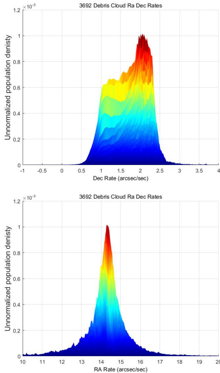
Figure 5. Same as Fig. 4 but with the RA/Dec rate components separated for clarity. The individual peaks show the most common RA/Dec rates expected for the Titan Transtage debris during the observing period.
