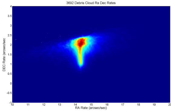
Figure 4. Density plot showing the distribution of the RA and Dec rates of the propagated modeled debris objects during the night of observations over Las Campanas Observatory. The peak values represent the tracking rates necessary for most objects to appear near-circular on the focal plane, thus minimizing the noise inherent in detections that are smeared across many pixels. Objects detected moving at these rates are theorized to be more likely associated with the breakup cloud rather than background debris.
