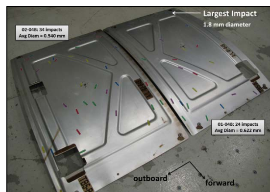
Figure 11. Inspection results on airlock shields
