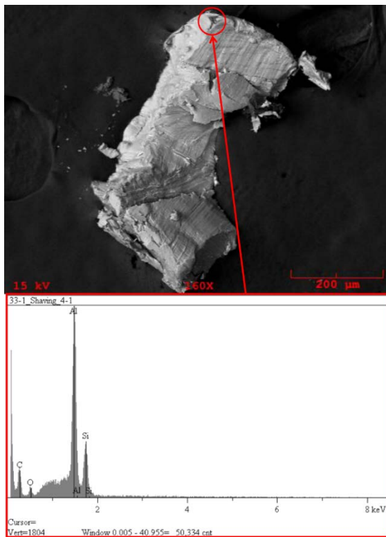
Figure 18. SEM results of sample from crater 33-1 indicate trace silica melt in the aluminum
