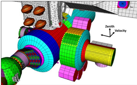
Figure 19. Airlock shield FEM
