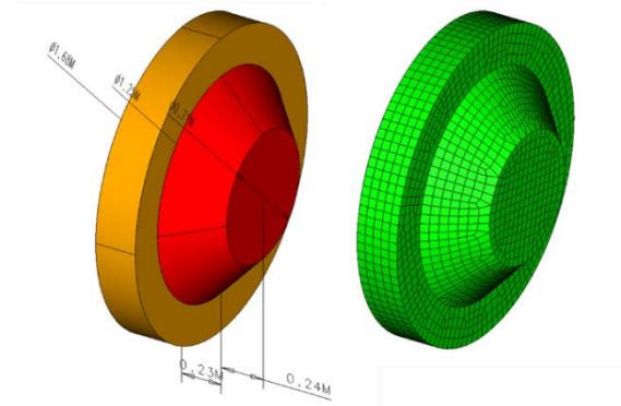
Figure 8. PMA-2 cover surface geometry and FE model
