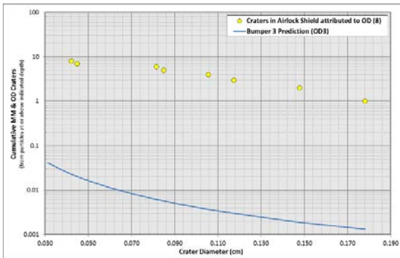
Figure 21. Observed craters from ORDEM 3 compared to Bumper 3 predictions
