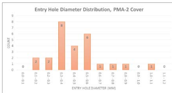
Figure 4. Distribution of PMA-2 entry hole sizes
