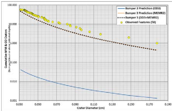
Figure 20. Observed craters from ORDEM 3 and MEMR2 compared to Bumper 3 predictions
