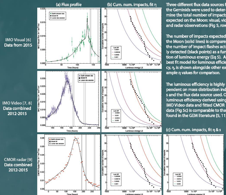
Fig 5: Luminous efficiency analysis results
