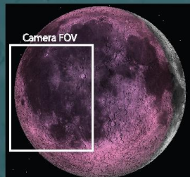
Fig 1: GEM visibility (pink) 14-15 Dec 2015
