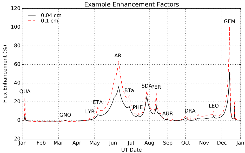
Figure 9. MEO annual meteor shower forecast sample output. This plot shows the enhancement of the total flux due to meteor showers for the smallest two reference particle sizes. Fluxes, fluences, and enhancement factors assume that the spacecraft surface in question is oriented to face the shower radiant, maximizing the intercepted flux.
