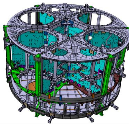
Figure 5. ESM Primary Structure.
