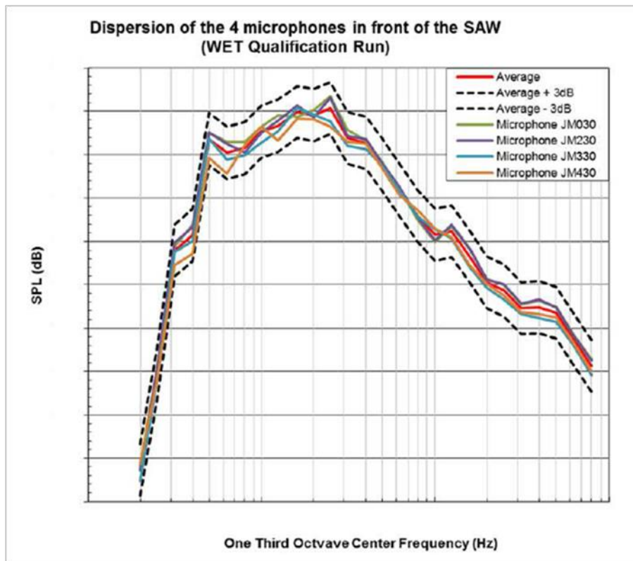
Figure 20. Homogeneity of the Acoustic Level Measured at the SAW QM (Group 124) for AC0248.
