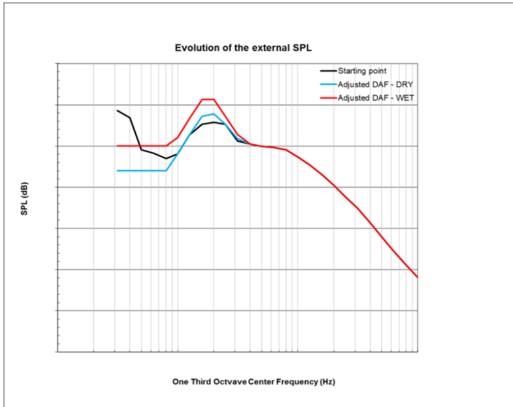
Figure 22. Evolution of the External Excitation Noise.
