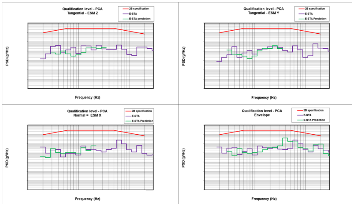
Figure 25. Comparison between Predictions and Measurement near PCA Mounting Points.
