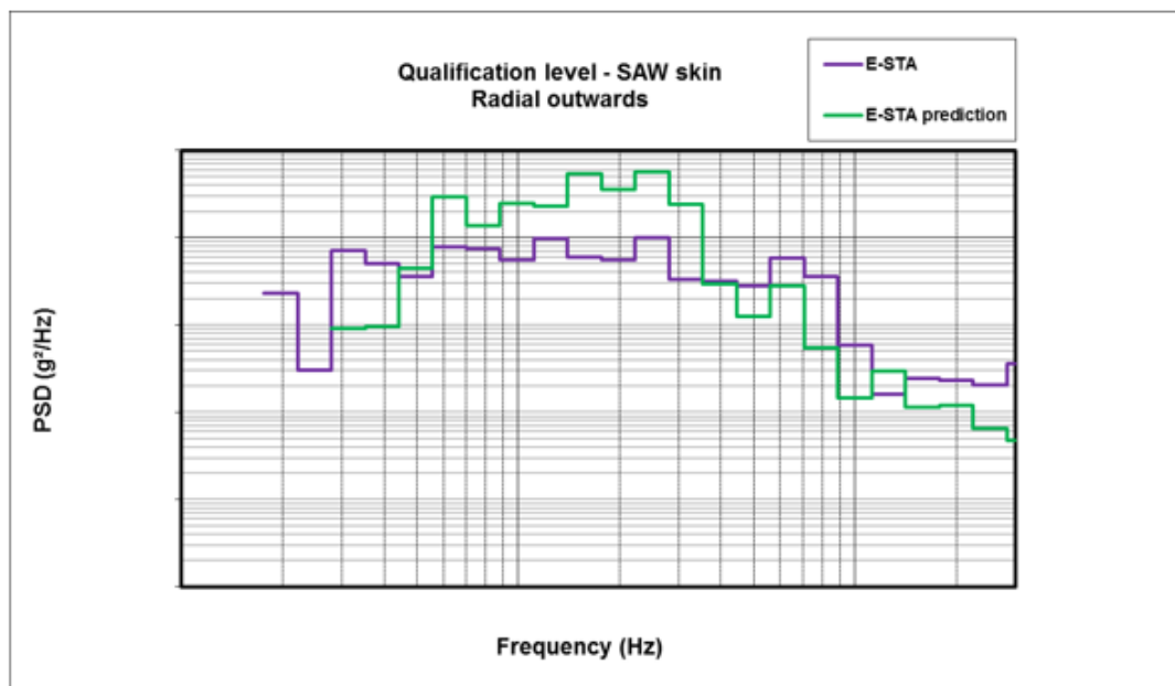
Figure 23. Envelope of Structural Response on SAW Panel 3 (normal direction).
