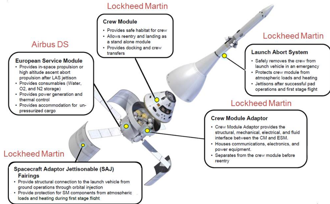
Figure 2. Orion MPCV.
