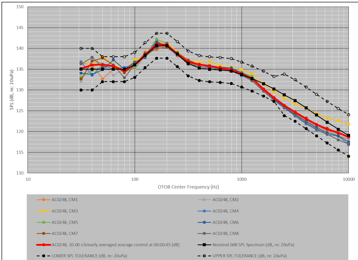
Figure 14. Control Microphone Performance for AC0248.
