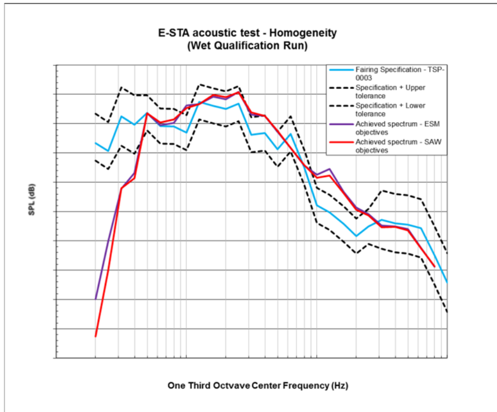
Figure 19. Homogeneity of the Acoustic Field within the SM Outer Cavity for AC0248.
