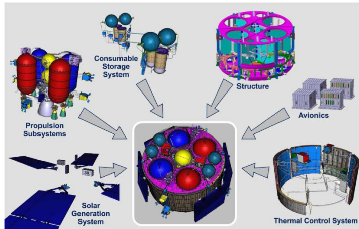
Figure 4. ESM Subsystems.
