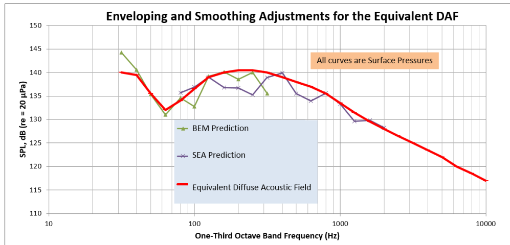
Figure 15. E-STA Qualification External Diffuse Acoustic Field (surface pressures).
