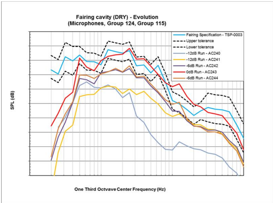
Figure 17. Evolution of the Acoustic Test Levels within the SM Outer Cavity for Dry Tank Configuration.
