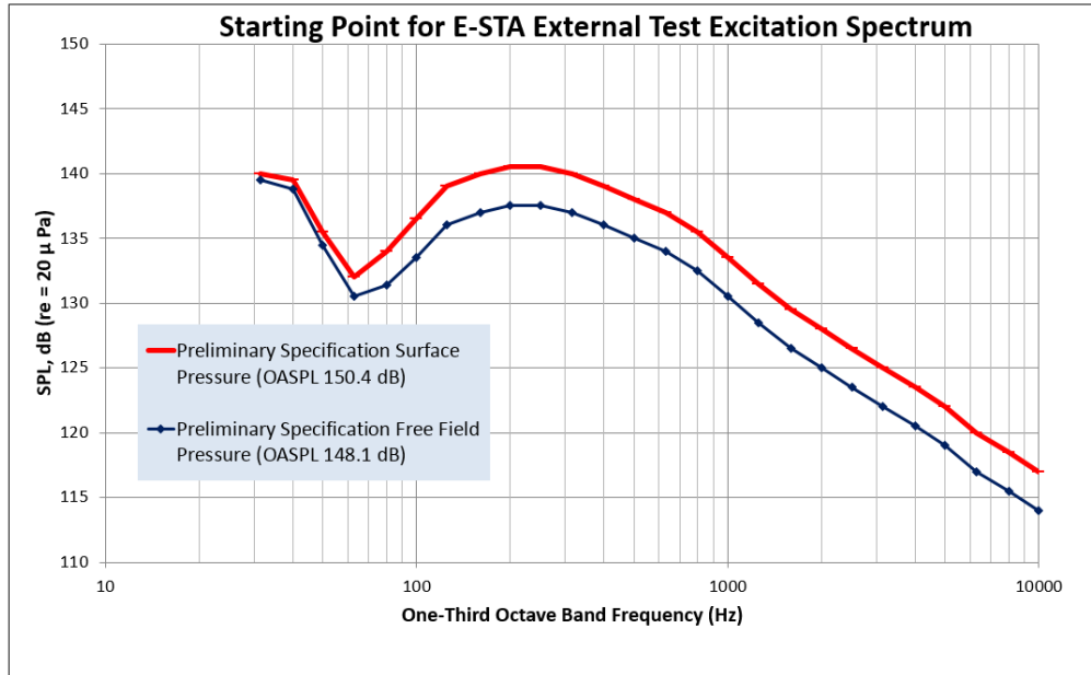
Figure 16. Response-based Starting External Excitation (free-field).
