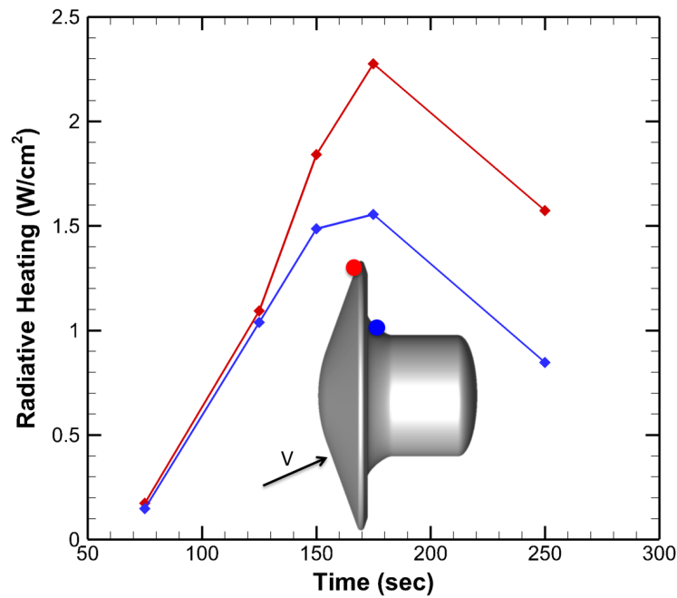
Figure 12: Peak radiation on the forebody and afterbody for aerocapture.
