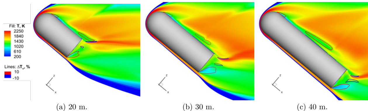
Figure 23: Contours of translational temperature (fill) and relative vibrational temperature (lines) at symmetry plane for varying length.
