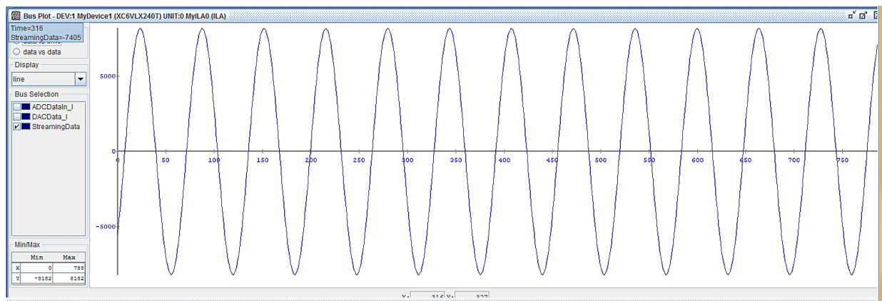
Figure 24.—Receive (Rx)-side streaming data from sine wave using internal loopback.
