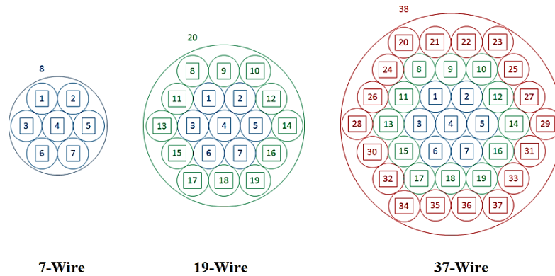
Figure 9: Schematic of the 7-, 19- and 37-wire analysis configurations
