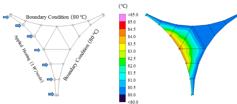
Figure 7: Finite element model configuration for air conduction study
