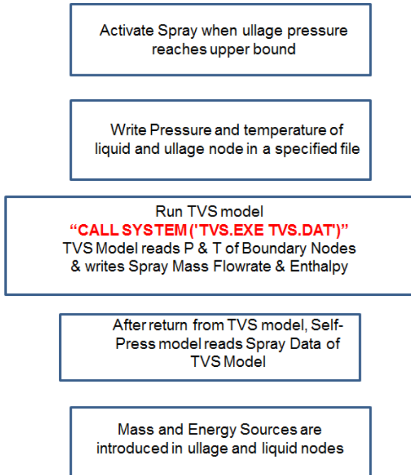
Figure 9. The main steps of model integration
