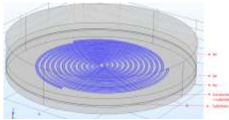
Fig 8. 3D domains built to model removal of particles via spiral-shaped conductors
