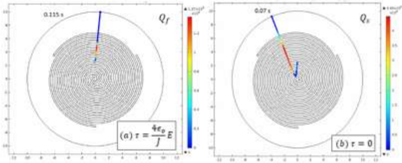
Fig 5. Trajectory and velocity of a dust particle modeled with two charging times: a) equation 3, b) 0,
