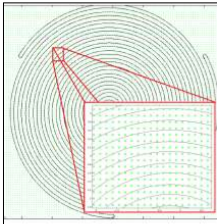
Fig 6. Initial distribution of 8,690 particles evenly dispersed throughout the spiral-shaped-conductor removal system.
