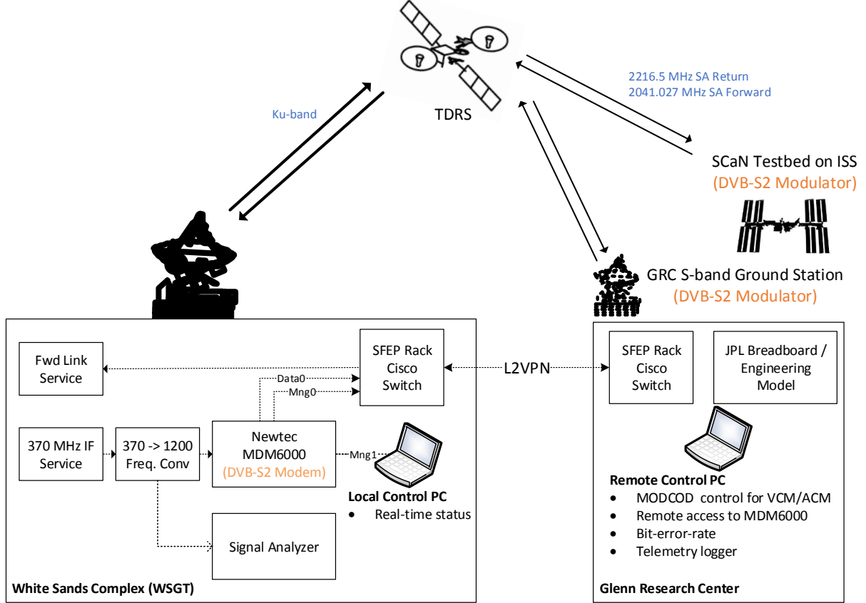
Fig. 2. Test Configuration
