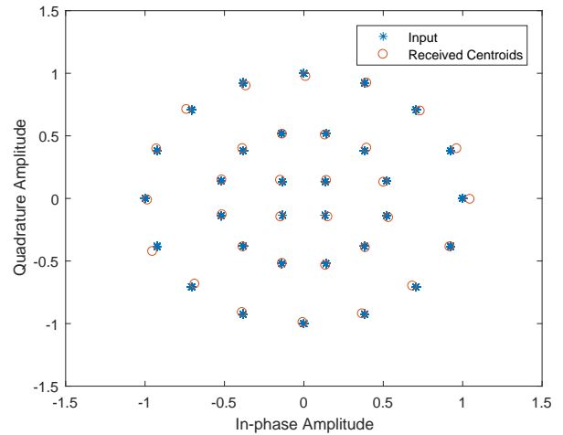
Fig. 32. Observed TDRS Nonlinearity
