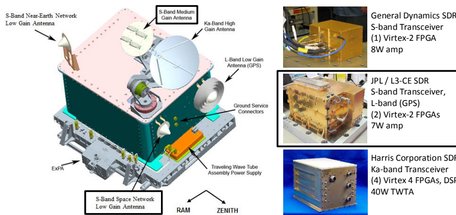
Fig. 1. SCaN Testbed
