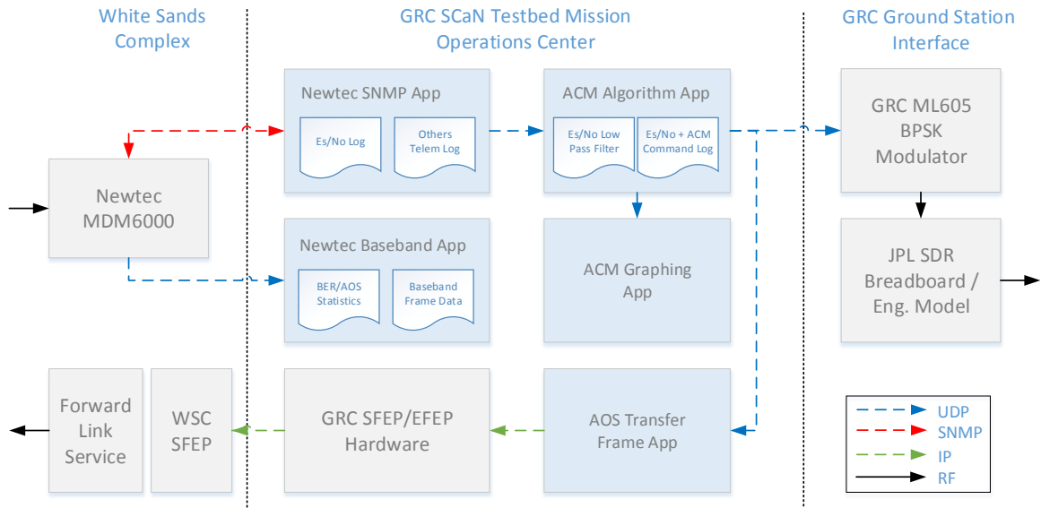
Fig. 6. Ground System
