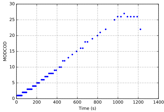
Fig. 10. MODCOD vs Time
