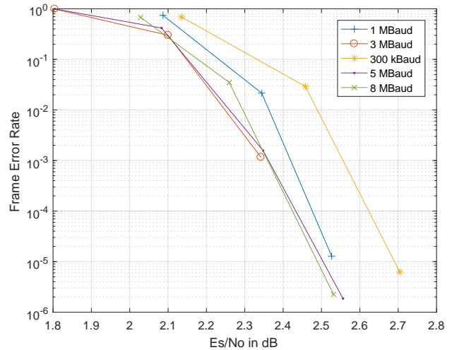
Fig. 9. FER Results for MODCOD 5
