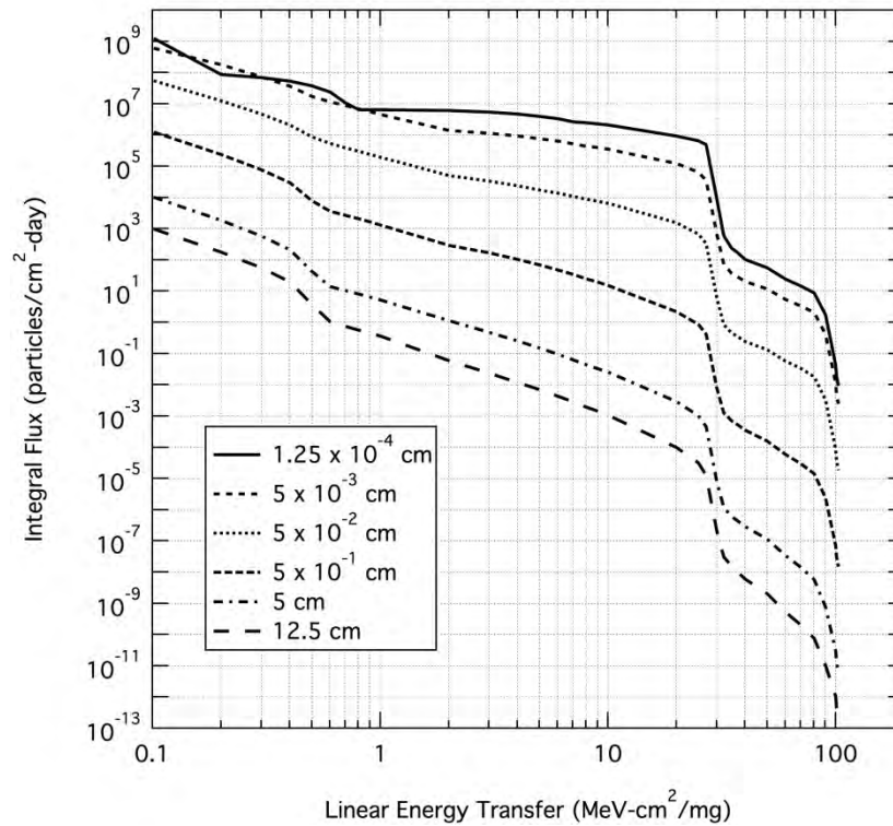
Figure 3.3.2.1-2. SPE Worst Day Integral Flux for Selected Al Shielding Thickness as a Function of LET
