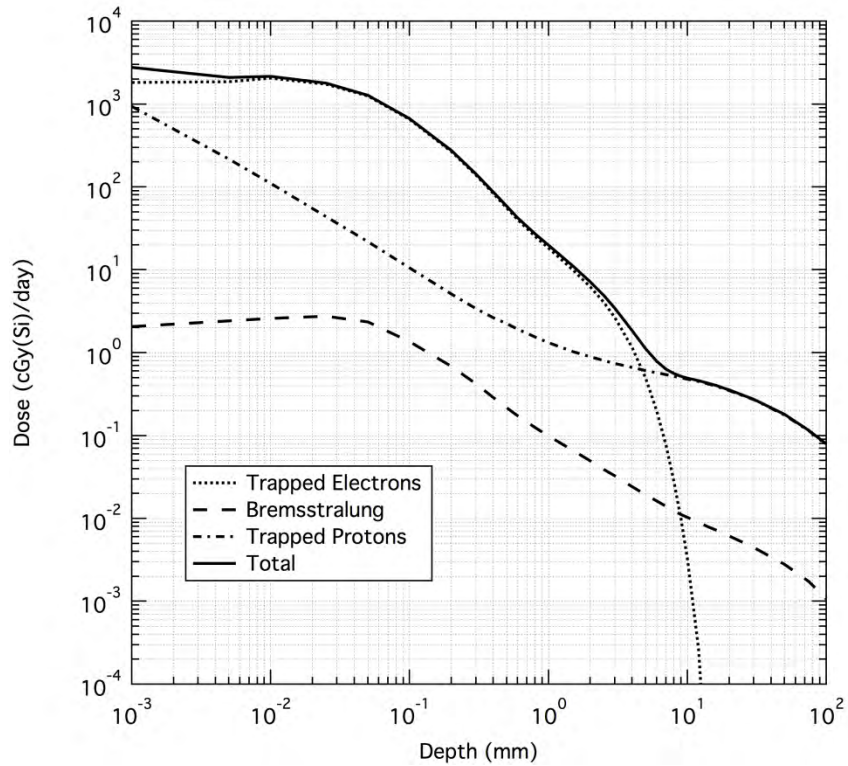
Figure 3.3.1.1-4. Daily Trapped Belts TID Inside Shielding
