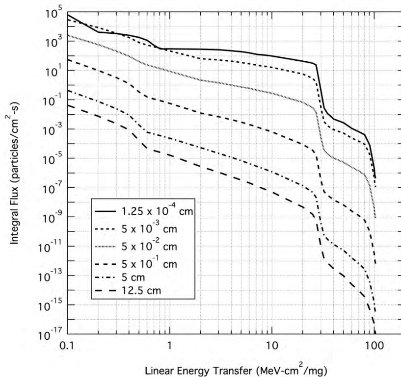
Figure 3.3.2.2.1-1. SPE Integral Peak LET Flux for Selected Al Shielding Thickness as a Function of LET
