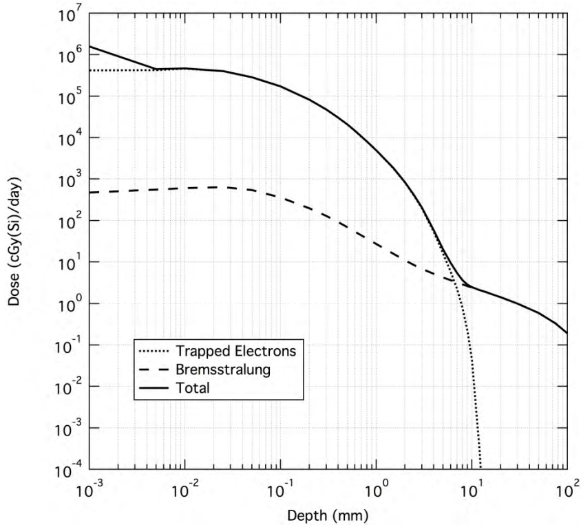
Figure 3.3.1.3-2. Daily Trapped Belts TID Inside Shielding
