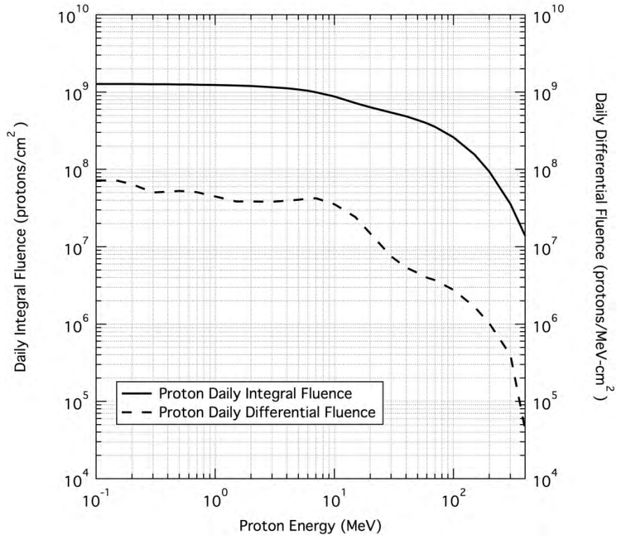
Figure 3.3.1.2.1-1. Daily Trapped Proton Fluences
