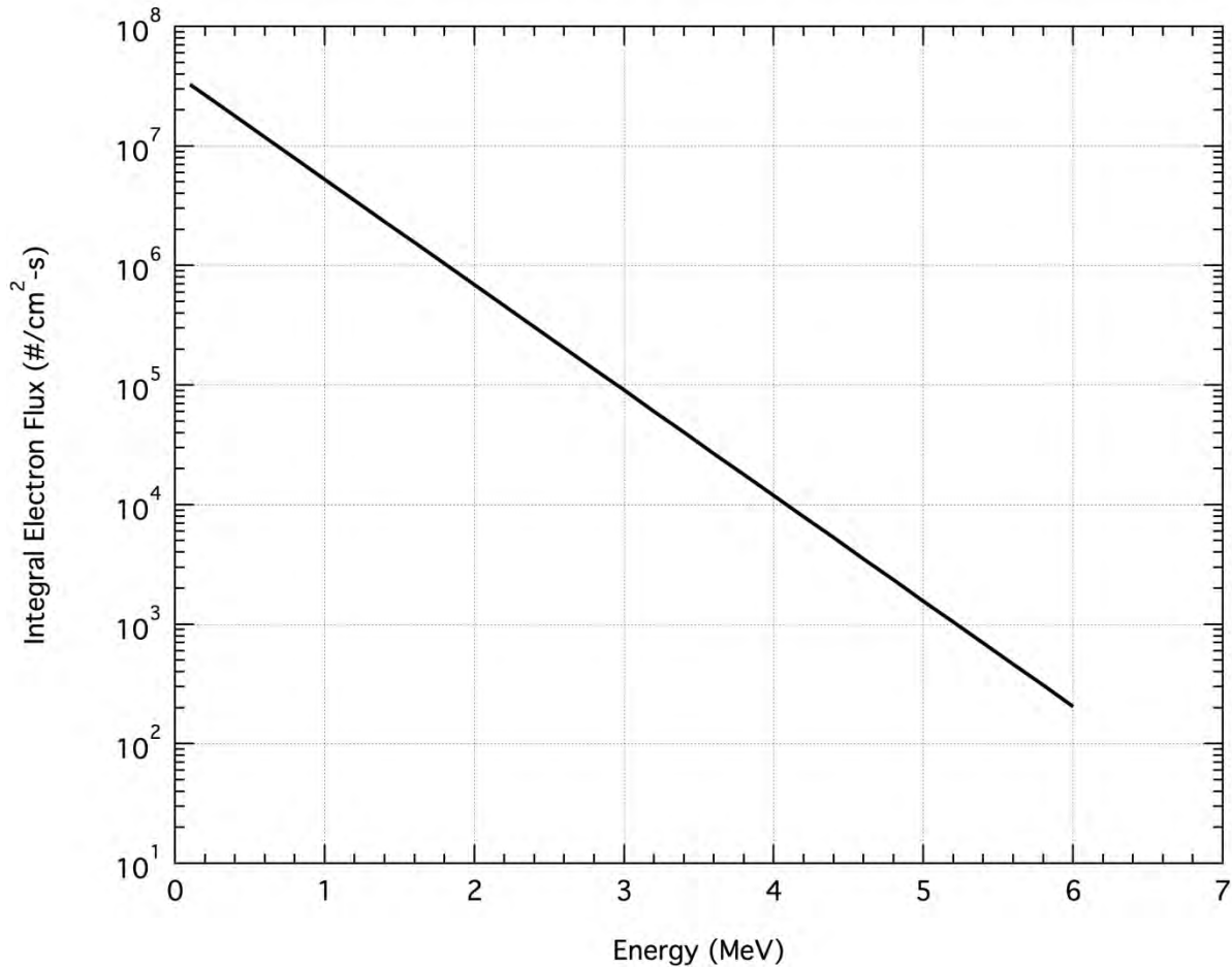
Figure 3.3.3.2.2-1. Radiation Belt Transit Average Integral Electron Flux
