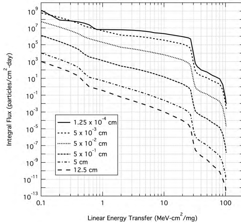
Figure 3.3.2.1-2. ISS SPE Worst Day Integral Flux for Selected Al Shielding Thickness as a Function of LET
