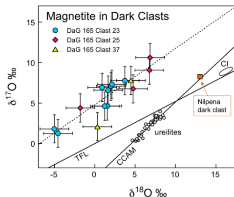
Fig. 1. Oxygen isotope ratios of magnetites from dark clasts in DaG 165. The regression line of all data is shown as a dotted line. Other bulk literature data are from [5, 15].
