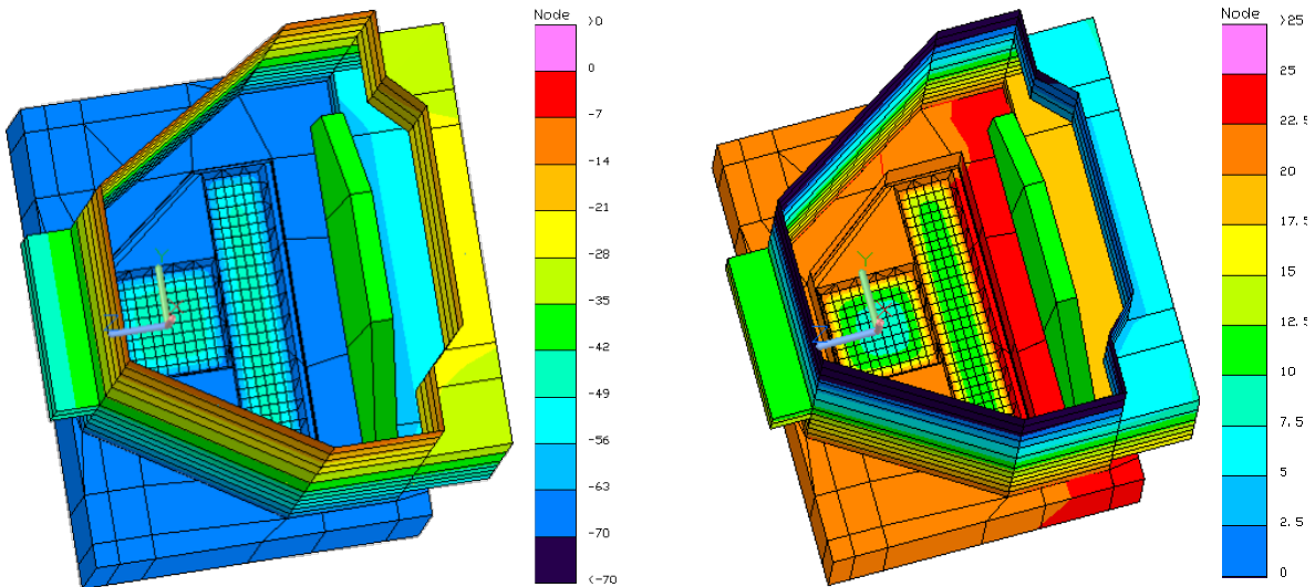
Figure 7. Temperature distribution over the interior (cavity) of the ACIS instrument during normal operations (left panel) with the detector-housing heater off and the focal-plane at -120^{\circ}\text{C} ; during a room-temperature bakeout (right panel) maintaining a cool ( <-60^{\circ}\text{C} ) focal-plane.
