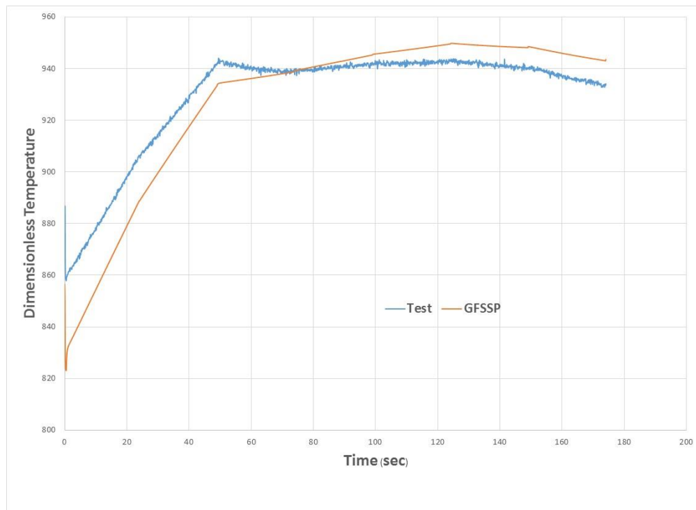
Figure 18. Comparison between predicted and measured temperature for Cubes Test
