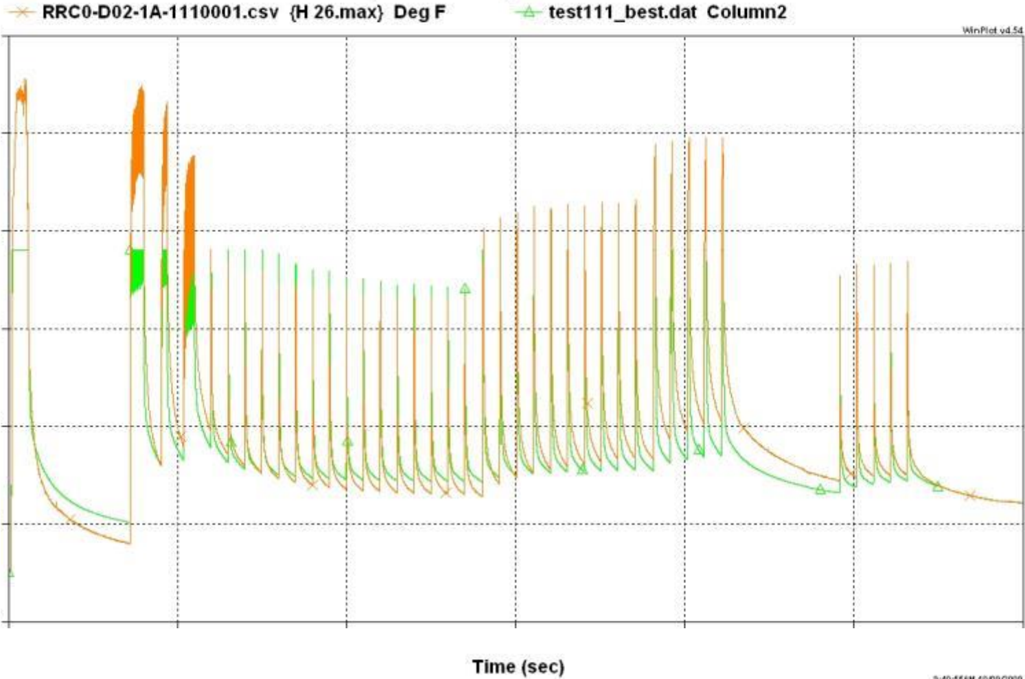
Surface Temperature Comparison For Test -111
