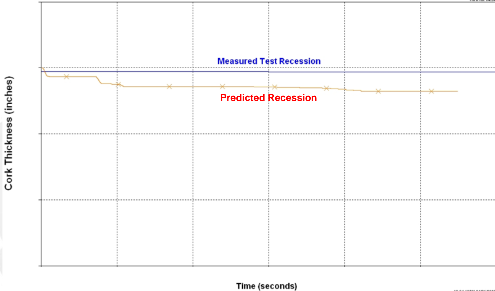
Comparison of Analytical and Measured Recession for Test -111
