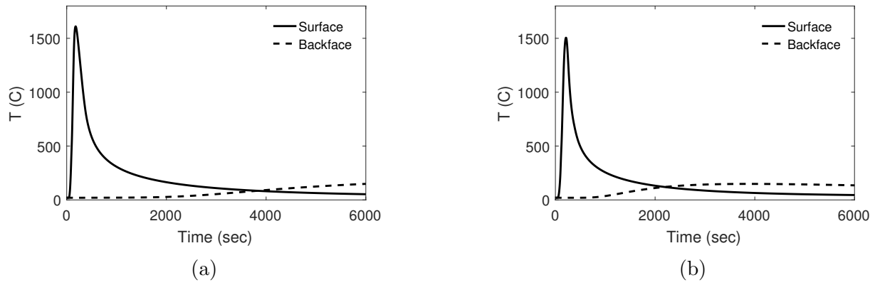
Figure 9: The surface and backface temperatures for the hot structure concept during the (a) aerocapture and (b) entry baseline trajectories.
