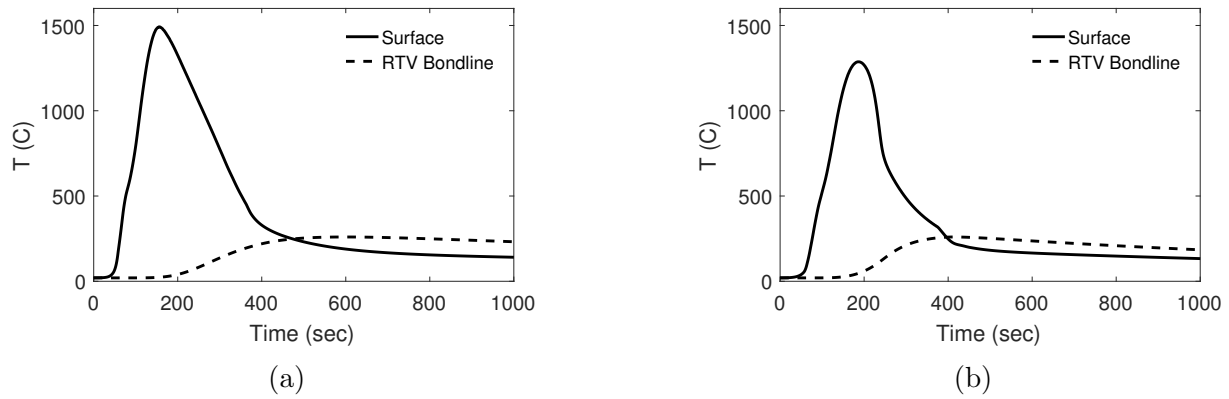
Figure 8: The surface and bondline temperatures for the ablative TPS during the first 1000 seconds of the (a) aerocapture and (b) entry baseline trajectories.
