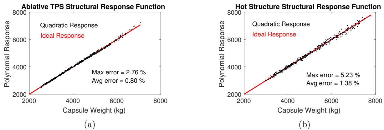
Figure 7: Structural response function output of the (a) ablative TPS and (b) hot structure concept for the capsule design compared to the ideal response.
