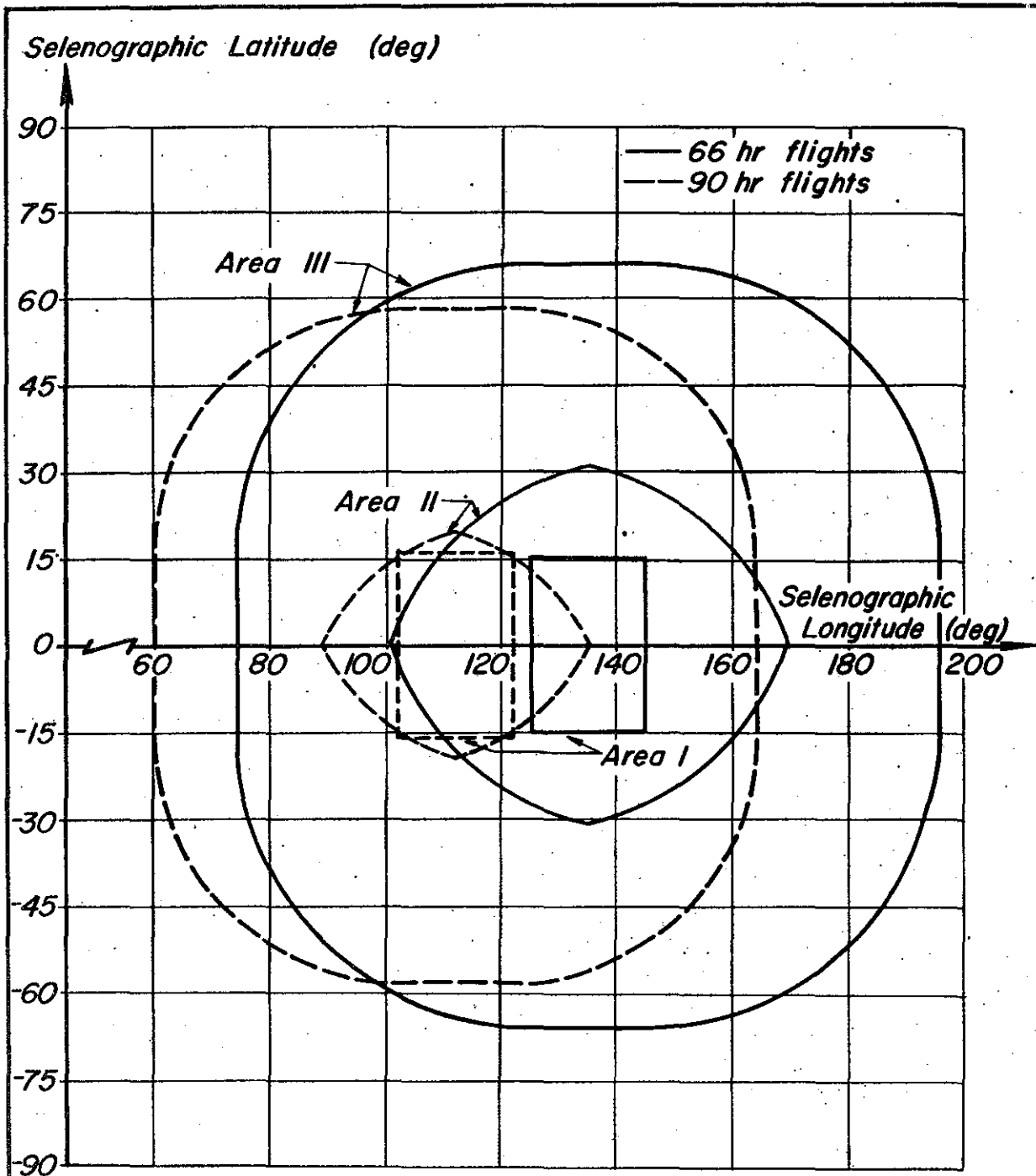
FIG 5. LANDING SITE ACCESSIBILITY FOR 66 HOUR AND 90 HOUR FLIGHTS VIA THE DIRECT MISSION MODE FOR ALL ARRIVAL TIMES
