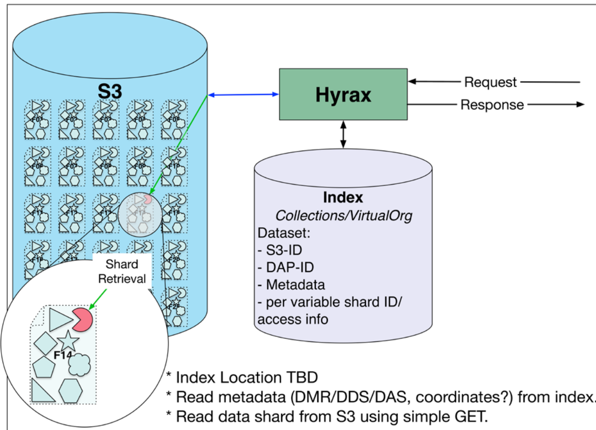
Figure A2-3: Diagram of Architecture 3 in which files are split into multiple pieces (shards) and those shards are stored in S3. OPeNDAP requests are serviced by copying requested shards directly from S3. In this case, the original data are preserved as shards, but the original files are not preserved.
