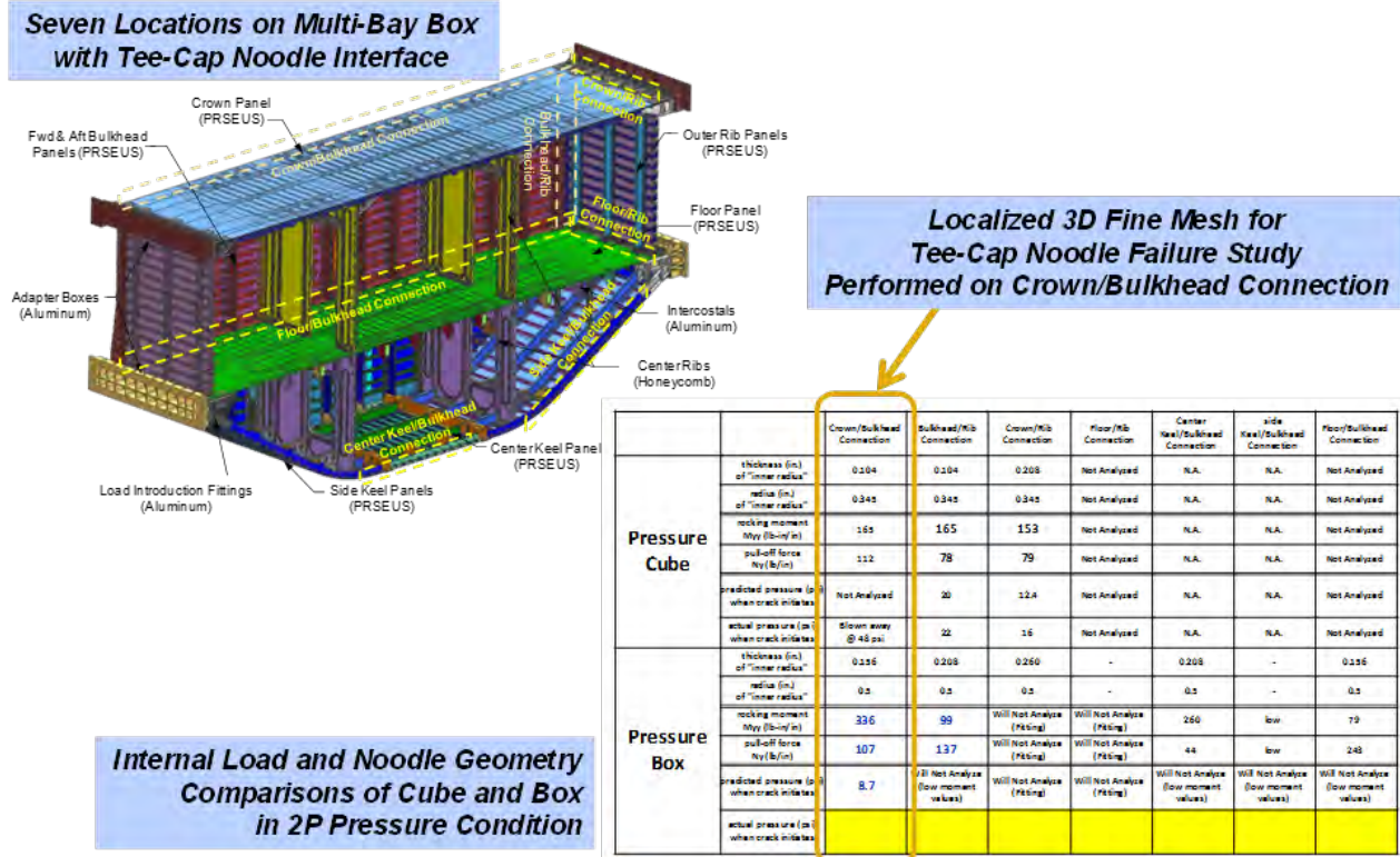
Figure 4-100. Seven Locations With Integral Cap Features Were Investigated
