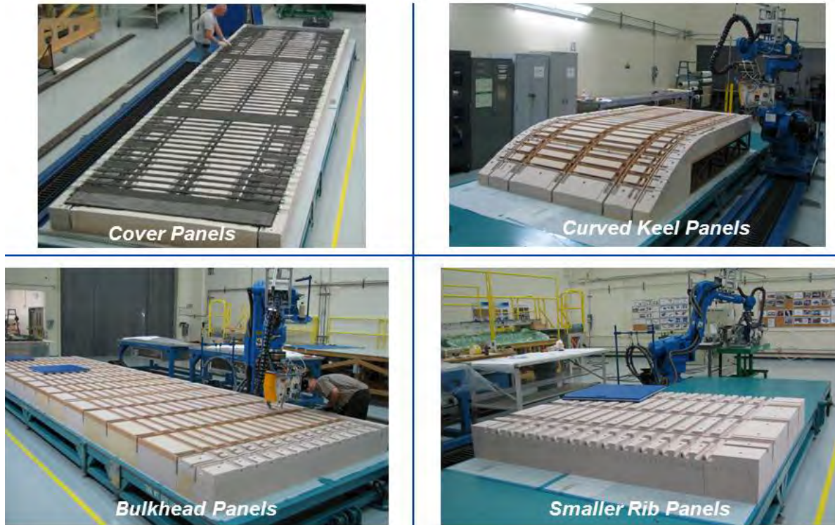
Figure 5-8. Multiple Block Configurations Shown on Common Stitching Table
