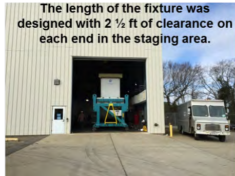
Figure 6-131. MBB Pushed Into COLTS Staging Area
