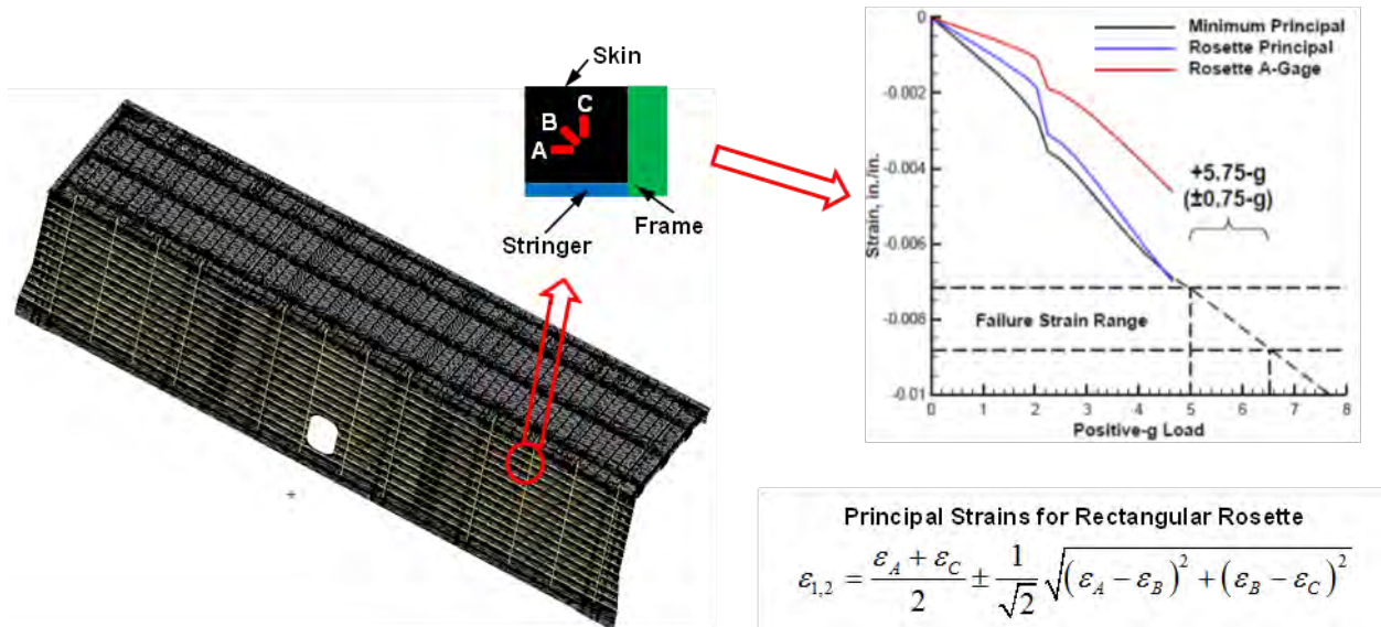
Figure 4-191. Strains on Upper Bulkhead Skin in 5.0-g Condition
