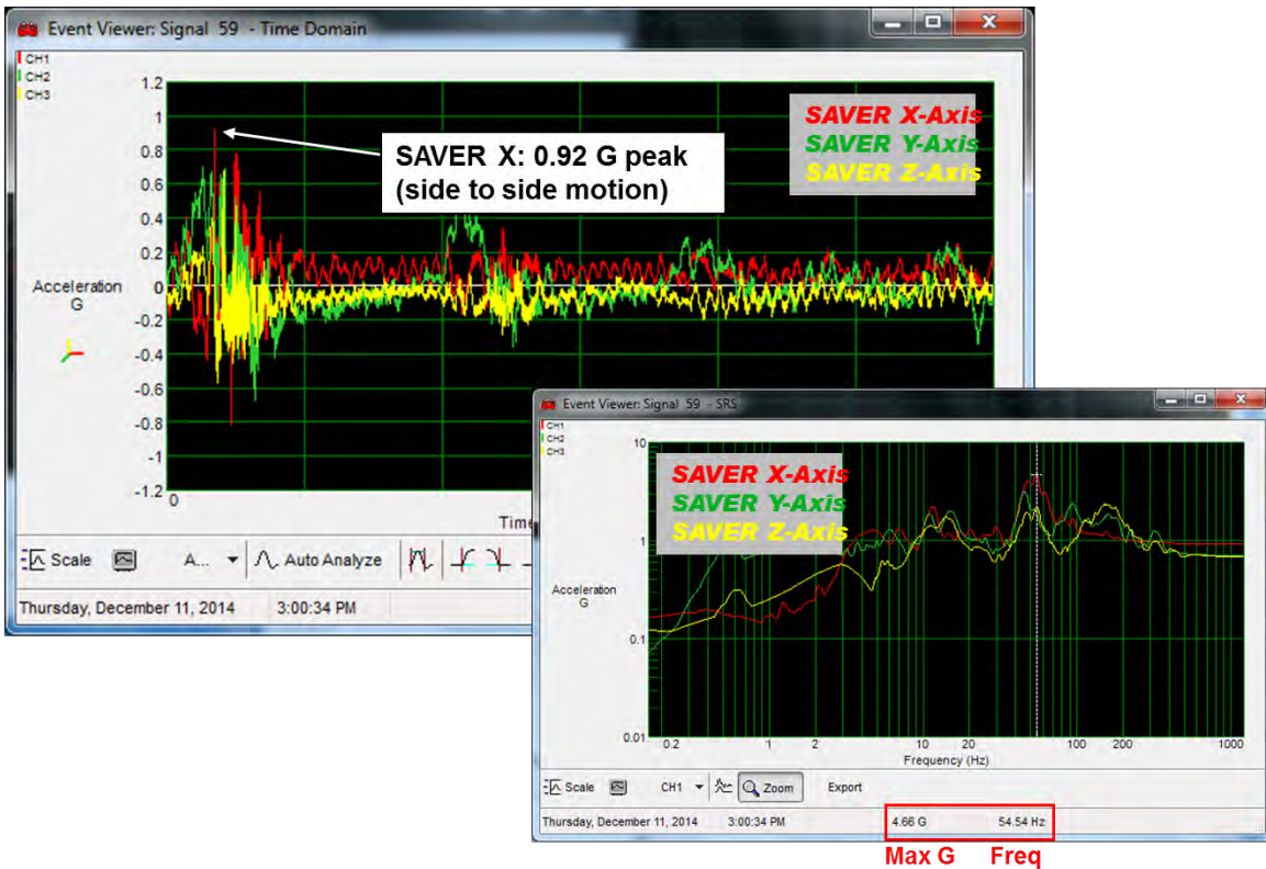
Figure 6-129. Maximum Landing Event (no. 59) at NASA LaRC on 11 December 2014
