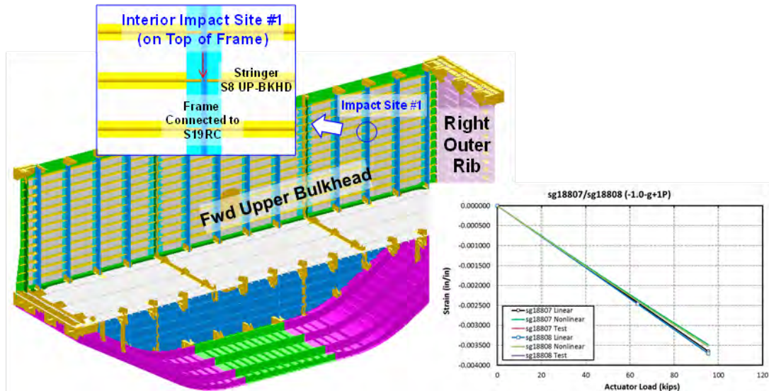
Figure 4-169. Strains on Interior Impact Site no. 1 in -1.0-g + 1P DUL Condition
