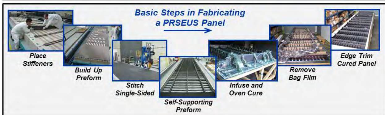
Figure 5-1. Preform Assembly and Cure Tooling Are Primary Toolsets for Panel Fabrication
