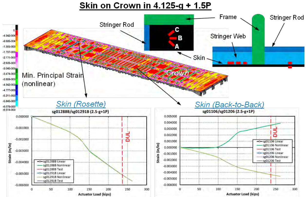
Figure 4-178. Strain on Crown Skin in 4.125-g + 1.5P Condition
