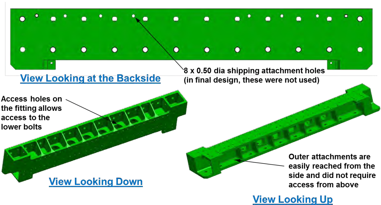
Figure 7-7. Upper Adaptor Fitting
