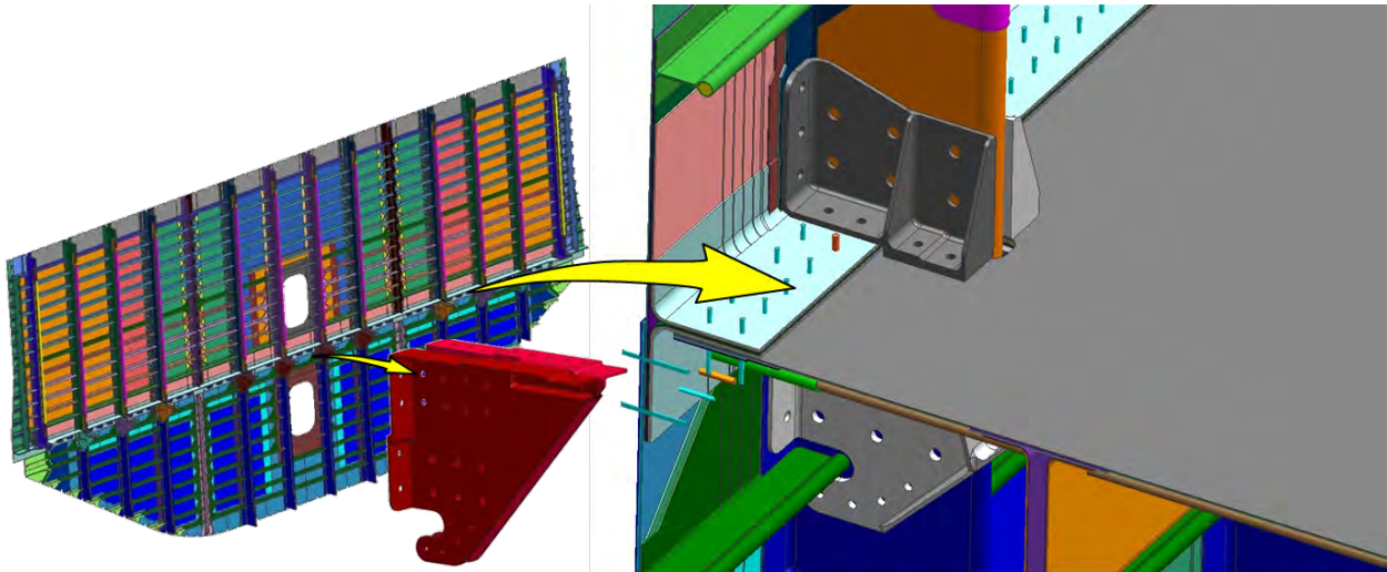
Figure 3-69. Floor Attachment
