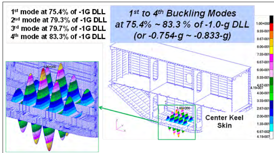
Figure 4-90. First to Fourth Buckling Modes in -1.0-g Maneuver Condition
