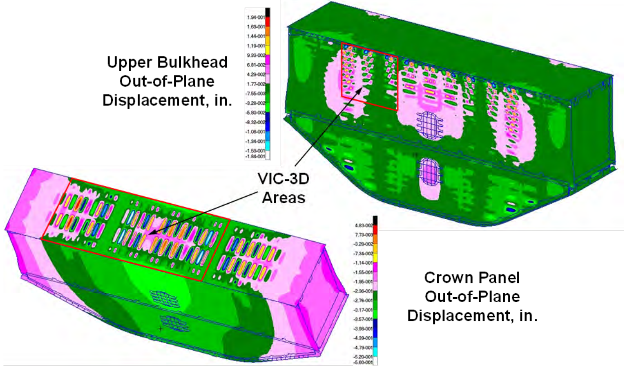
Figure 4-123. VIC-3D Measurements of the MBB in 2.5-g DUL Condition
