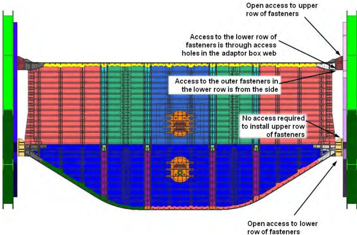
Figure 3-76. Platen Access
