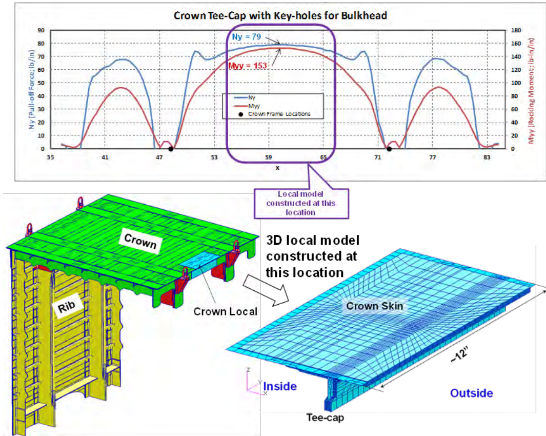
Figure 4-101. Location of 3D Detailed FEM Study of T-cap on the Crown of the Pressure Cube
