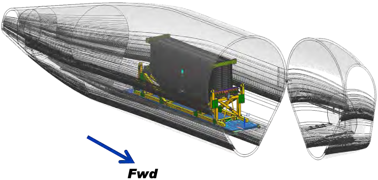
Figure 6-87. MBB Positioned Inside the Super Guppy
