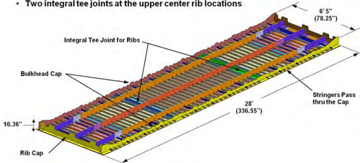
Figure 3-9. Crown Panel Assembly
