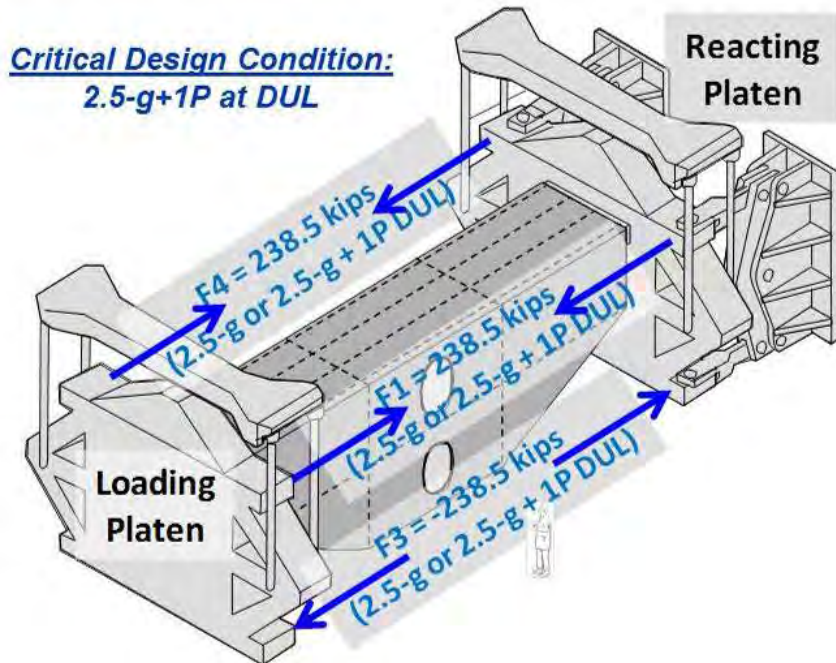
Figure 2-16. COLTS Loads Needed to Generate Critical Compression Loading in the Crown Panel
