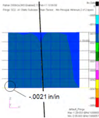
Figure 4-73. Minimum Principal Strains on the Center Frame of the Crown in 2.5-g Condition
