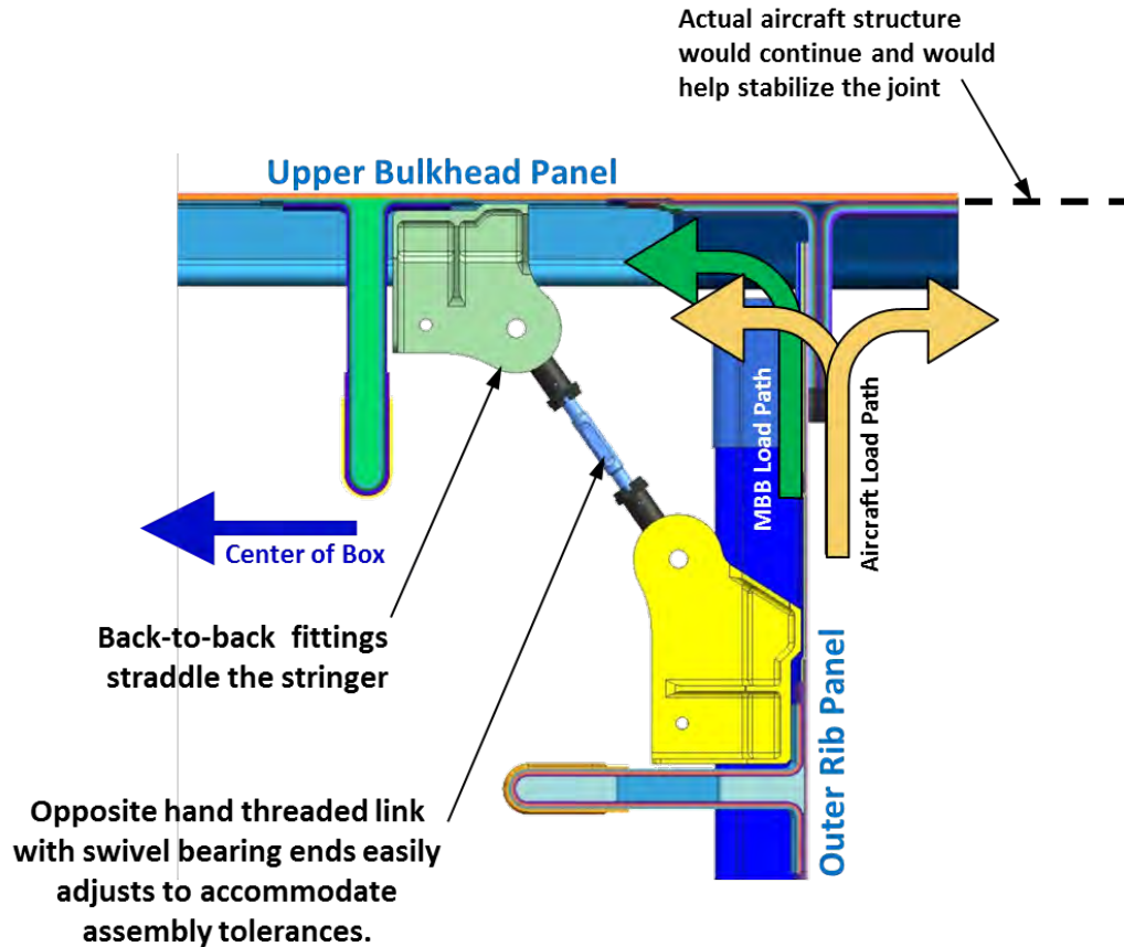
Figure 3-67. Upper-Bulkhead-to-Outer-Rib-Corner Supports
