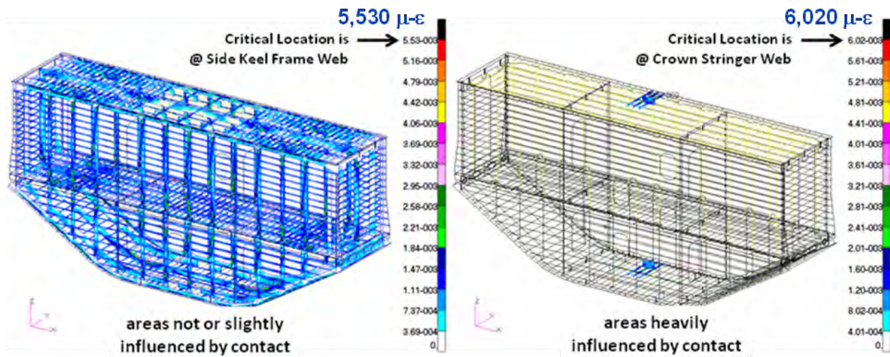
Figure 4-17. Maximum Principal Strains on Composite Stringer/Frame/T-cap Webs in 2P Condition
