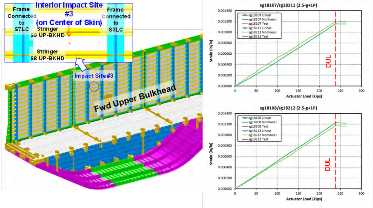
Figure 4-185. Strains on Interior Impact Site no. 3 in 4.125-g + 1.5P Condition
