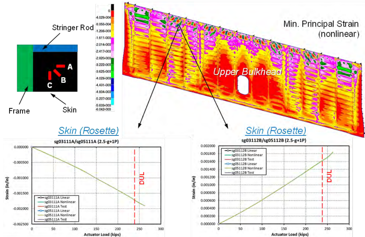
Figure 4-179. Rosette Strains on Upper Bulkhead Skin in 4.125-g + 1.5P Condition
