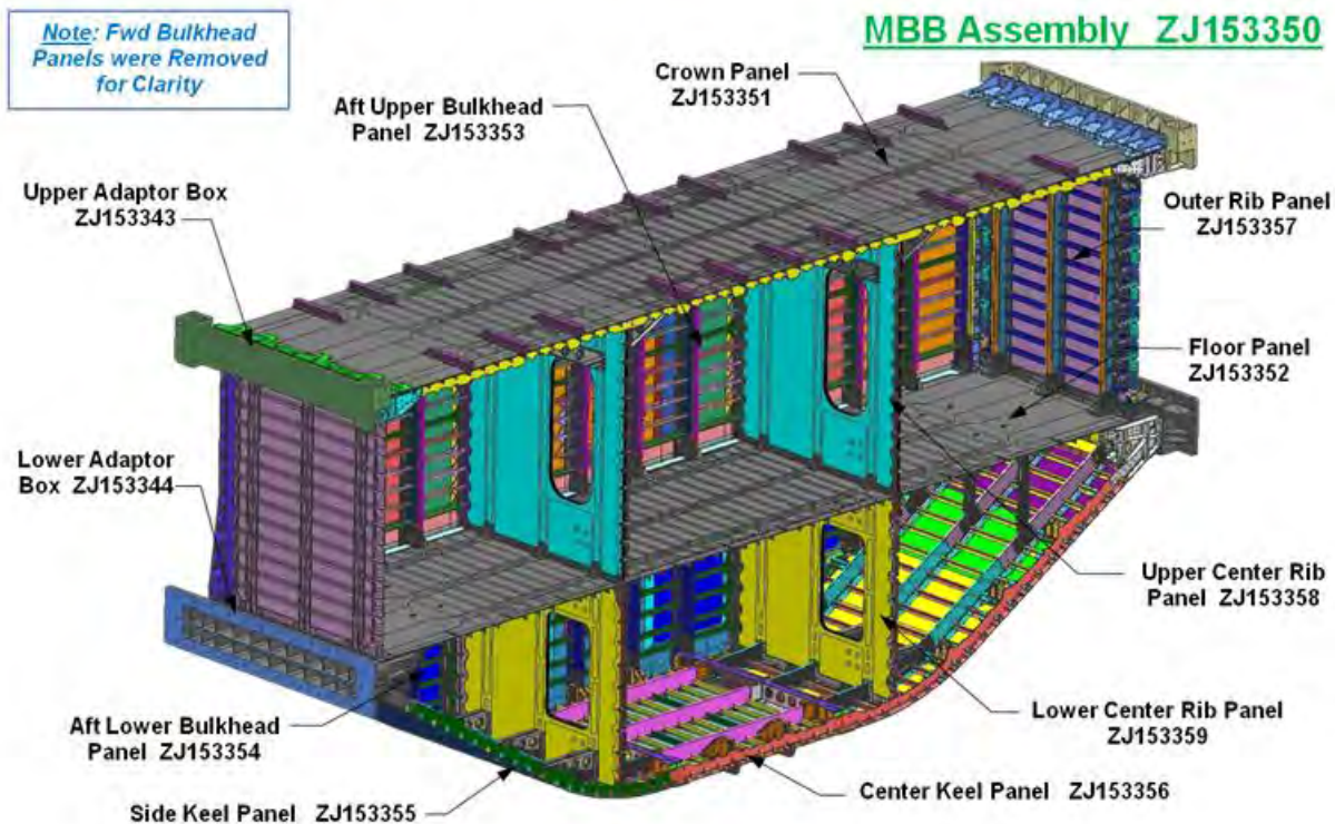
Figure 6-34. Multi-bay Box Assembly Major Components
