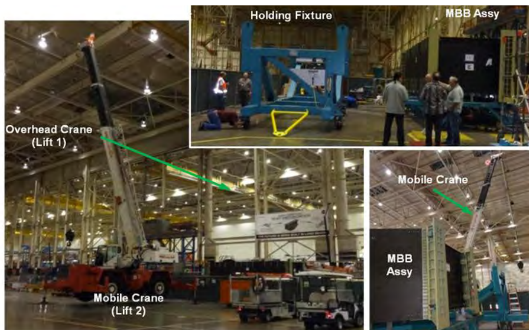
Figure 6-65. Preparing for the Move to the Holding Fixture
