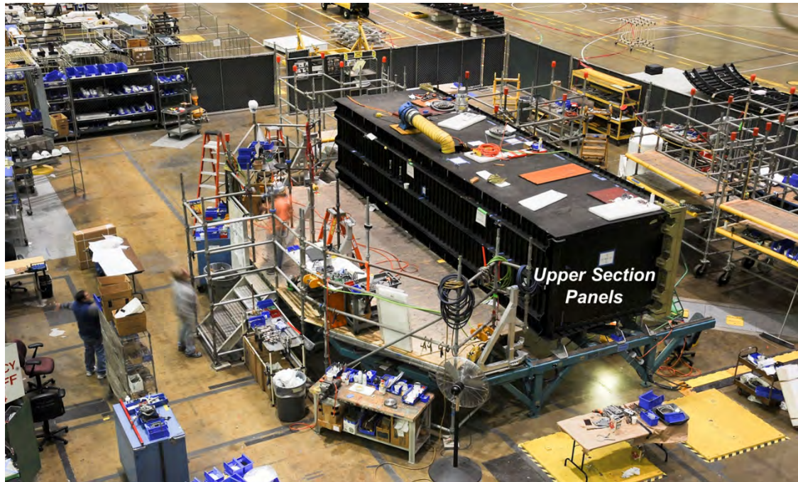
Figure 6-46. Upper Section Panel Assembled With Floor Panel Installed
