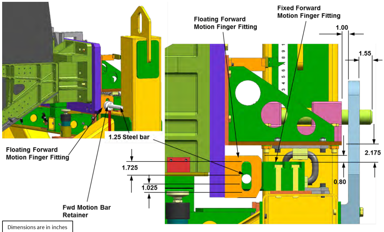
Figure 6-98. Motion Restraint Bar Clearances
