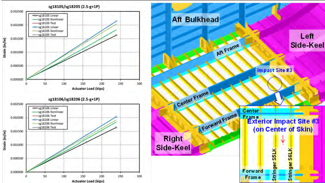
Figure 4-147. Strains on Exterior Impact Site no. 3 in 2.5-g + 1P DUL Condition
