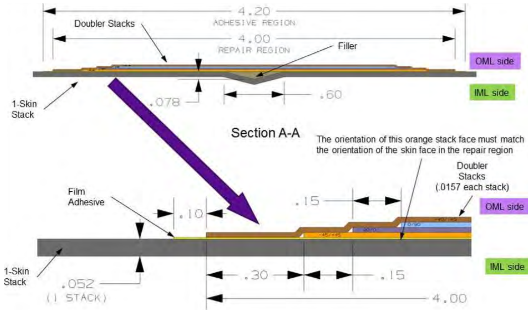
Figure B-6. Pre-cured Patch Overlap and Edge Taper Dimensions
