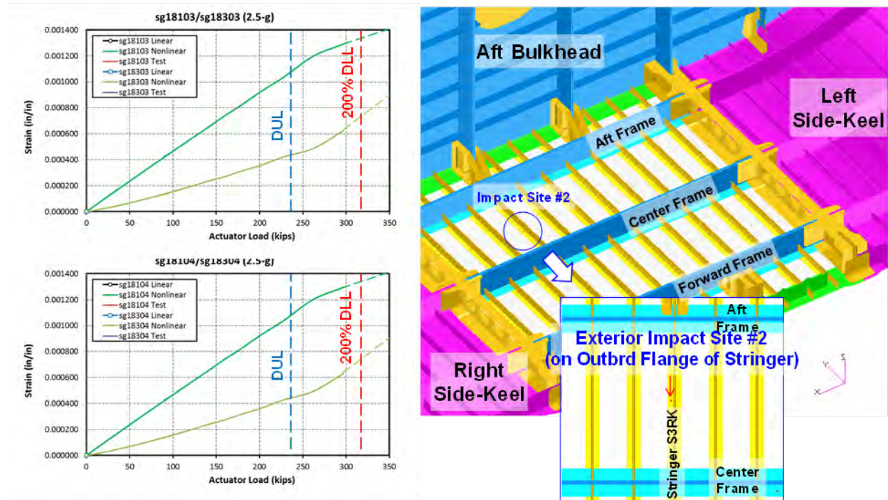
Figure 4-193. Strains on Exterior Impact Site no. 2 in 5.0-g Condition
