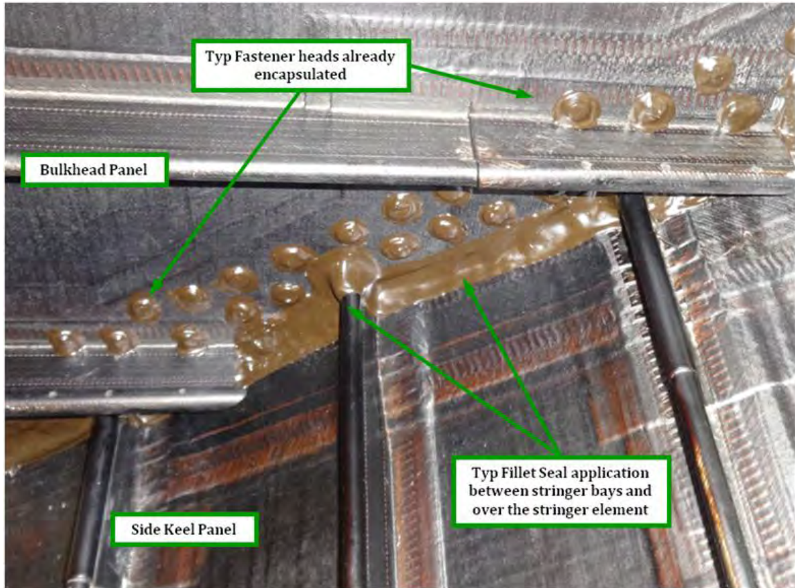
Figure 6-57. Typical Panel-to-Panel Edge Sealing
