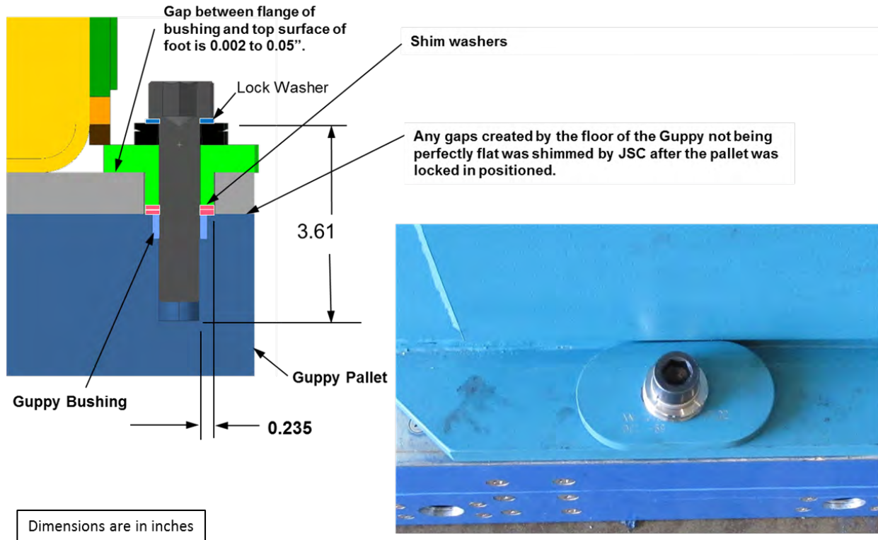
Figure 6-118. Z-Axis Restraints
