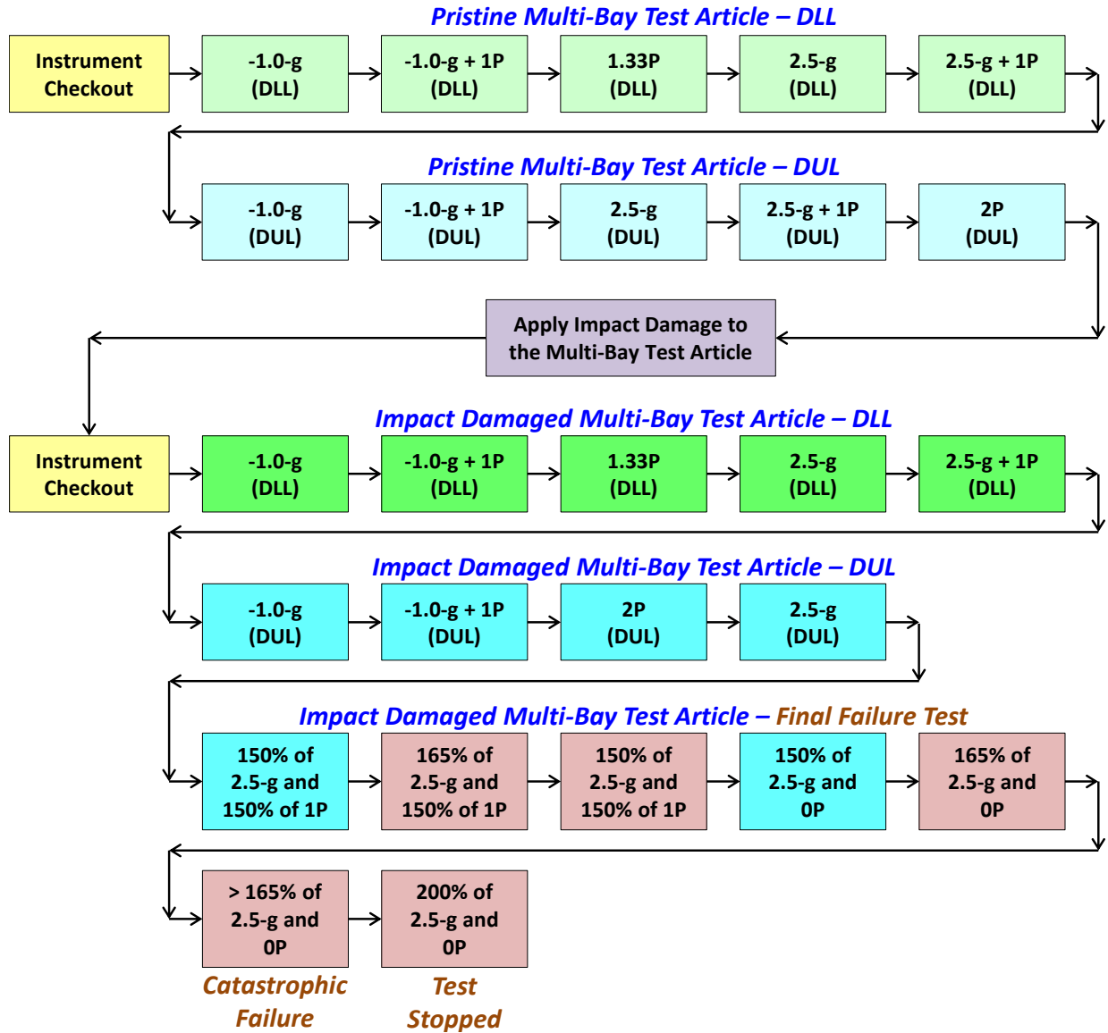
Figure 7-27. Sequence of the MBB Structural Tests
