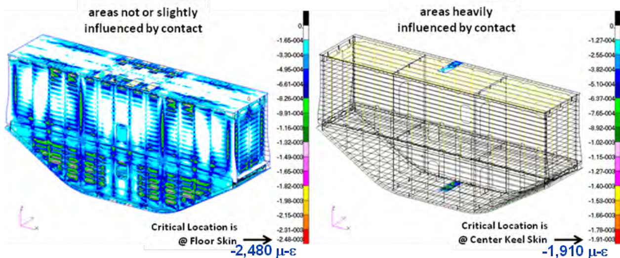
Figure 4-40. Minimum Principal Strains on Composite Skins in -1.0-g + 1P Condition
