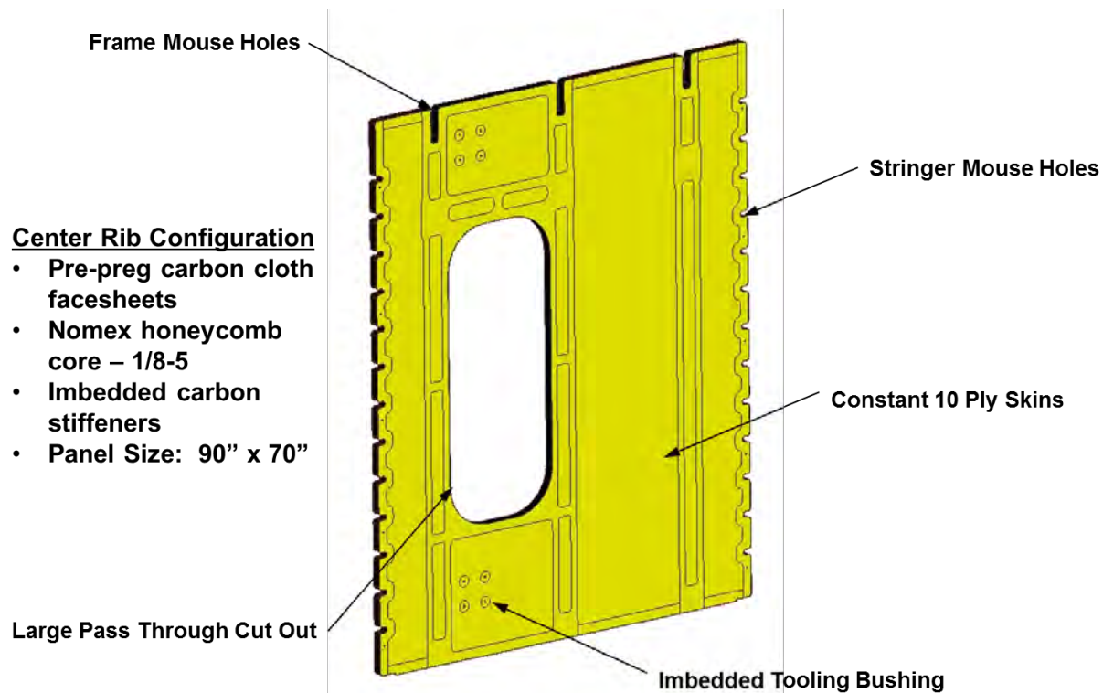
Figure 3-53. Upper Center Rib Panel Assembly
