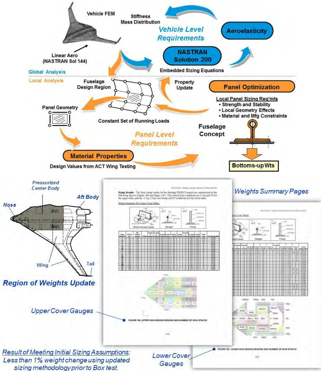
Figure 2-11. Summary of FEM-based Trade Study Structural Weights
