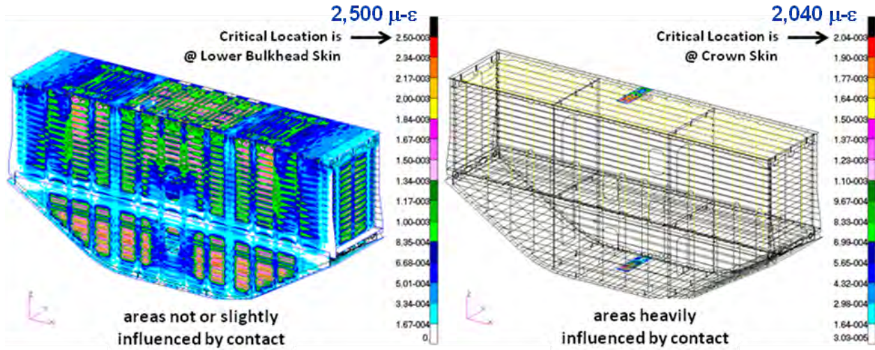
Figure 4-39. Maximum Principal Strains on Composite Skins in -1.0-g + 1P Condition
