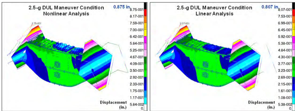
Figure 4-121. Displacements of the MBB From Linear and Nonlinear Analyses in 2.5-g DUL Condition
