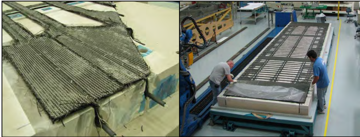
Figure 6-12. Rod and Fillet Installation (left) and Skin Layup Under Progress (right)
