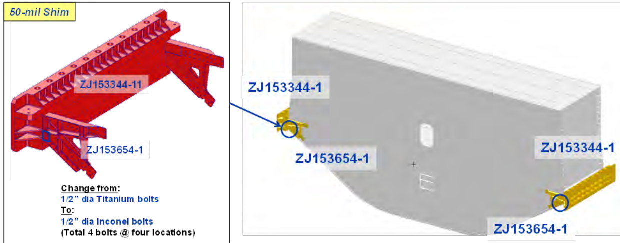
Figure 4-66. Fastener Change on ZJ153344-1 and ZJ153654-1 From the Fastener Bending Calculation
