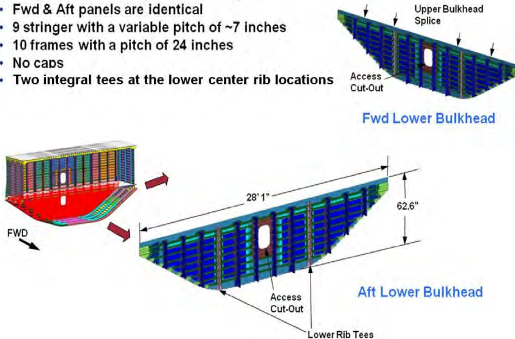
Figure 3-28. Lower Bulkhead Panel Assembly
