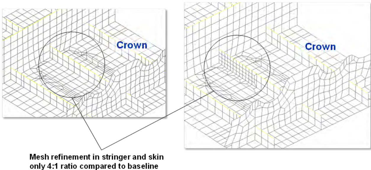
Figure 4-74. Comparison of Coarse-FEM to Fine-Mesh FEM With Refined Stringer Meshing
