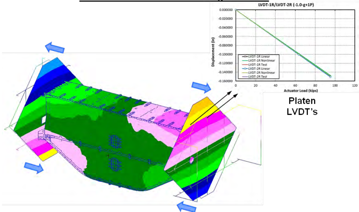
Figure 4-162. LVDT Measurements of the MBB in -1.0-g + 1P DUL Condition
