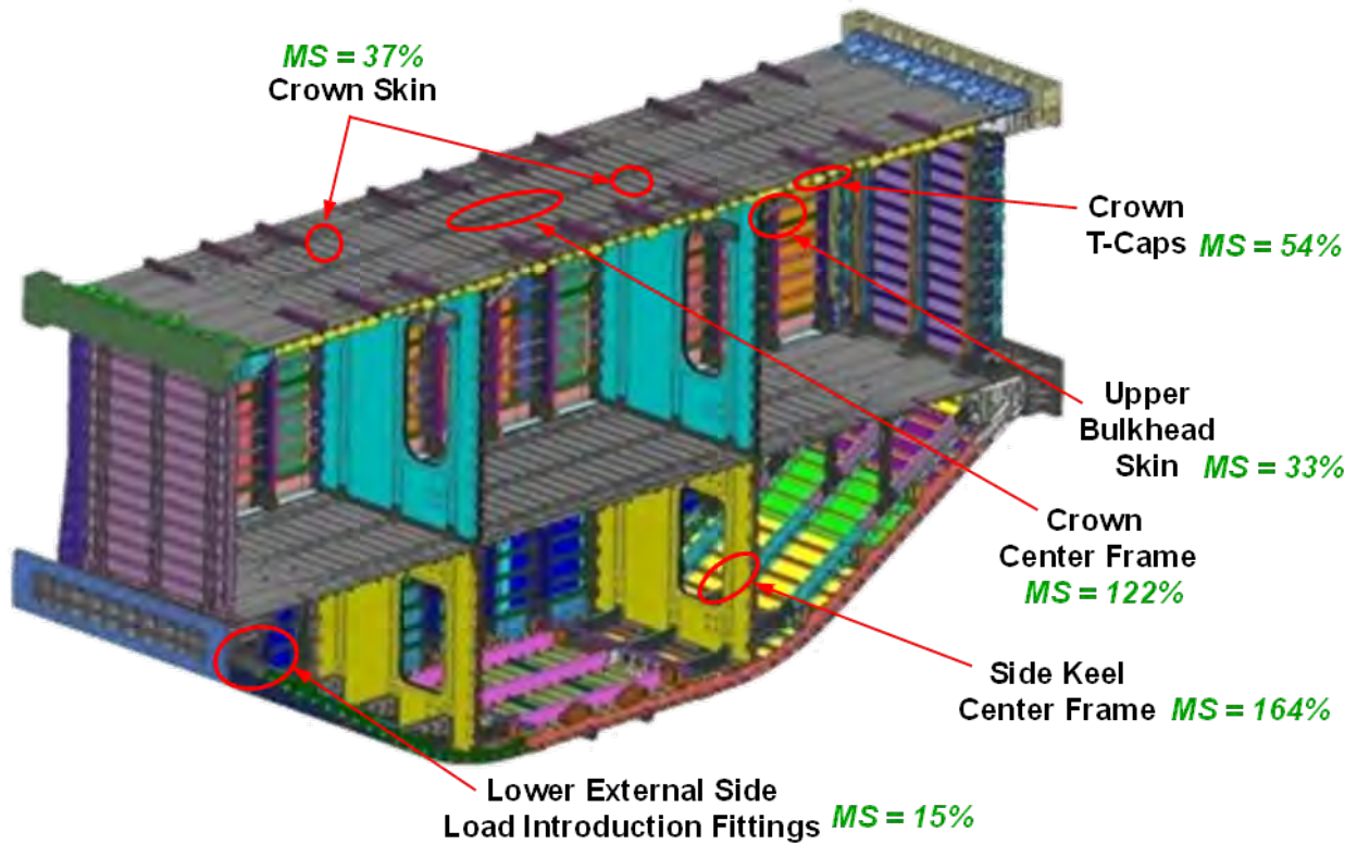
Figure 4-125. Critical Locations in Failure Predictions for the MBB in 2.5-g DUL Condition
