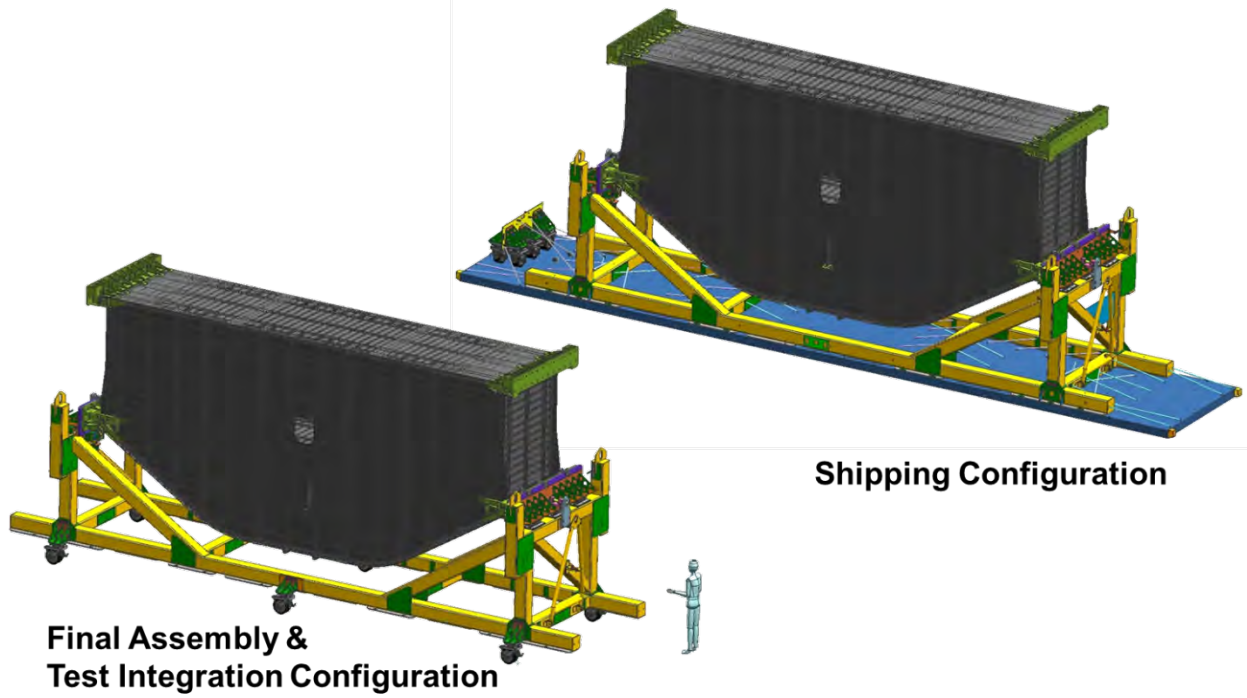
Figure 6-86. Holding Fixture Tool for the MBB
