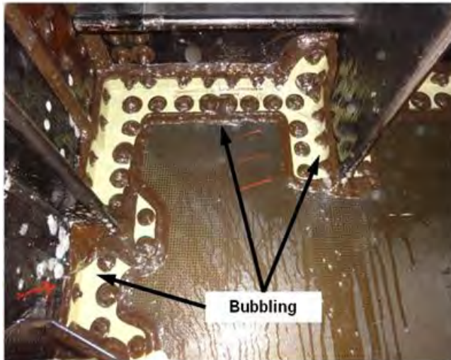
Upper Center Rib with leaks
