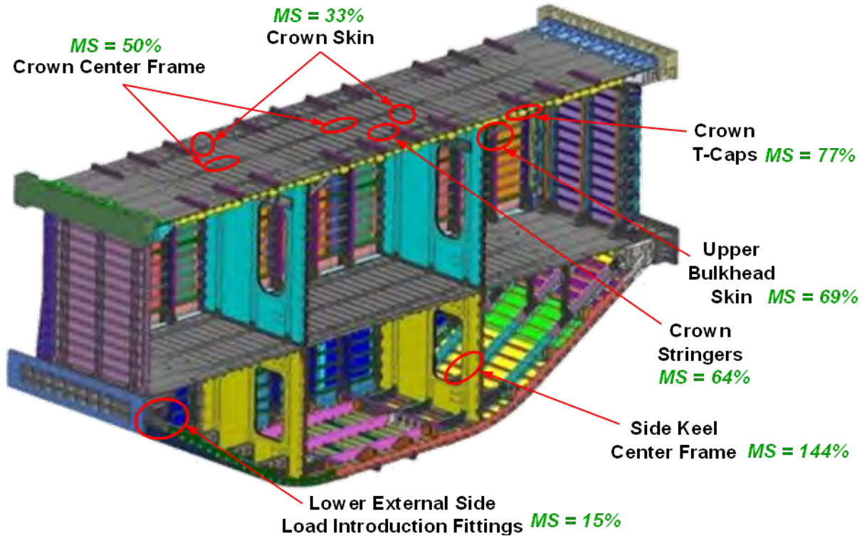
Figure 4-138. Critical Locations in Failure Predictions for the MBB in 2.5-g + 1P DUL Condition
