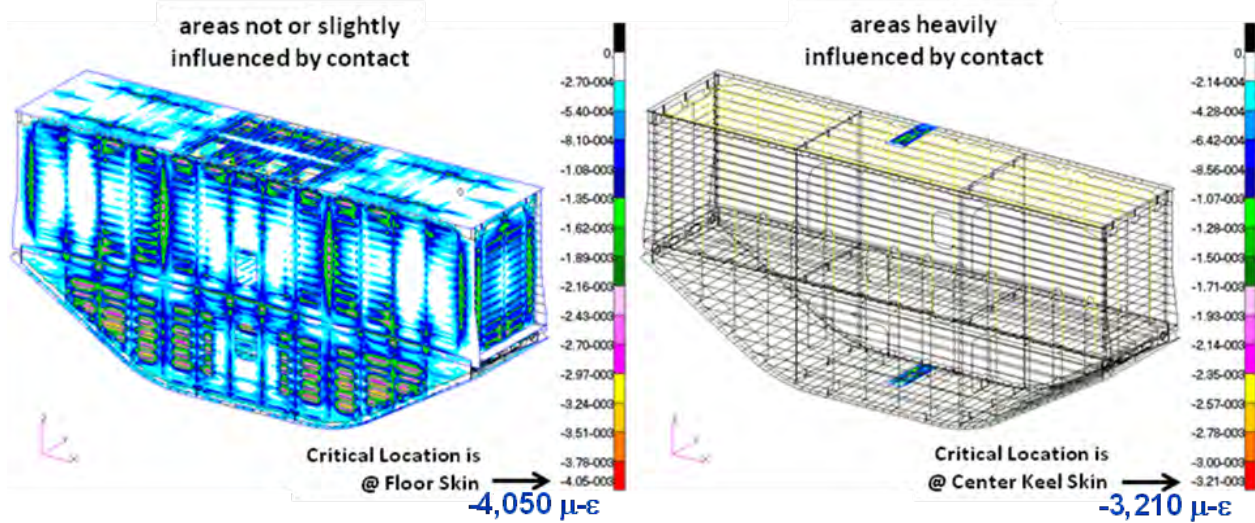
Figure 4-16. Minimum Principal Strains on Composite Skins in 2P Condition
