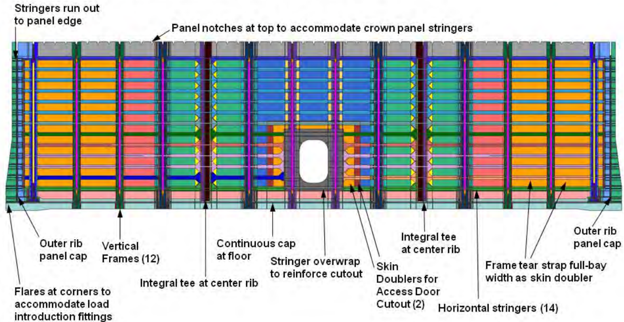
Figure 3-21. Upper Bulkhead Panel Features
