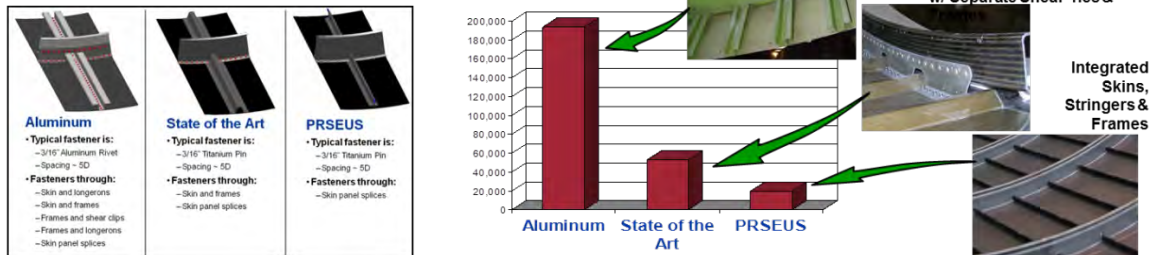
Figure 3-59. Required Number of Fasteners for Different Structural Concepts
