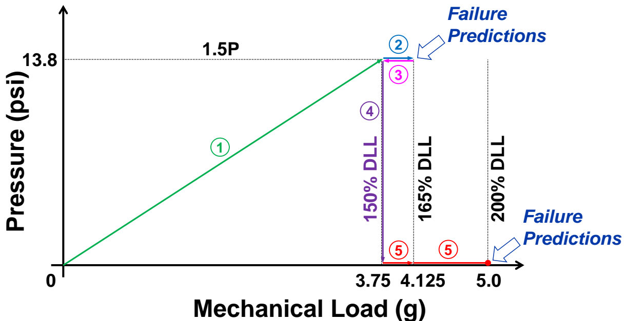
Figure 4-171. Loading Sequence Chart of Final Failure Testing
