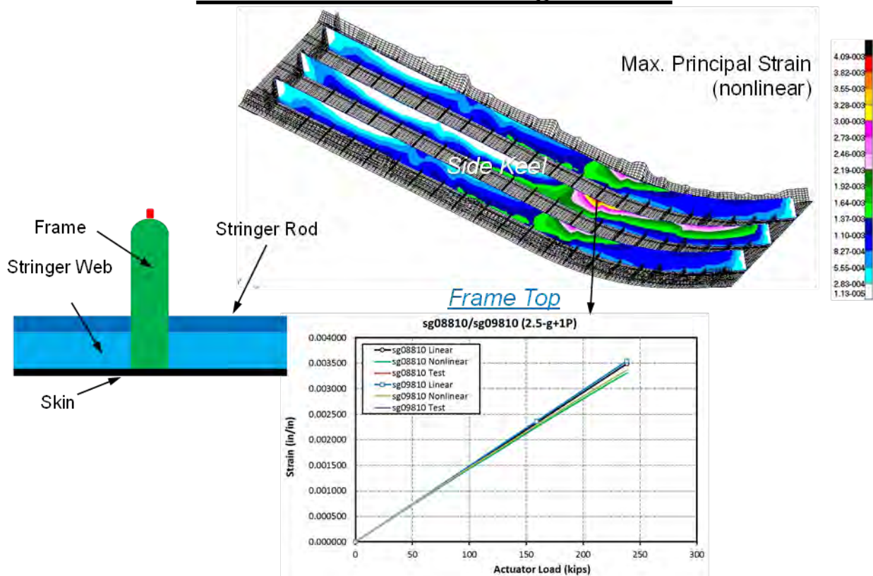
Figure 4-144. Strains on Side Keel Frames in 2.5-g + 1P DUL Condition
