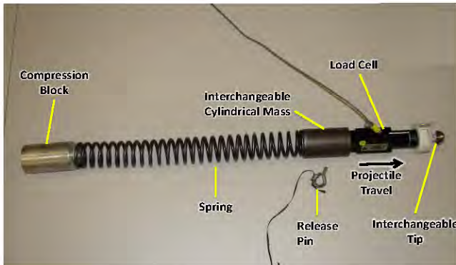
Figure 7-25. NASA Spring-Loaded Impactor
