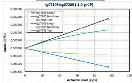
Figure 4-165. Strains on Center Keel Frames in -1.0-g + 1P DUL Condition
