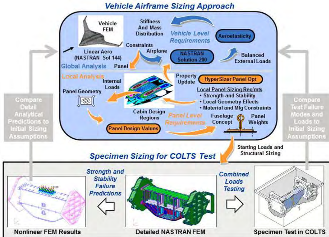
Figure 2-12. MBB Loads/Gages Were Derived from Vehicle-Level Sizing Results
