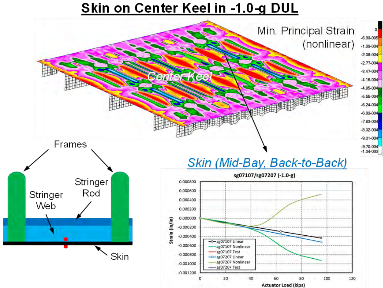
Figure 4-156. Strain on Center Keel Skin in -1.0-g DUL Condition
