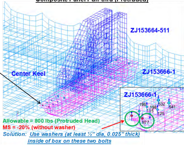
Figure 4-56. Composite Panel Pull-Through Failure Results on the Center Keel
