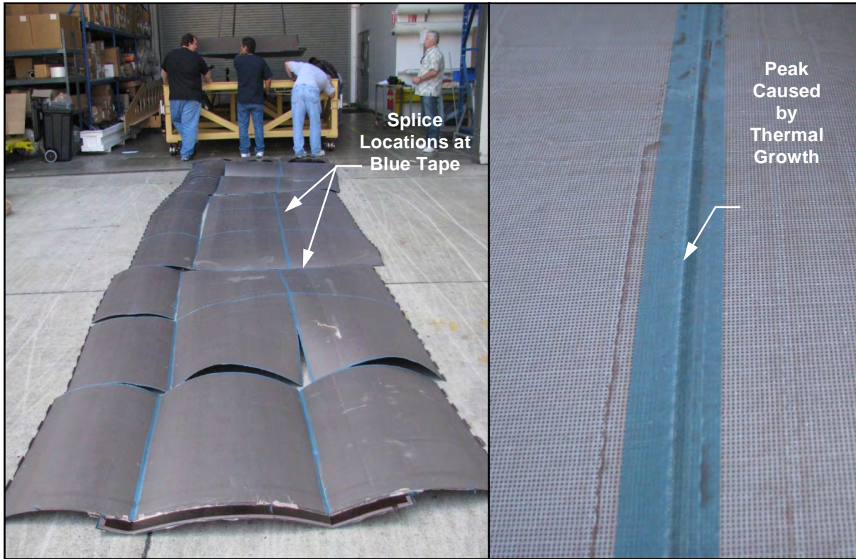
Figure 6-27. Deformation of Steel Perforated Plates at Butt Joints due to Thermal Expansion
