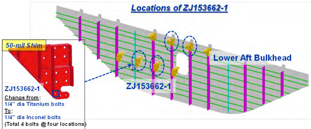
Figure 4-60. Fastener Change on ZJ153662-1 From the Fastener Bending Calculation
