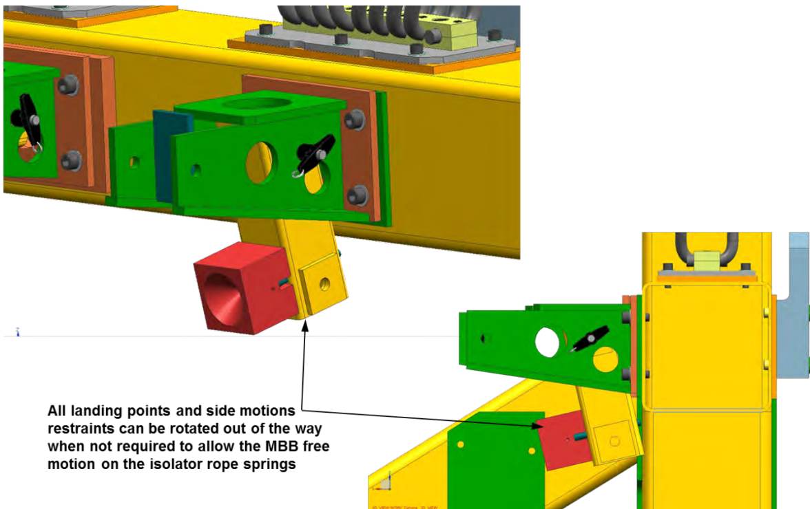
Figure 6-95. Interface Handing Fixture Swing-Down to Allow the MBB to "Float" on the Isolators
