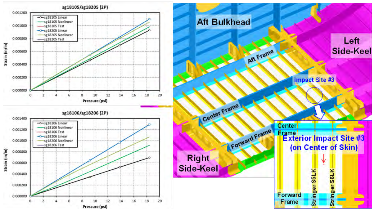
Figure 4-118. Strains on Exterior Impact Site no. 3 in 2P Condition
