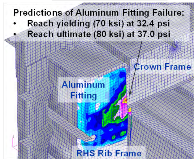
Figure 4-93. Pressure Cube Fitting Post-Failure Photograph and Predictions
