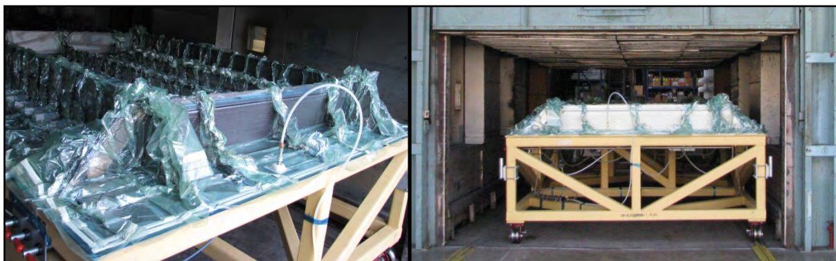
Figure 6-20. Resin-Infusion Processing of Crown Panel Inside Oven
