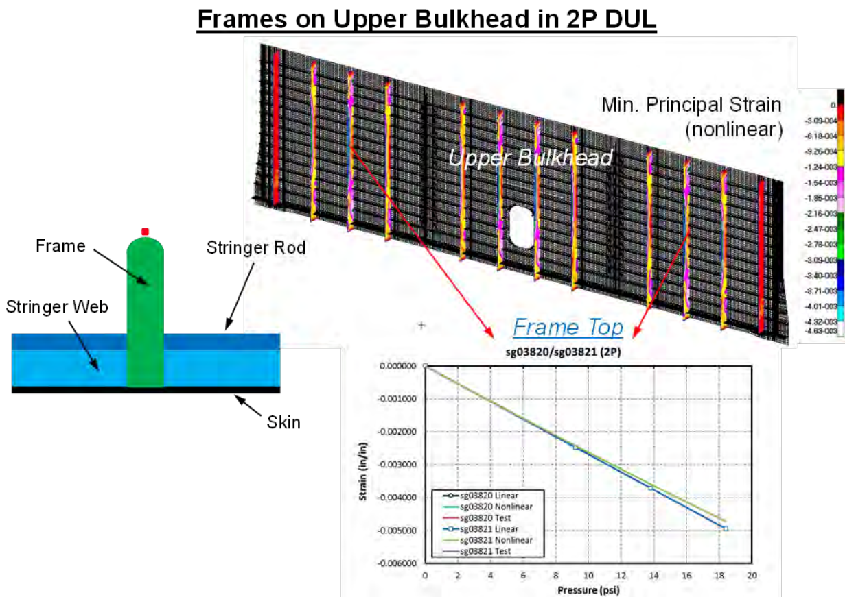
Figure 4-113. Strains on Upper Bulkhead Frames in 2P Condition
