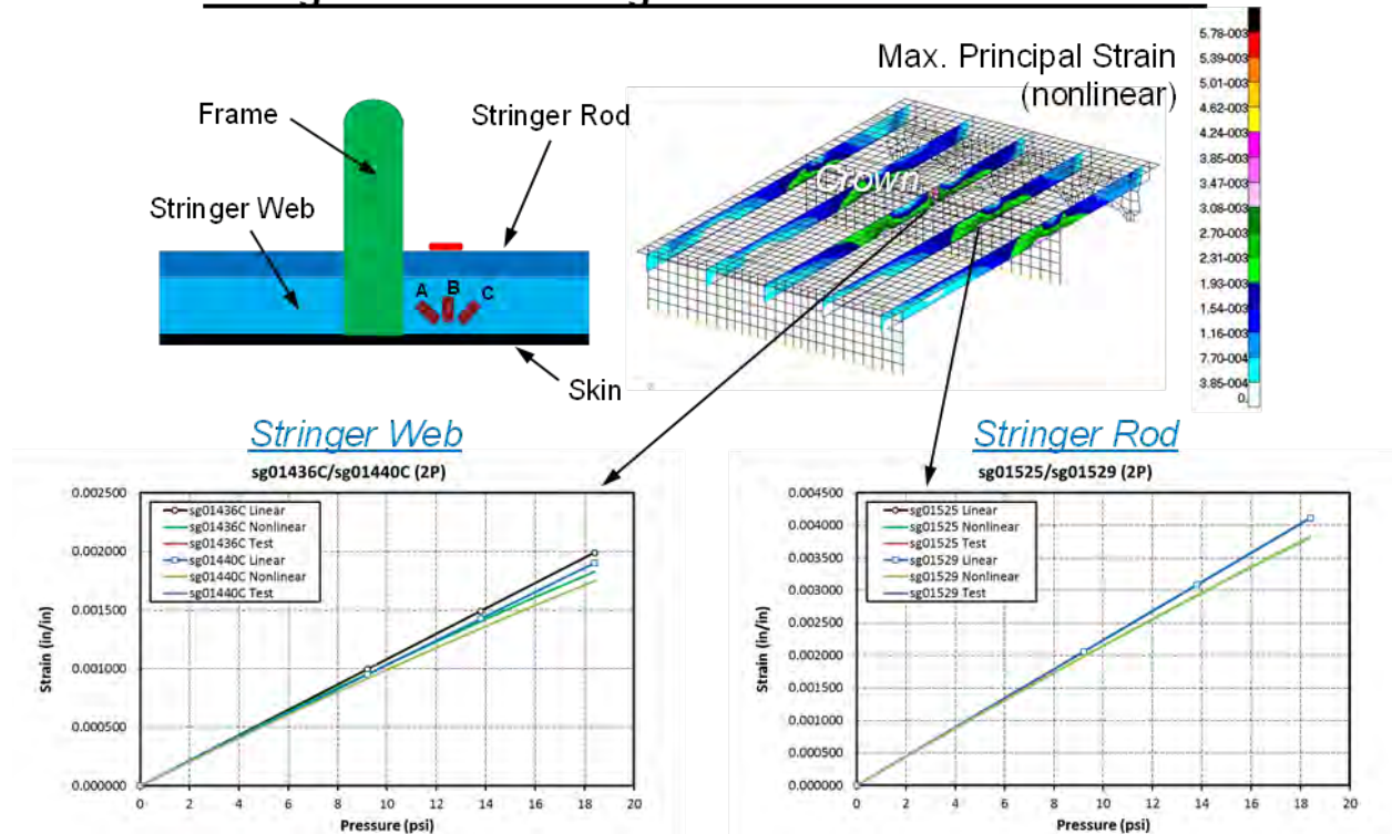
Figure 4-111. Strains on Crown Stringer Webs and Stringer Rods in 2P Condition
