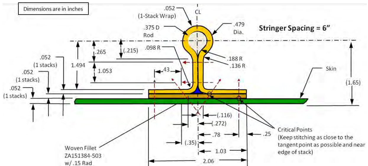
Figure 3-4. Stringer Dimensions
