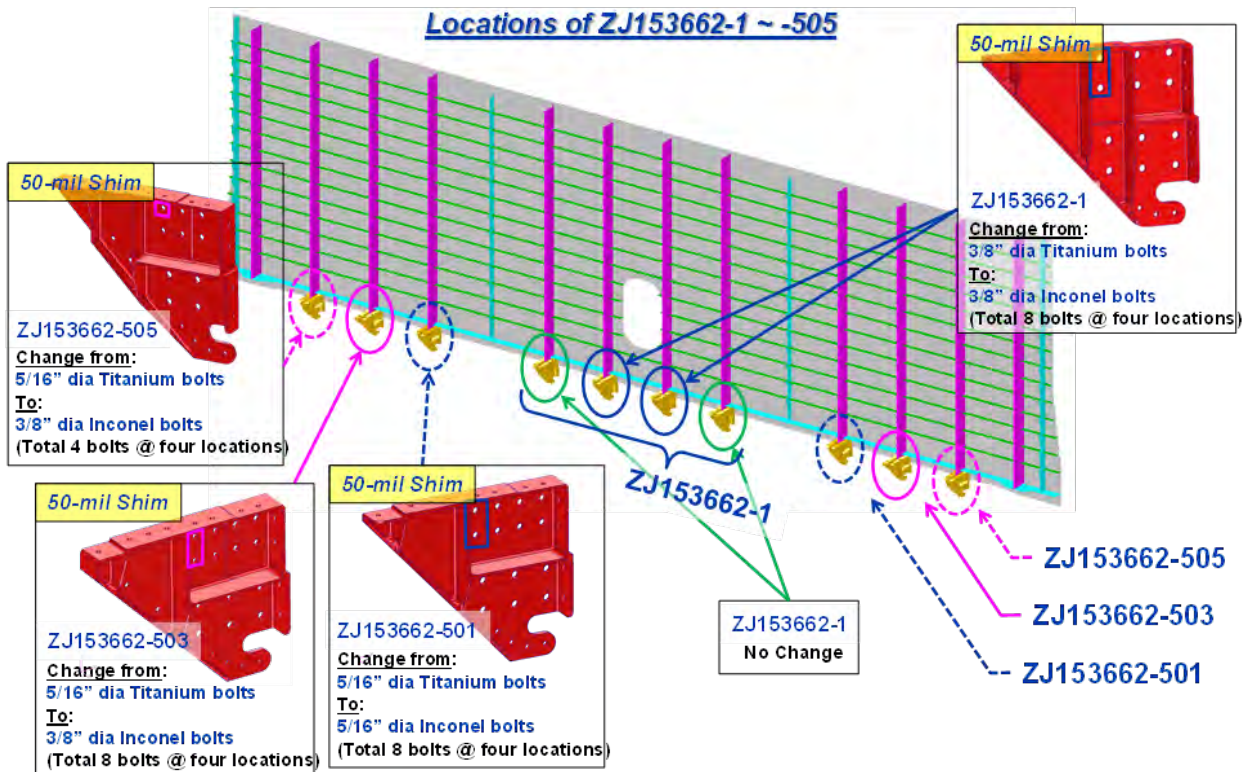
Figure 4-61. Fastener Changes on ZJ153662-1 to -505 From the Fastener Bending Calculation
