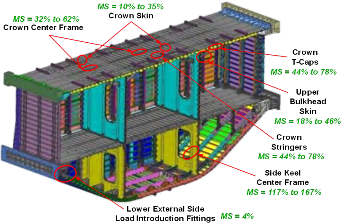
Figure 4-174. Critical Locations in Failure Predictions for the MBB in 4.125-g + 1.5P Condition
