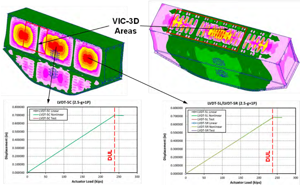
Figure 4-172. VIC-3D and LVDT Measurements of the MBB in 4.125-g + 1.5P Condition
