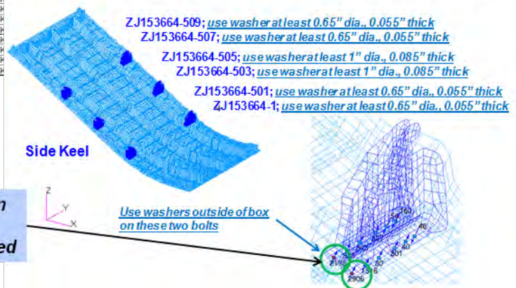
Figure 4-57. Composite Panel Pull-Through Failure Results on the Side Keels
