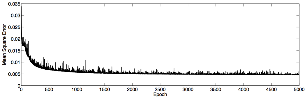
Figure 3. Mean square error in the training phase
