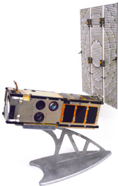
The engineering qualification model of the ISARA spacecraft showing the 3 CUMULOS cameras.
