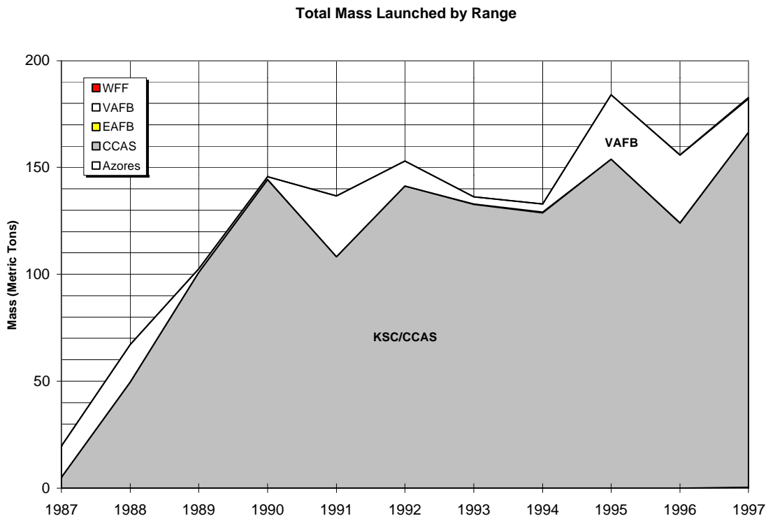
FIGURE 1—U.S. Spacelift Performance By Launch Area (1987-1997)
