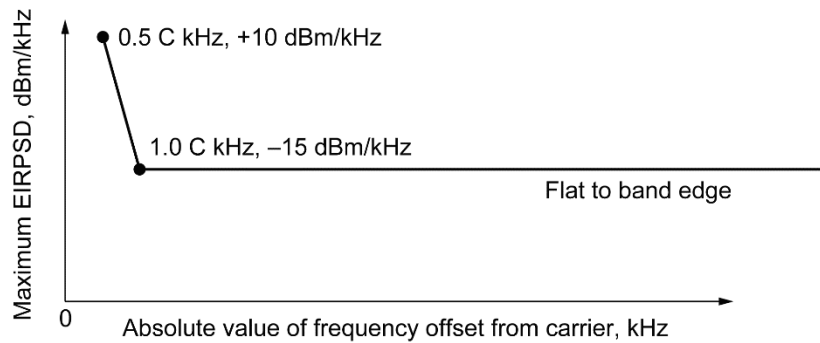
Figure 14.—C-band ground radio system transmitter effective isotropically radiated power spectral density (EIRPSD) mask.
