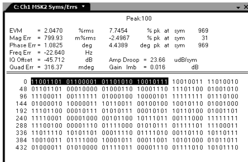
Figure 6.—Data Class 4 digital demodulation. (a) Trace A constellation diagram. (b) Trace C symbol table/error summary (RMS, root mean square). (c) Trace C symbol table/error summary (peak).
