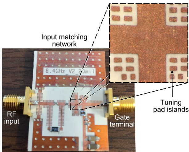
Figure 5.—Isolated input matching network with tuning pads.
