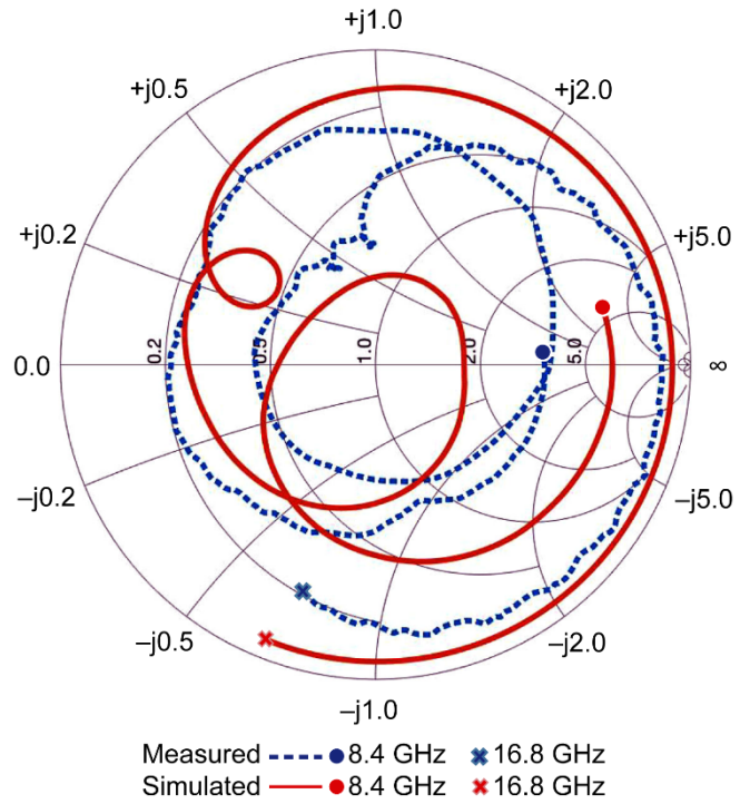
Figure 6.—Simulated and Measured ( \Gamma_{opt-in} ) parameters of input matching network after copper pad tuning from 8.4 to 16.8 GHz.
