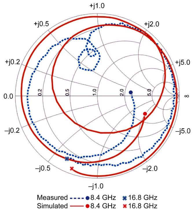
Figure 7.—Simulated and Measured ( \Gamma_{opt-out} ) parameters of output matching network after copper pad tuning from 8.4 to 16.8 GHz.
