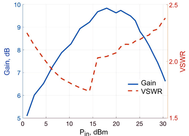
Figure 10.—Measured Gain and VSWR vs. P_{in} for inverse Class-F GaN amplifier, V_{DS} = 40 V, V_{GS} = -3.2 V, and frequency = 8.45 GHz.
