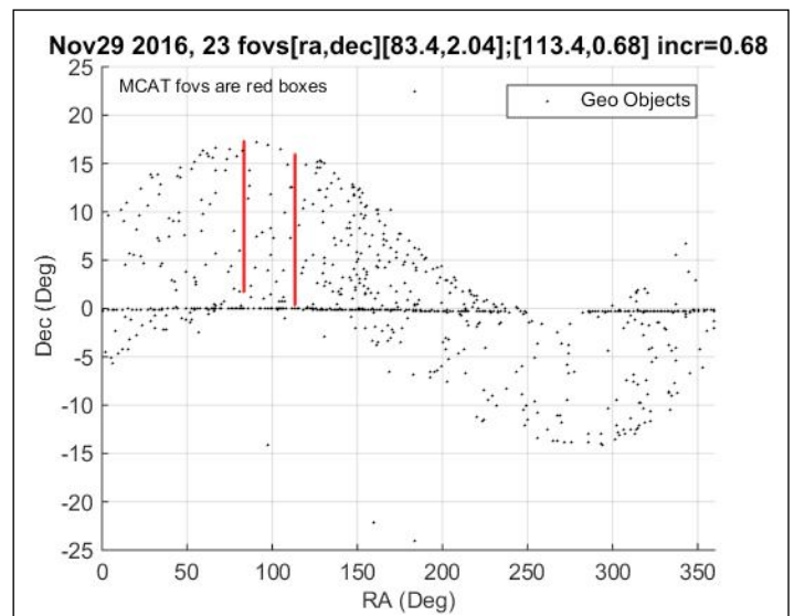
Figure 4. The distribution of catalogued GEO objects for 29 November 2016. Twenty-three FOVs are stacked (appearing as two red bars) representing the pointings in RA of the telescope on a given night, one preceding and the other following the anti-solar point. Up to 26 FOVs can be required for the regions that are wider in Dec space (e.g., RA \sim 80^\circ ).
