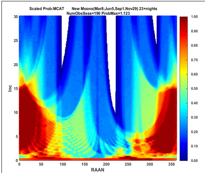
Figure 5. Four months sampled on a quarterly basis. The maximum EV here is 1.123. The white regions represent orbits that are not sampled using this method ( EV=0 ). There are also highly populated orbits that are observed with this strategy, but not fully sampled (i.e., where the EV is less than 1.0), implying this simulation scenario is not sufficient.
