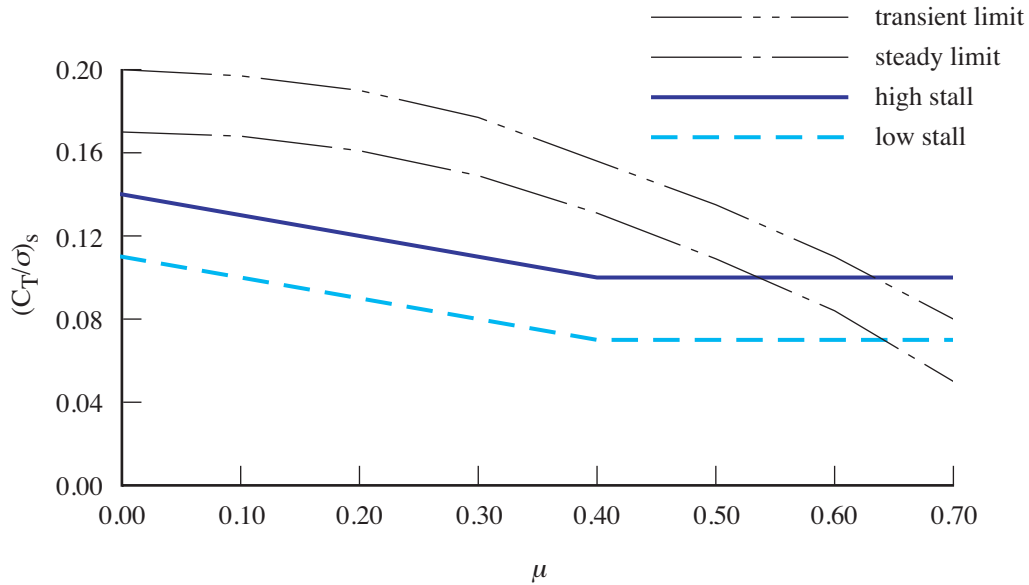
Figure 12-7. Stall function.
