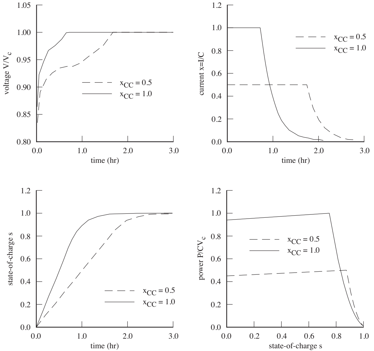
Figure 28-11. Lithium-ion battery charge characteristics.
