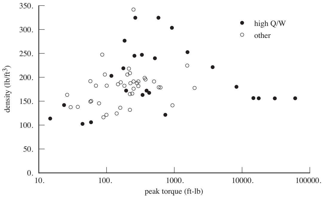
Figure 24-4. Motor density.
